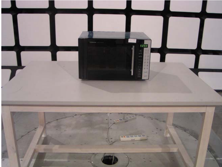
30 MHz to 1000 MHz- Radiated Emission–Front View
