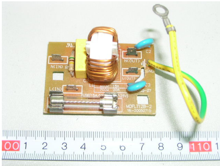
EUT – EMI Filter PCB Top View
