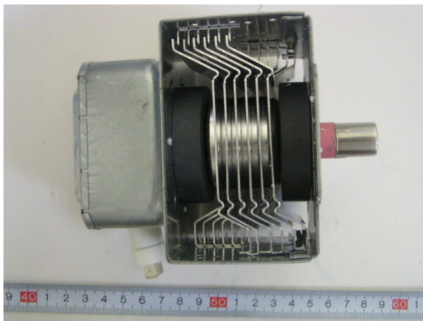
EUT- Magnetism Signal Generator Left View
