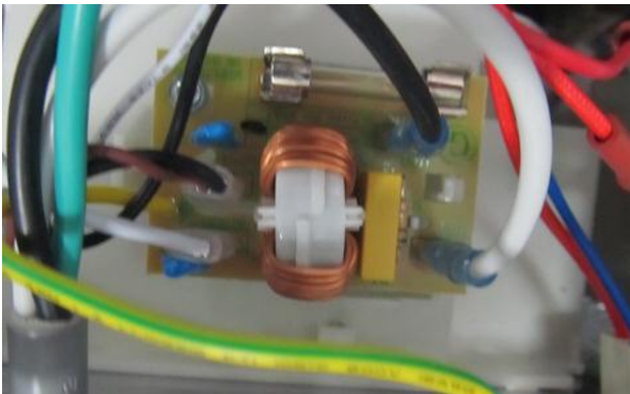
Power Filter Board Top View
