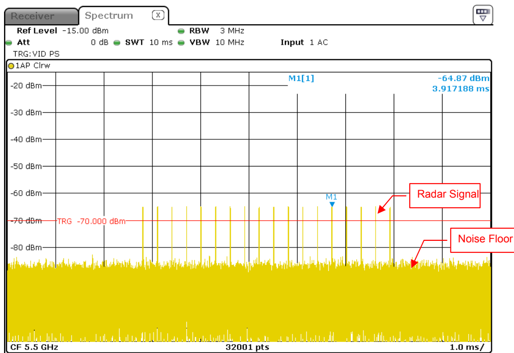
Radar Signal 3
