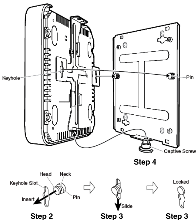
Figure 9. Attaching Access Point to Base Plate
