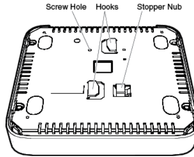
Figure 6. Bottom of Access Point
