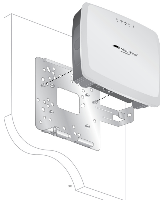
Figure 10. Aligning the Access Point with the Mounting Base Plate
