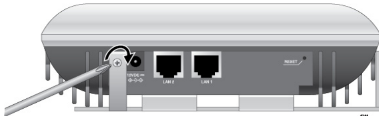
Figure 12. Fastening the Captive Screw to Secure the Access Point
