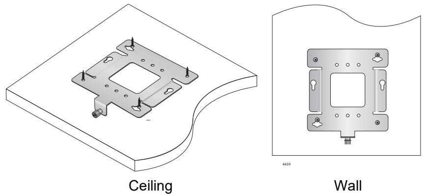
Figure 11. Stationary Bracket Position
