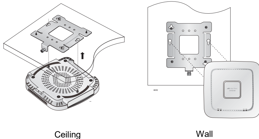
Figure 15. Align/Insert Access Point into Mounting Bracket
