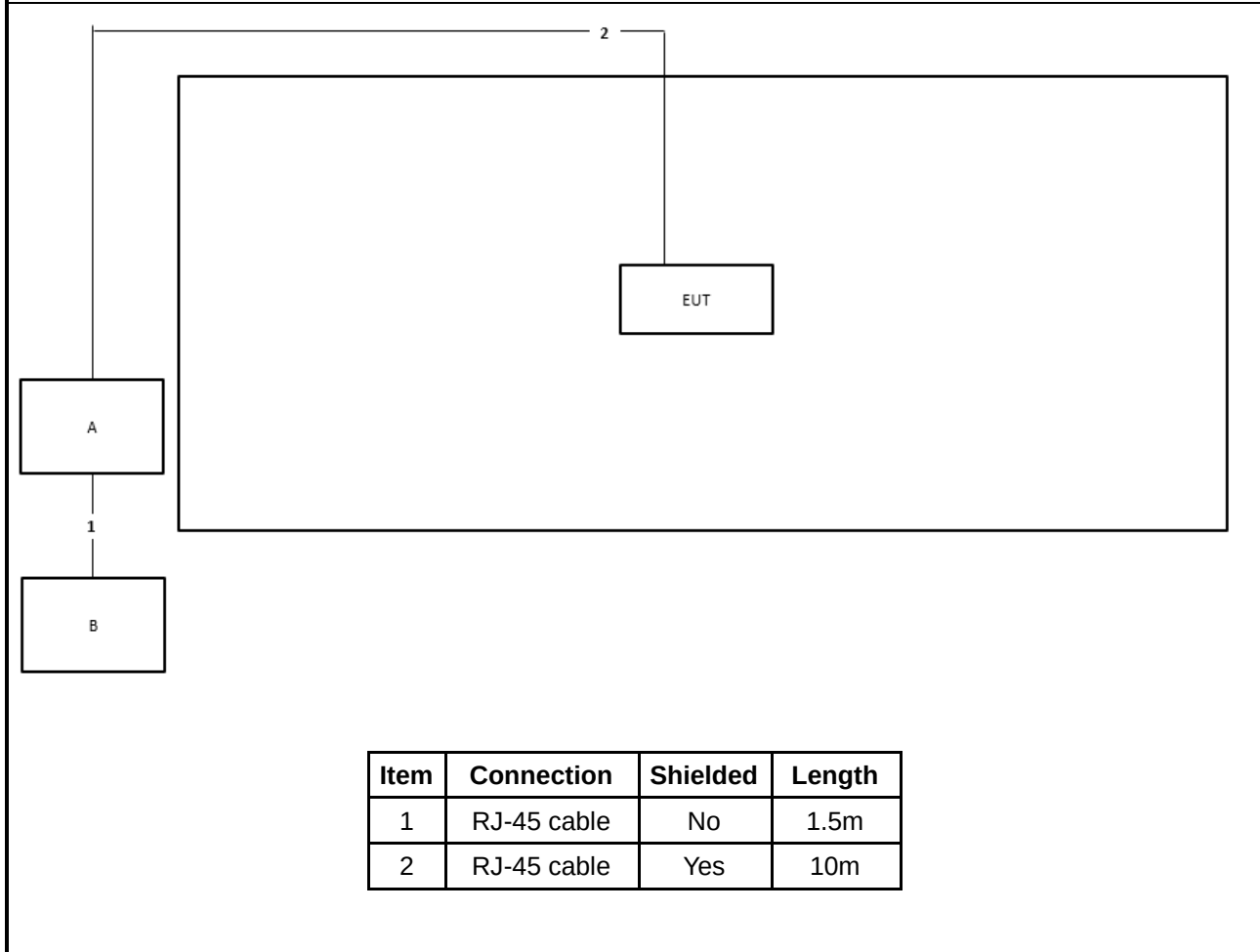
Test Setup Diagram - Radiated Test > 1GHz
