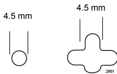
Figure 12. Hole Dimensions
