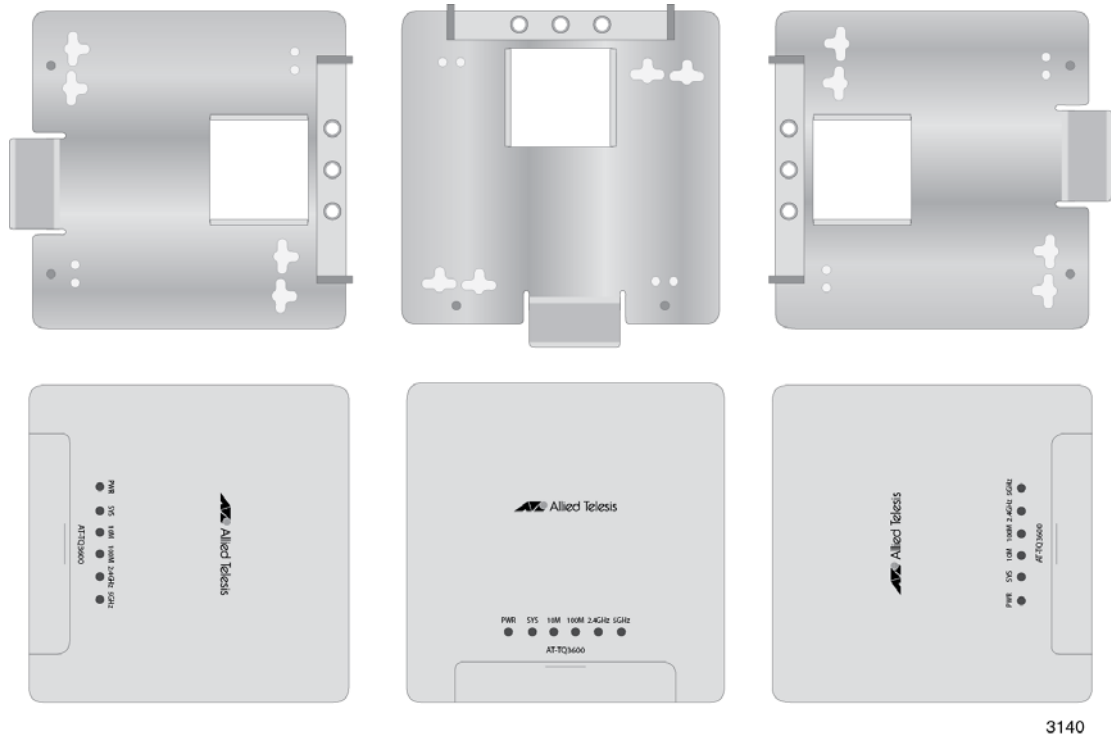
Figure 9. Wall Orientations
