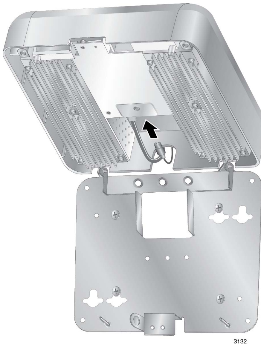
Figure 22. Connecting the DC Cable from the AT-TQ0091 Power Adapter
