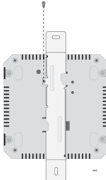
Figure 10. Attaching the Mounting-Bracket Screw
