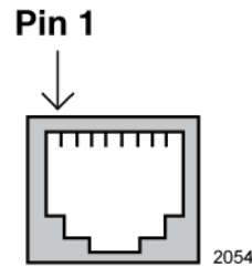
Figure 14. Pin Layout for the RJ-45 Connector on the LAN Port
