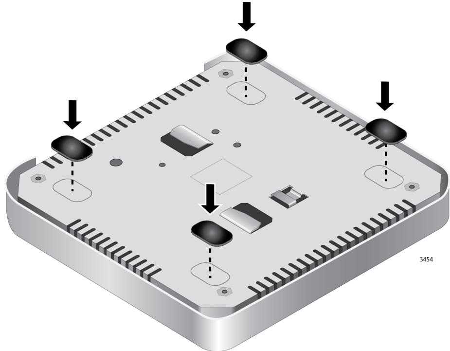
Figure 3. Installing the Rubber Feet
