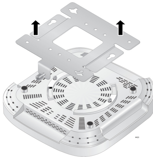
Figure 7. Removing Mounting Bracket From Access Point
