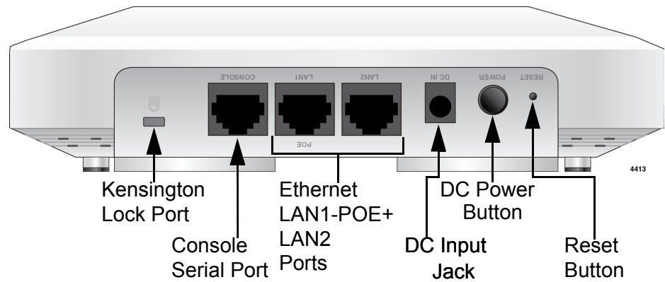
Figure 3. Back Edge View
