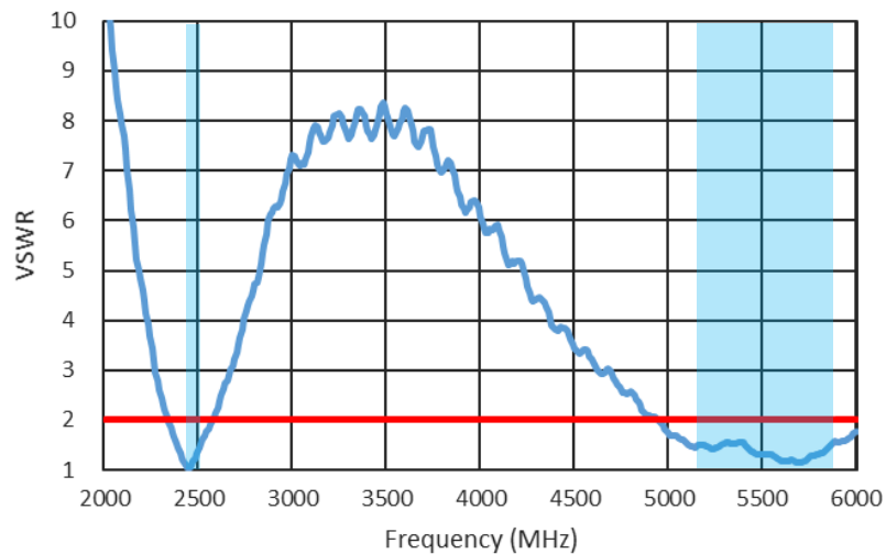
Dual2 VSWR=2
