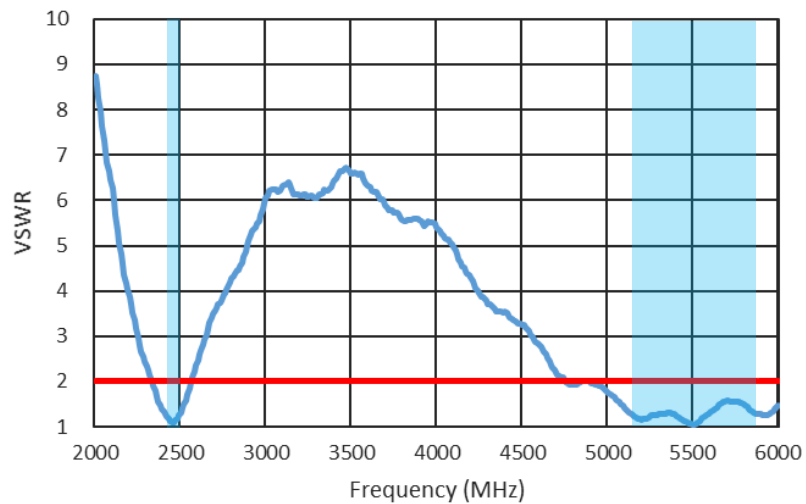
Dual3 VSWR=2
