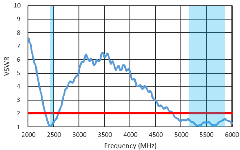
Dual4 VSWR=2
