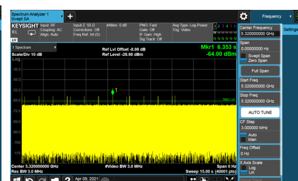
Radar Type 5 Calibration Plot
