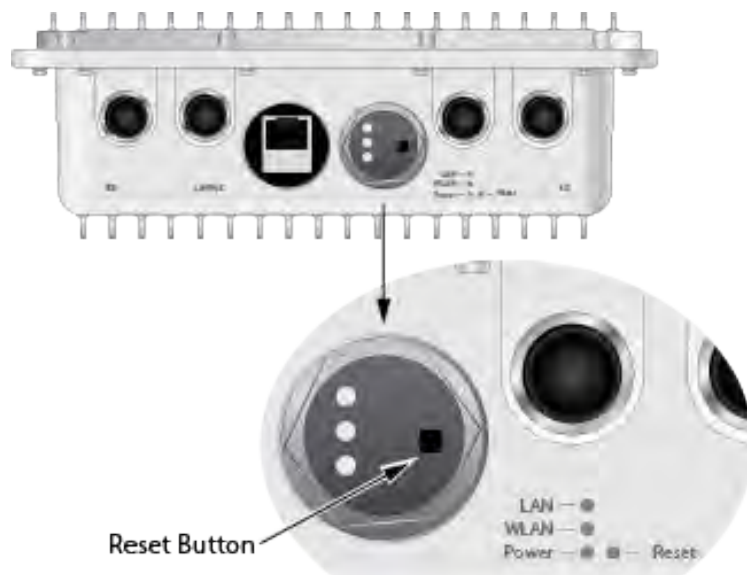
Figure 5. Reset Button
