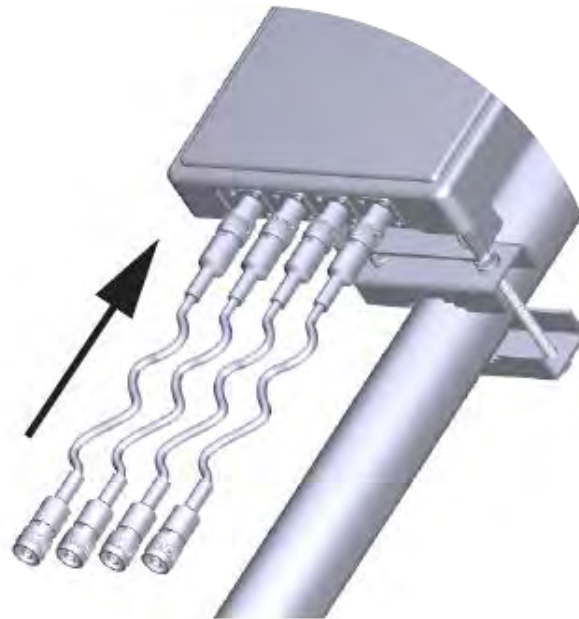
Figure 42. Attaching the Cables to the Antenna Connectors
