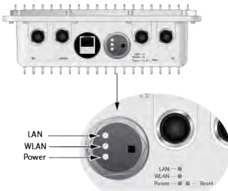
Figure 4. LEDs
