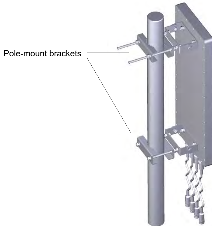
Figure 41. TQ0301 Patch Antenna on a Pole
