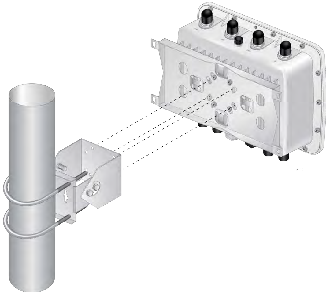
Figure 38. Attaching the Access Point to the Pole-Mount Brackets
