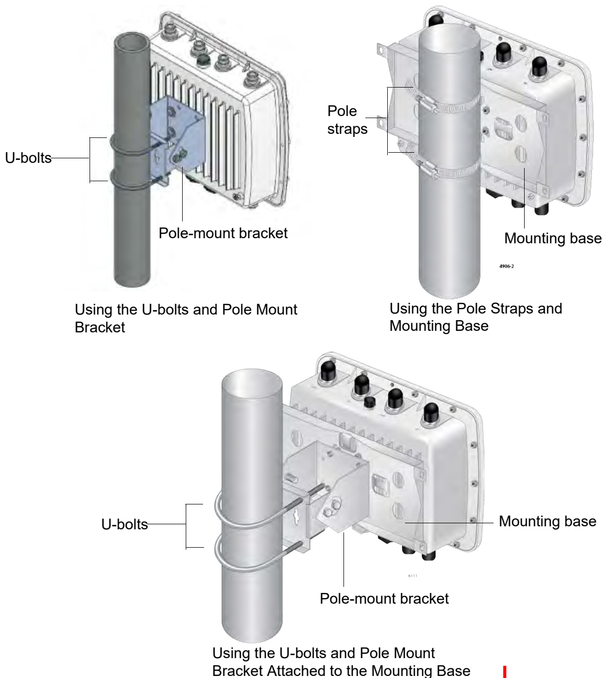
Figure 30. Three Methods of Pole Installations
