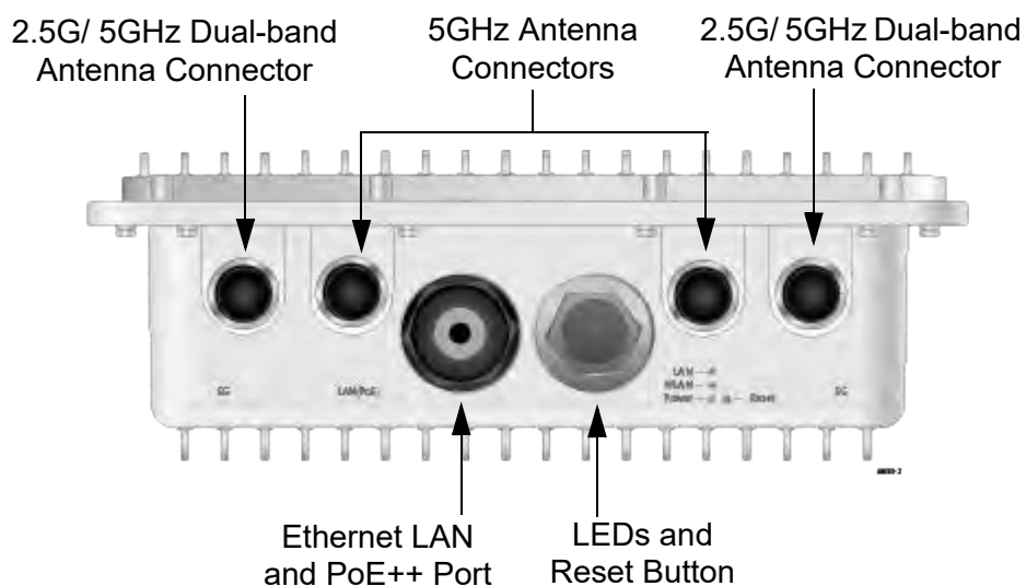
Figure 1. Front Panel of the TQ6702e GEN2 Access Point
