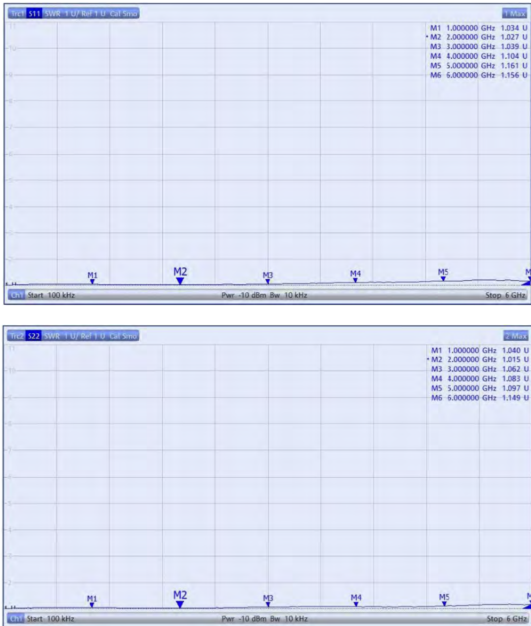
Figure 1: Model 305 Connector VSWR
