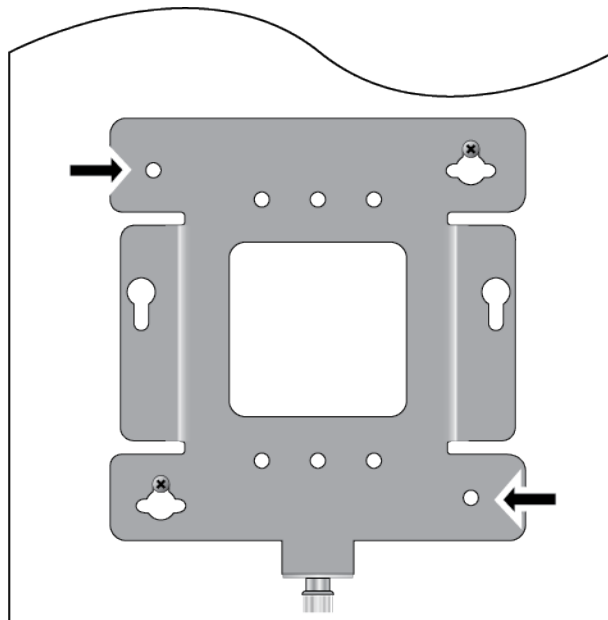
Figure 21. Pre-Drill Holes on Mounting Bracket
