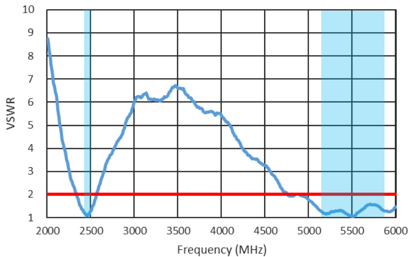
Dual3 VSWR=2
