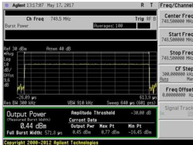
7.2_Power_DL_746-757MHz_GSM_Max
