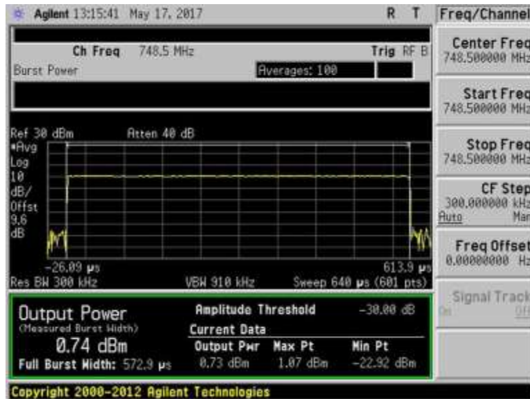
7.2_Power_DL_746-757MHz_GSM
