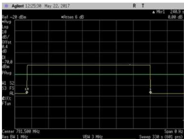
7.8_InactivityUL_776-787MHz
