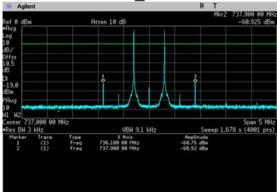
7.4_Intermod_DL_728-746MHz
