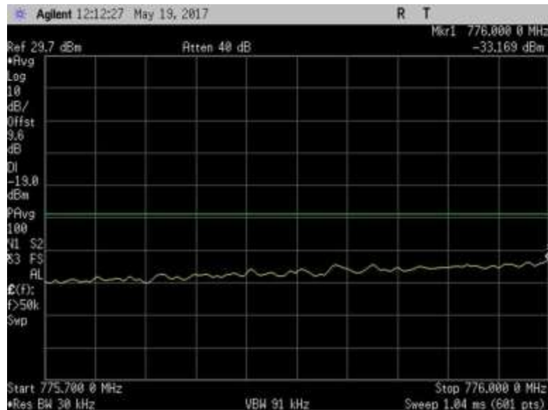
7.5_OBE_UL_776-787MHz_L_PreAGC_CDMA
