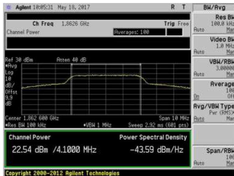
7.2_Power_UL_1850-1915MHz_AWGN_Max
