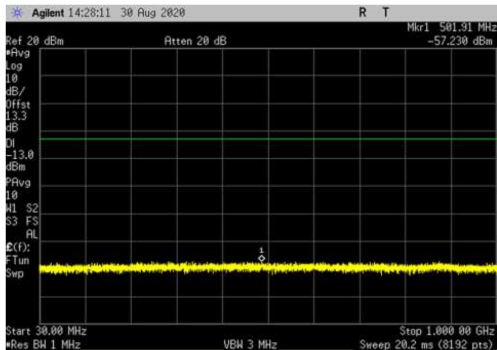
DL_H_256QAM_100MHz_RB1_CP_ 30- 1000MHz_fo
