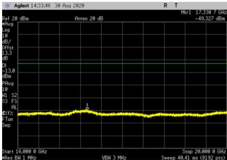
DL_H_16QAM_400MHz_Full_CP_16000-20000MHz_fo
