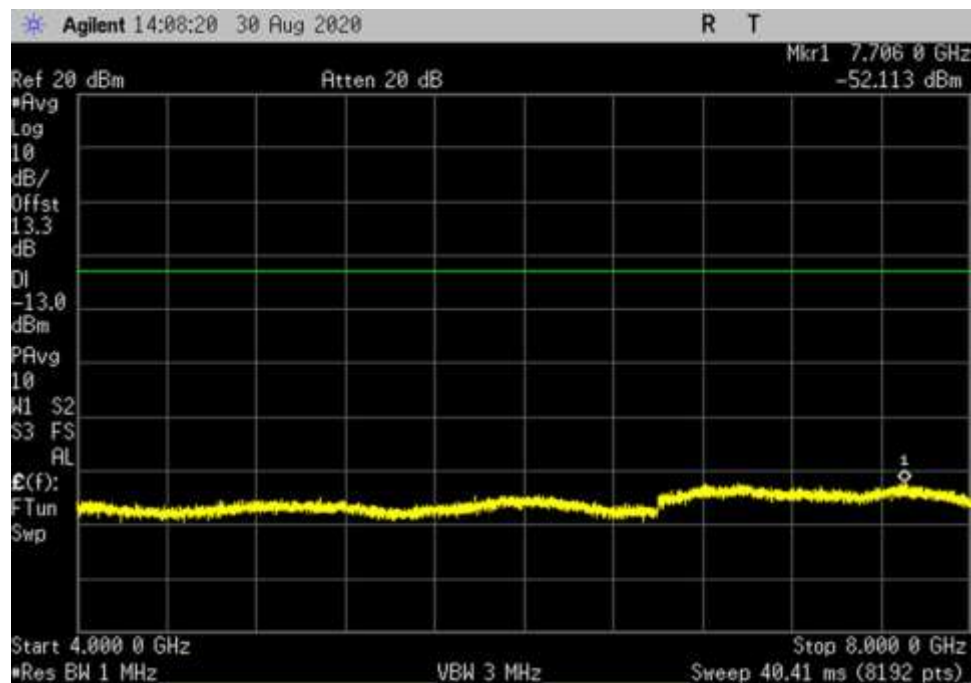
DL_H_16QAM_100MHz_Full_CP_4000- 8000MHz_fo
