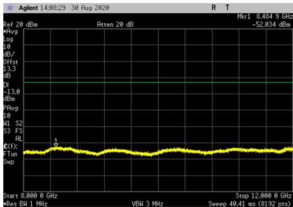
DL_H_16QAM_100MHz_Full_CP_8000- 12000MHz_fo
