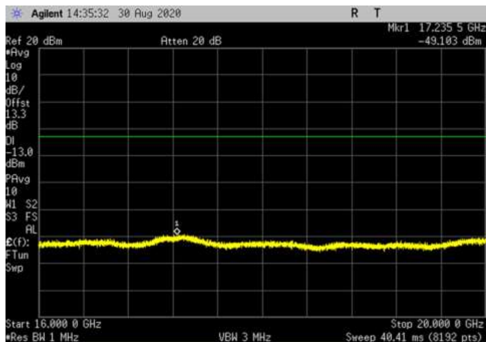
DL_H_64QAM_400MHz_Full_CP_16000- 20000MHz_fo
