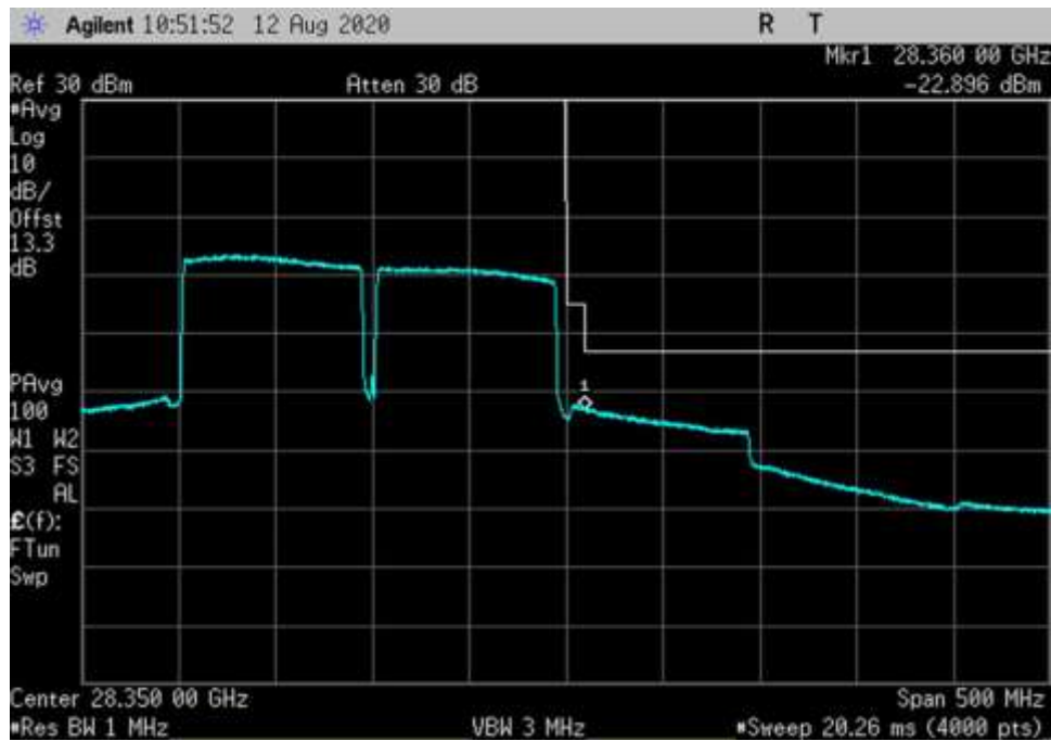
UL_27500-28350-256QAM-100MHz-H-AGC+3-DFT OFDM_HC
