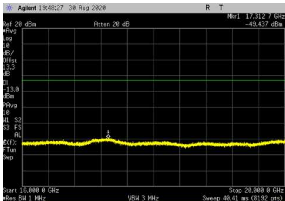
UL_V_256QAM_400MHz_Full_DFT_16000-20000MHz_fo
