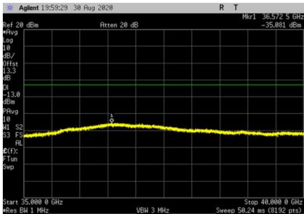
UL_V_64QAM_400MHz_RB1_DFT_35000-40000MHz_fo
