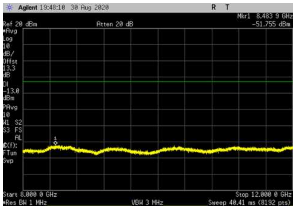
UL_V_256QAM_400MHz_Full_DFT_8000- 12000MHz_fo
