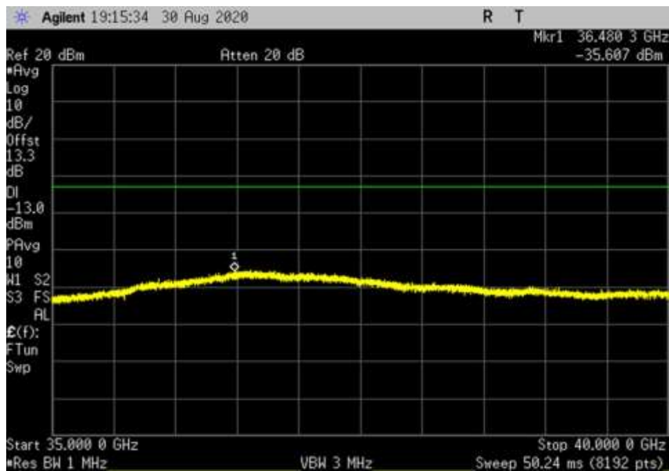
UL_V_256QAM_100MHz_Full_DFT_ 35000- 40000MHz_fo
