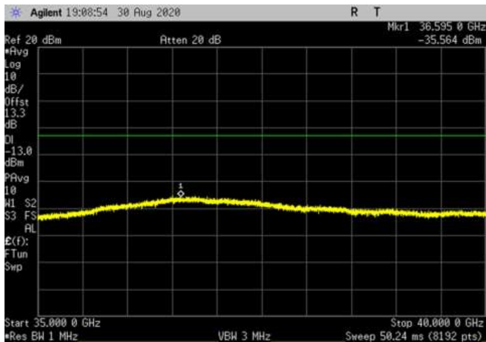
UL_V_QPSK_100MHz_Full_DFT_35000-40000MHz_fo
