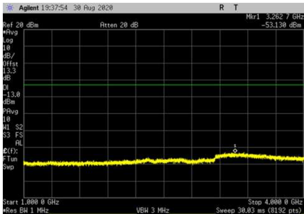
UL_V_QPSK_400MHz_Full_DFT_1000-4000MHz_fo
