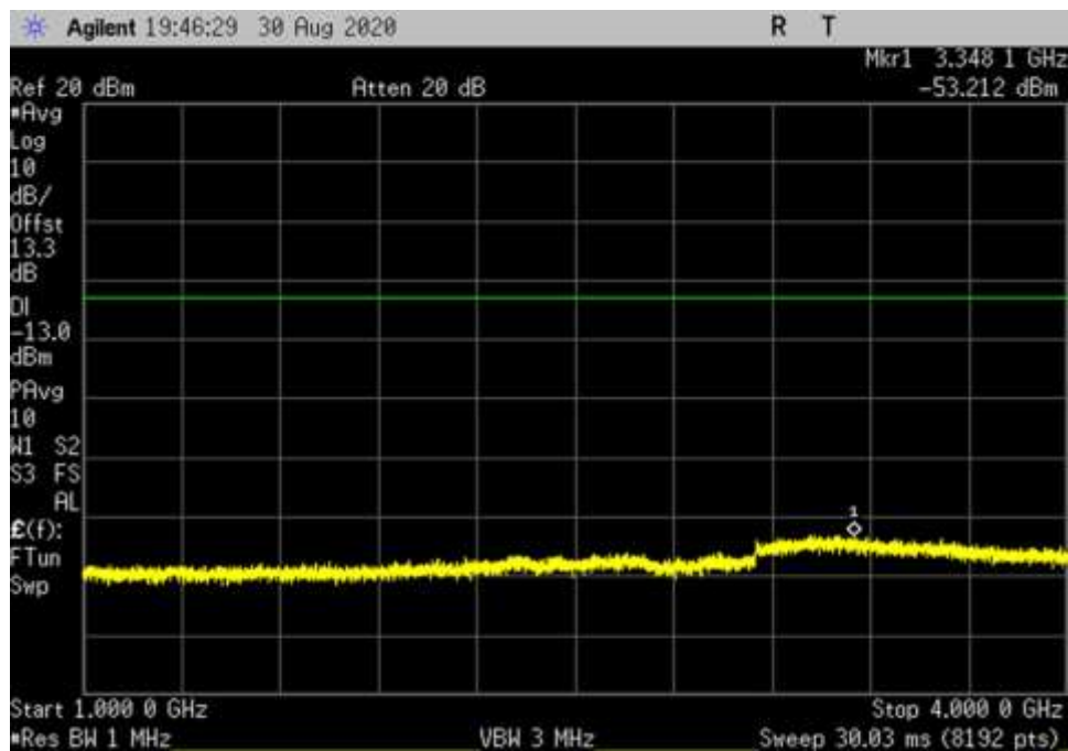
UL_V_256QAM_400MHz_Full_DFT_1000- 4000MHz_fo
