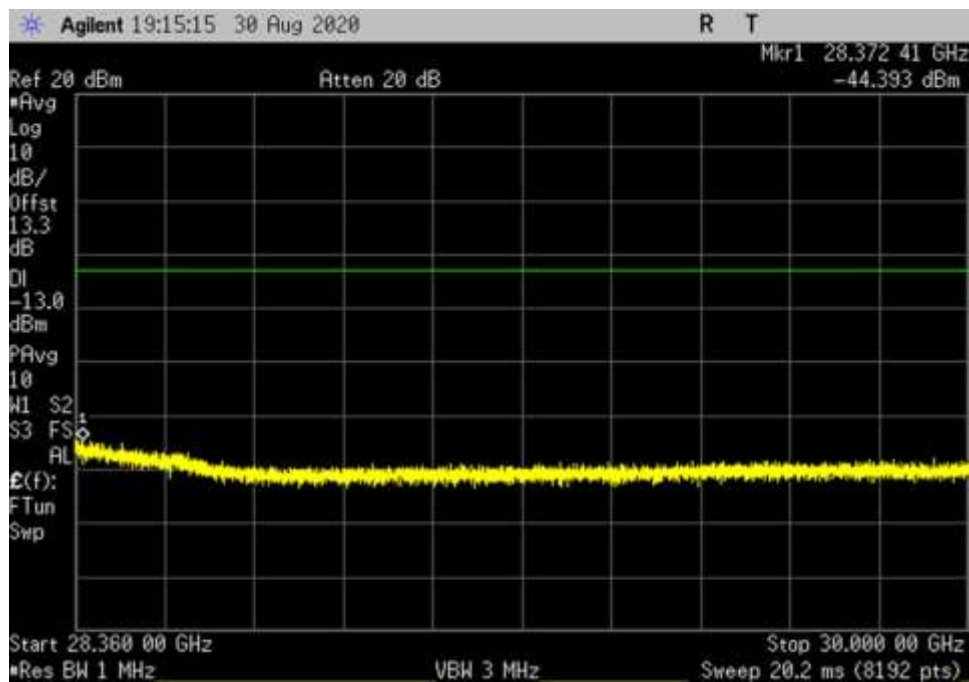
UL_V_256QAM_100MHz_Full_DFT_ 28360- 30000MHz_fo
