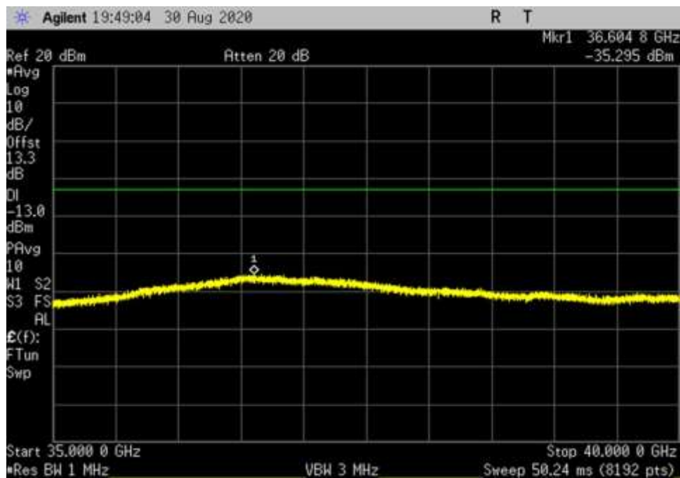
UL_V_256QAM_400MHz_Full_DFT_35000-40000MHz_fo
