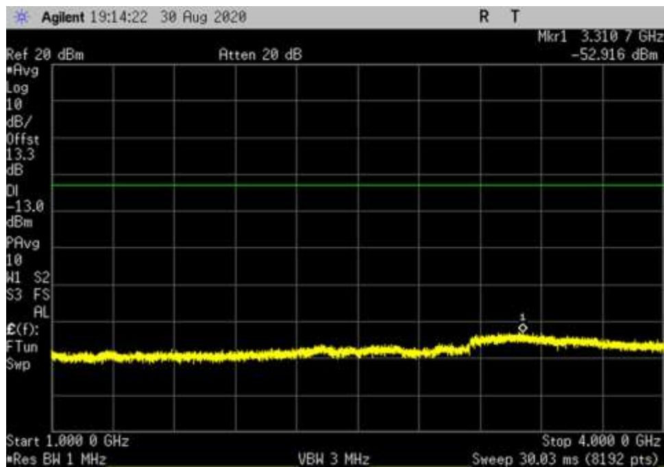
UL_V_256QAM_100MHz_Full_DFT_1000- 4000MHz_fo
