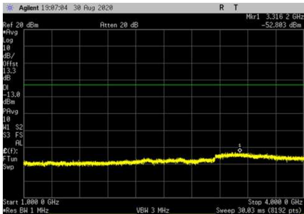
UL_V_QPSK_100MHz_Full_DFT_1000-4000MHz_fo
