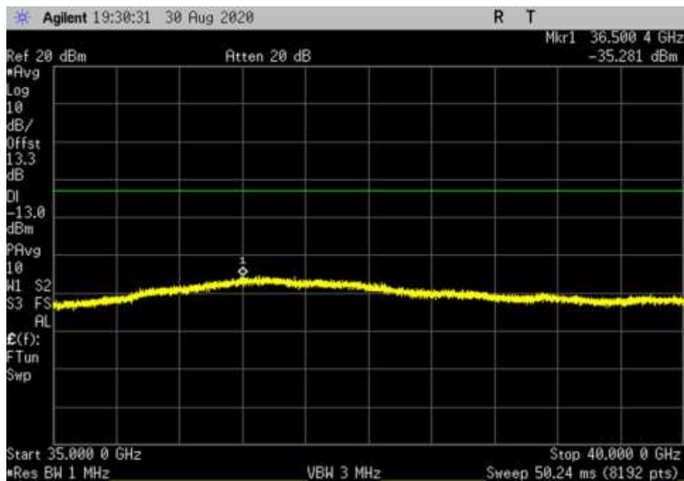
UL_V_256QAM_100MHz_RB1_DFT_35000-40000MHz_fo
