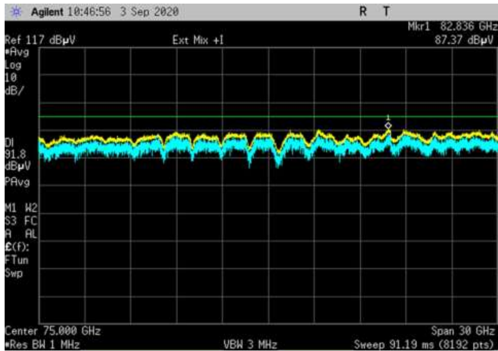
DL-Hout-64QAM-100MHz_ 60000- 90000MHz_MC-H
