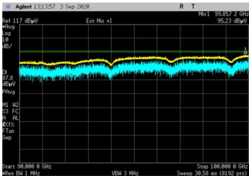
UL-Hout-QPSK-100MHz_90000-100000MHz_MC-V
