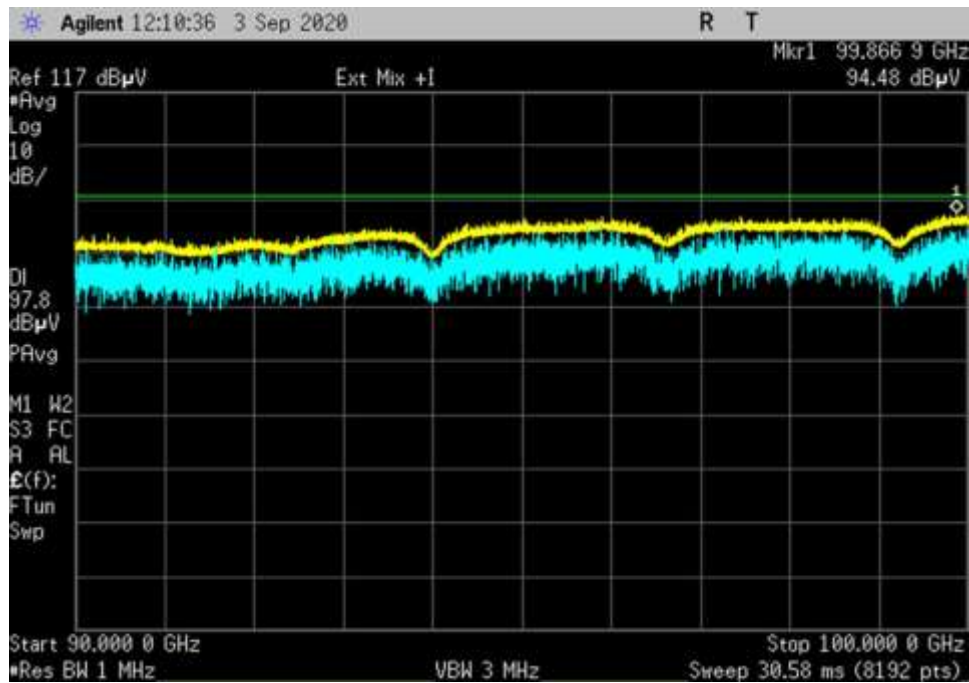
DL-Hout-QPSK-400MHz_ 90000- 100000MHz_MC-H
