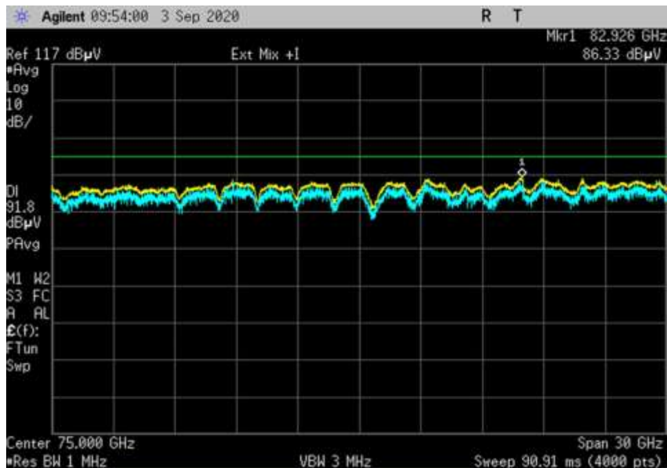
UL-Hout-QPSK-100MHz_ 60000- 90000MHz_MC-H
