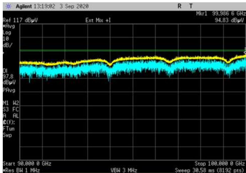
UL-Hout-QPSK-400MHz_90000-100000MHz_MC-H
