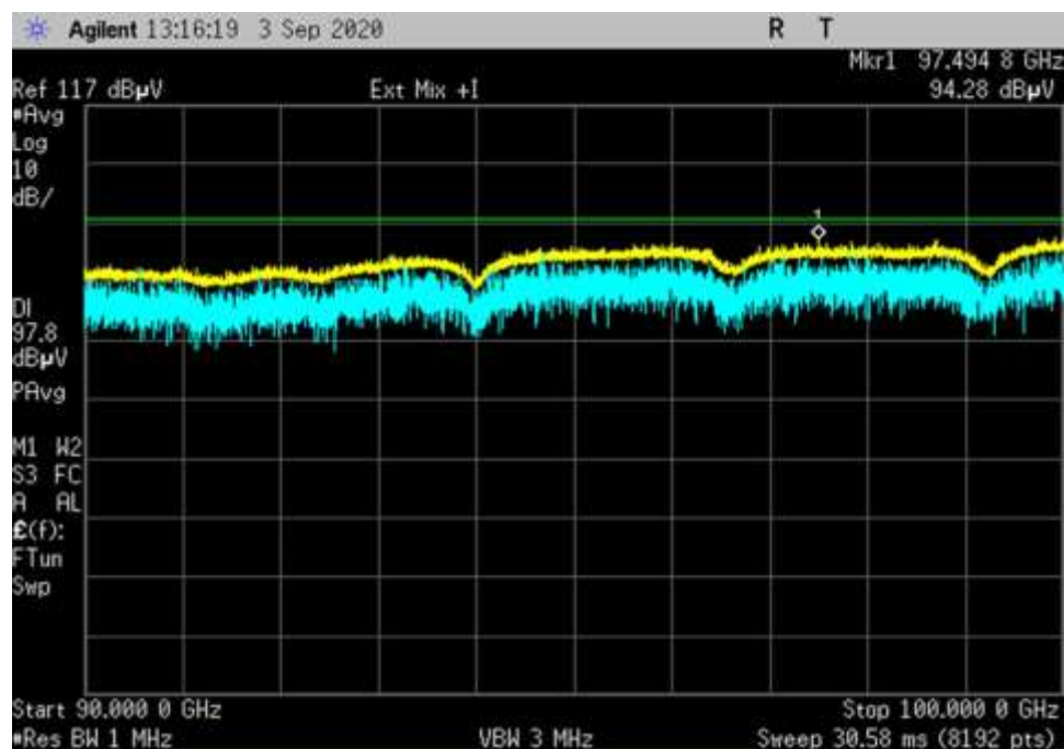
UL-Hout-QPSK-400MHz_90000-100000MHz_MC-V
