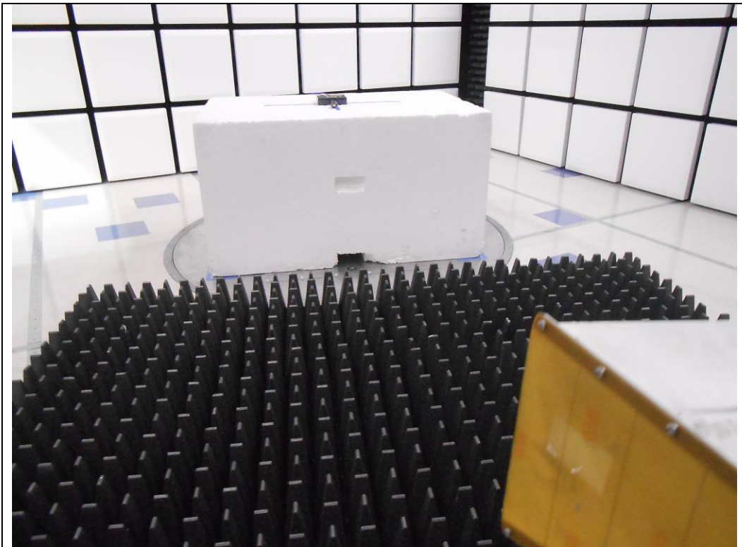
RF Radiated (1GHz and above testing)
