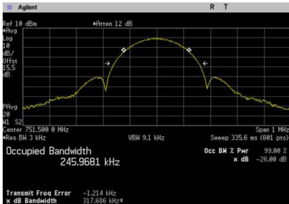
Out_DL_746-757_EDGE_751.5MHz
