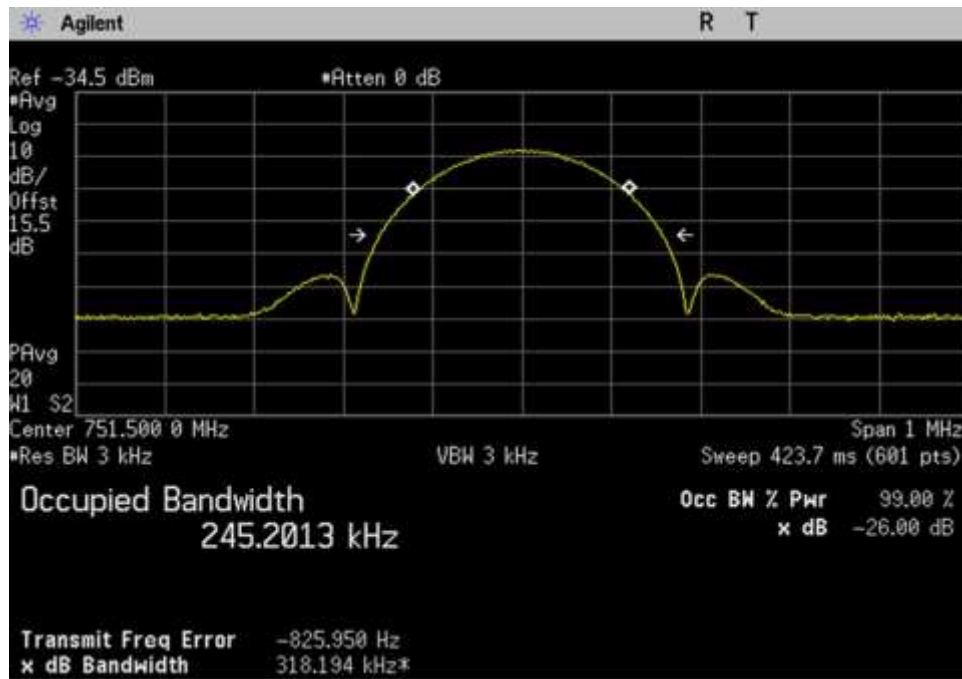
In_DL_746-757_EDGE_751.5MHz
