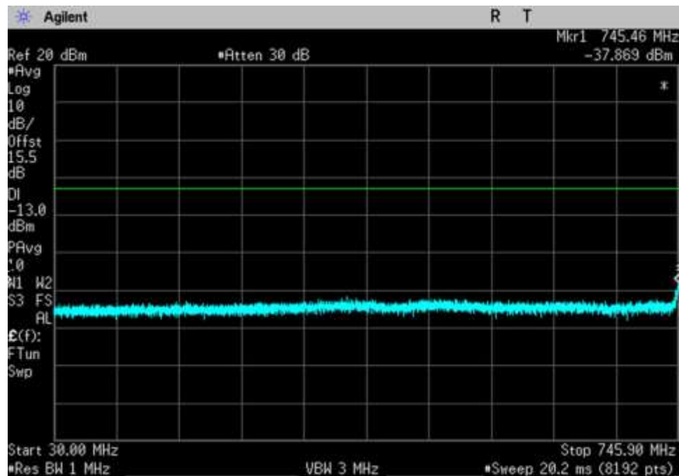
DL_746-757_30- 745.9MHz_SN4
