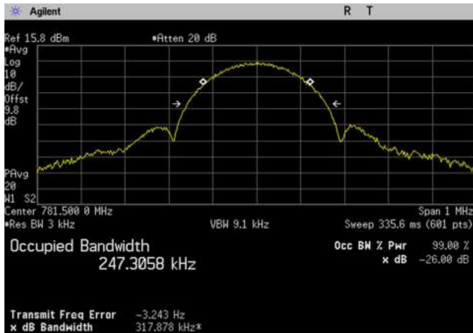
Out_UL_776-787_EDGE_781.5MHz
