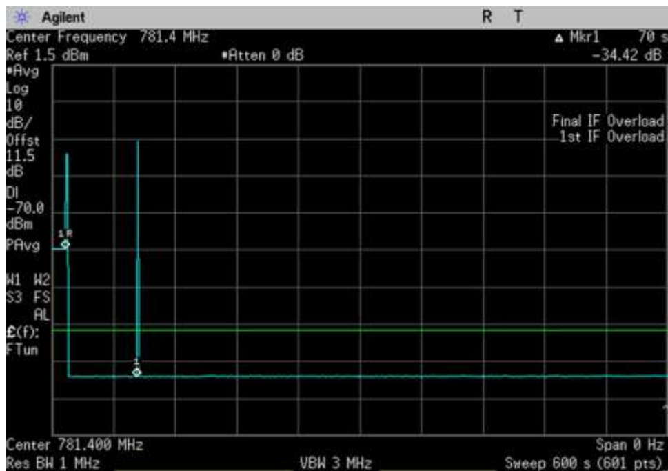
UL_776-787_600sec_ 781.4MHz_SN4
