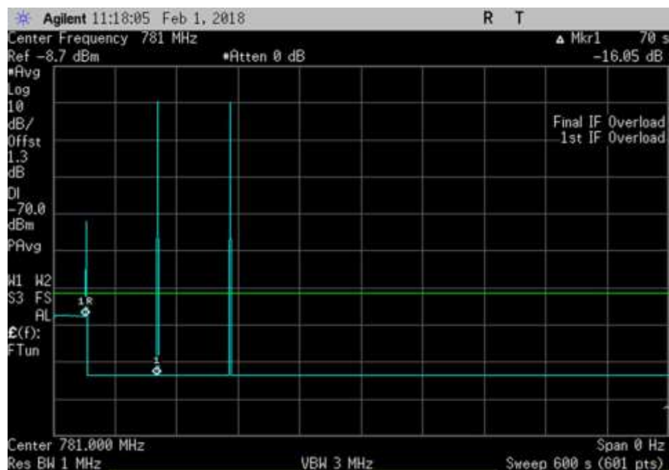
UL_776-787_600sec_781MHz
