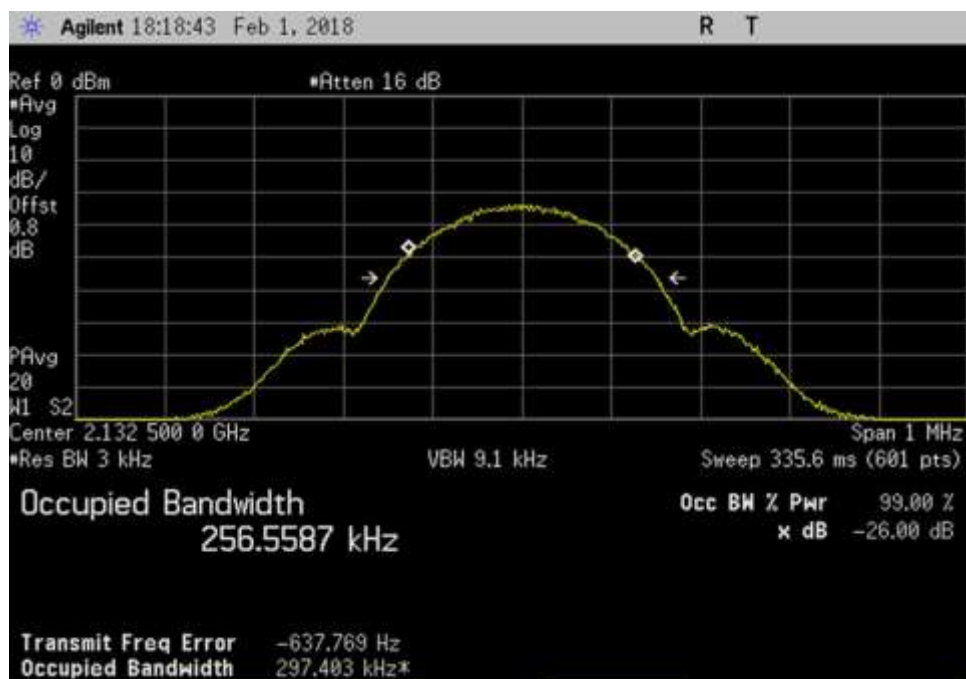
DL_2110-2155_GSM_2132.5MHz
