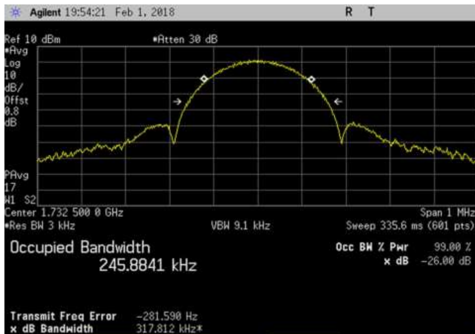
UL_1710-1755_EDGE_ 1732.5MHz
