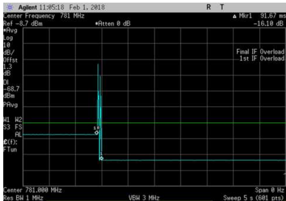
UL_776-787_781MHz
