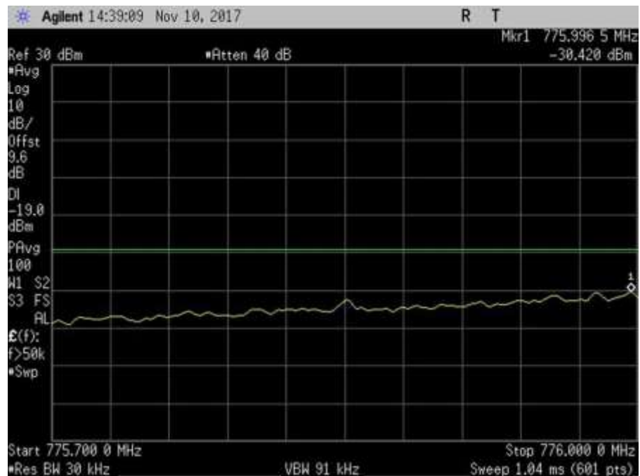
7.5_OBE_UL_776-787MHz_L_PreAGC_CDMA
