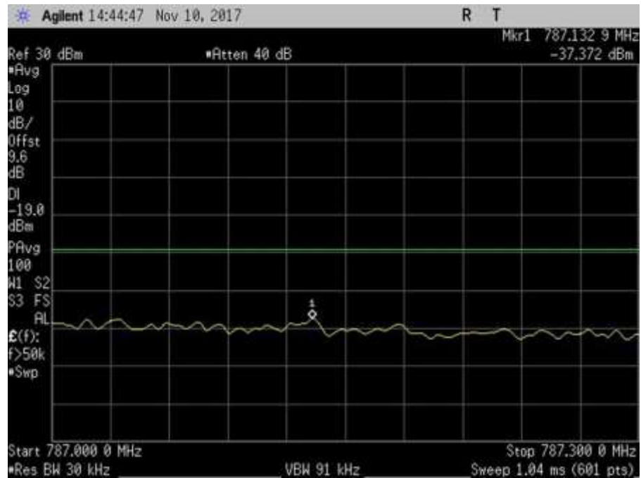
7.5_OBE_UL_776-787MHz_H_PreAGC_CDMA
