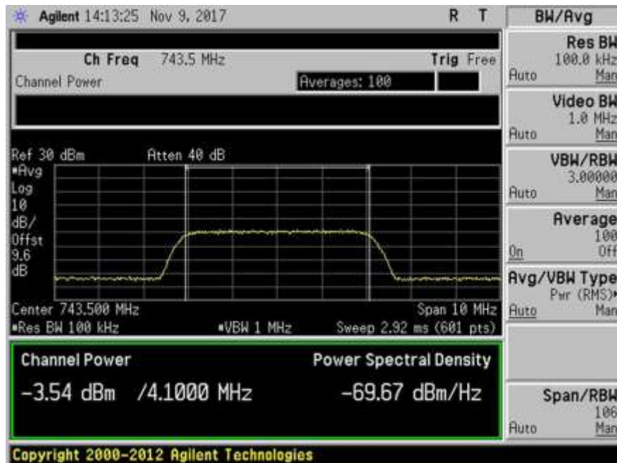
7.2_Power_DL_728-746MHz_AWGN
