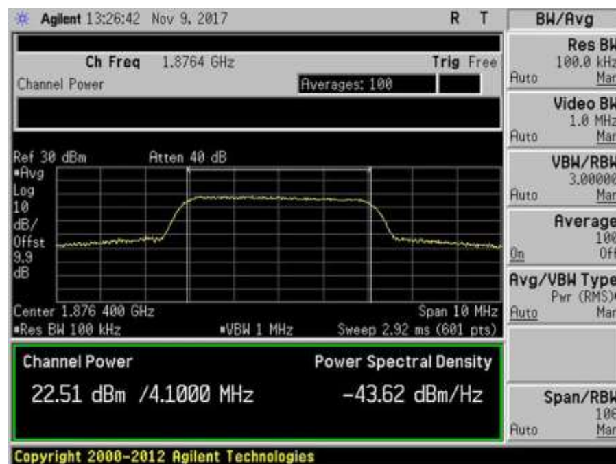
7.2_Power_UL_1850-1915MHz_AWGN_Max
