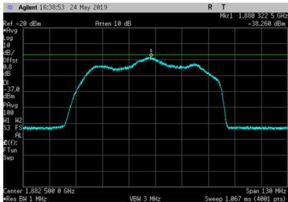
UL_1850-1915_1882.5MHz_100ft Cable
