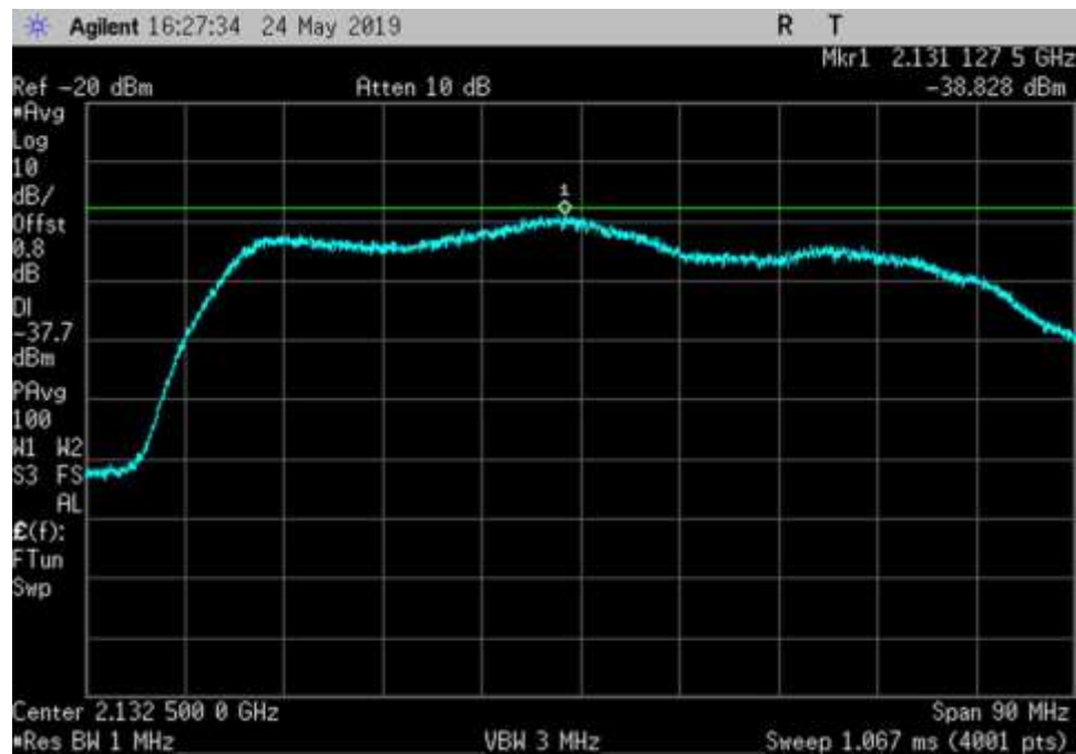
DL_2110-2155_2132.5MHz_50ft Cable
