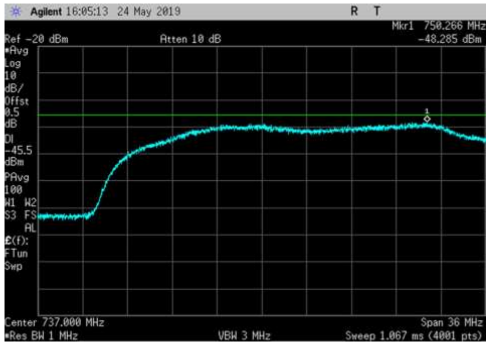
DL_728-746_ 737MHz_150ft Cable
