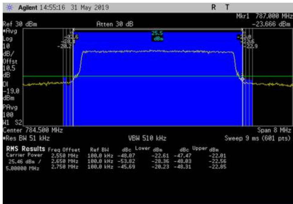
UL_776-787_LTE_ 780.5- 788.5MHz_100ft Cable
