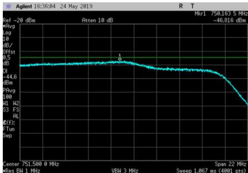
DL_746-757_751.5MHz_100ft Cable
