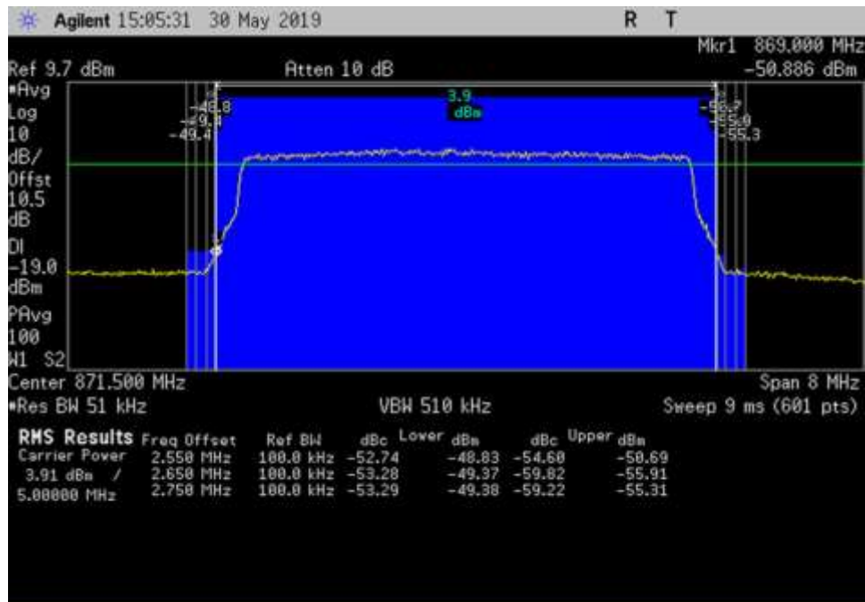
DL_869-894_LTE_867.5- 875.5MHz_100ft Cable
