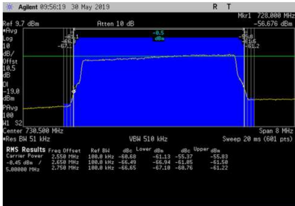
DL_728-746_LTE_ 726.5- 734.5MHz_150ft Cable
