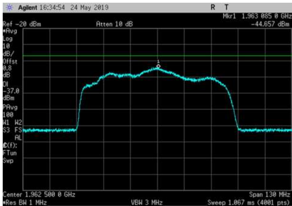
DL_1930-1995_1962.5MHz_100ft Cable
