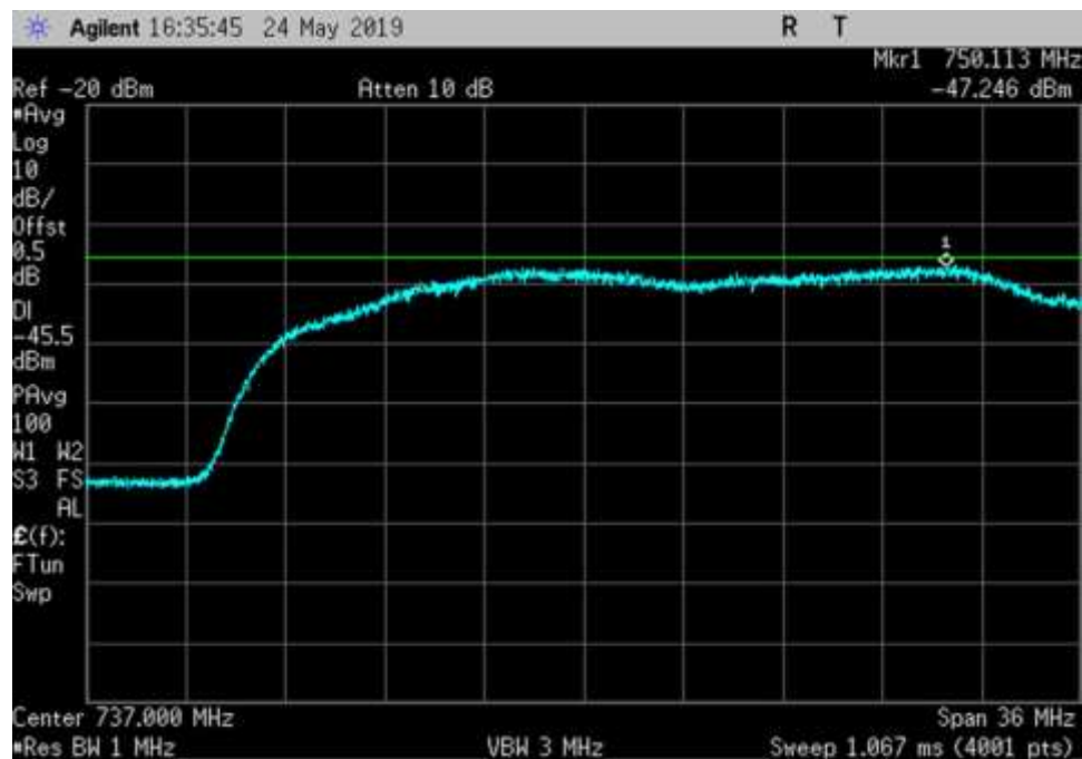
DL_728-746_737MHz_100ft Cable
