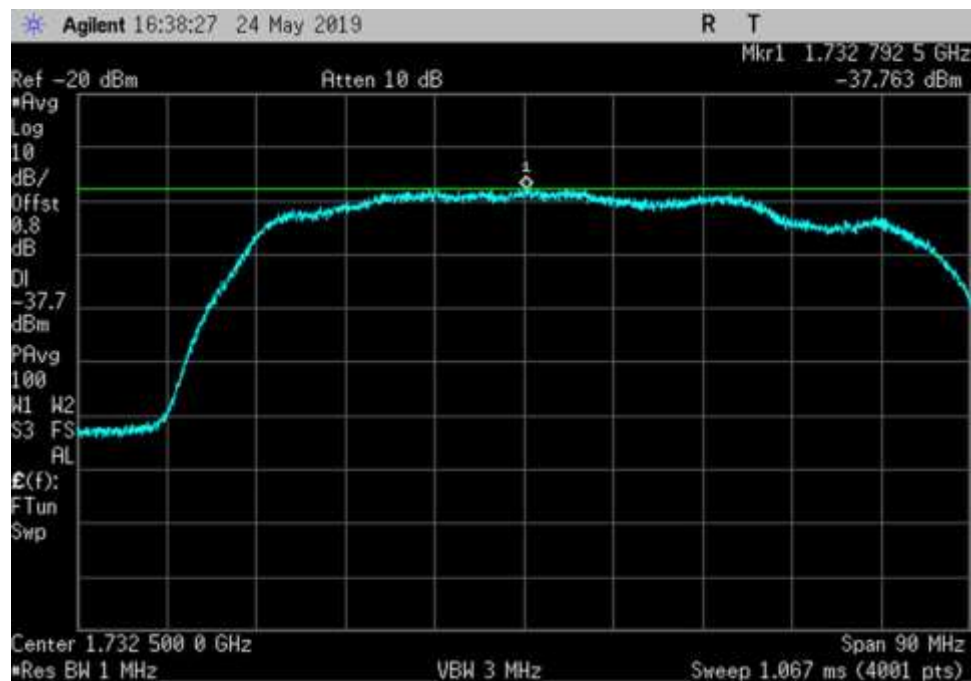
UL_1710-1755_1732.5MHz_100ft Cable
