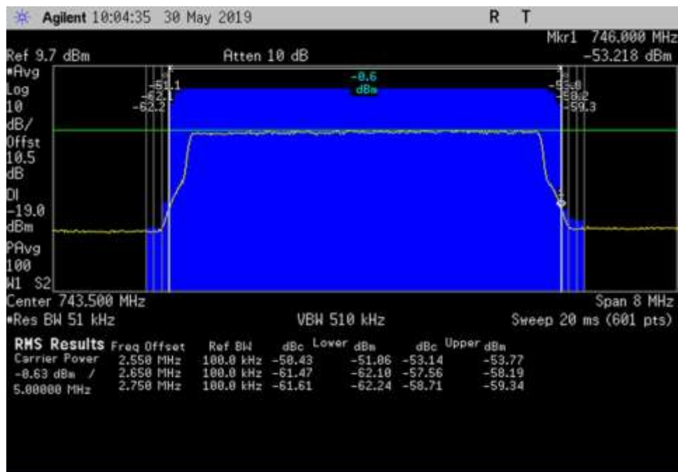
DL_728-746_LTE_ 739.5- 747.5MHz_150ft Cable
