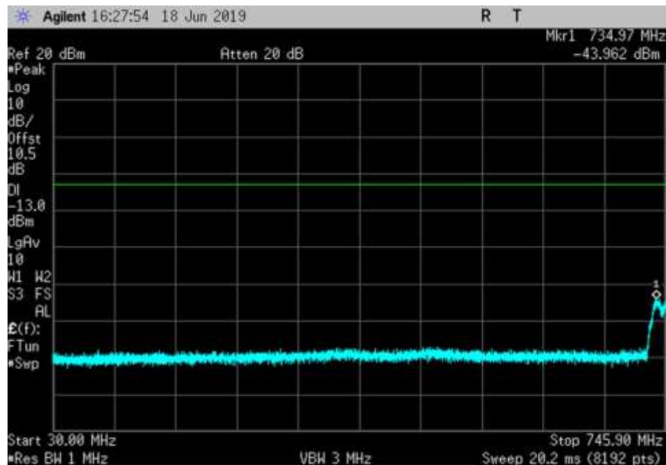
DL_746-757_ 30- 745.9MHz
