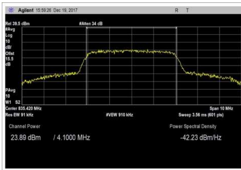
7.2 UL 824-849 AWGN_max
