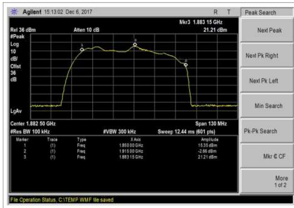
7.1 UL 1850-1915M
