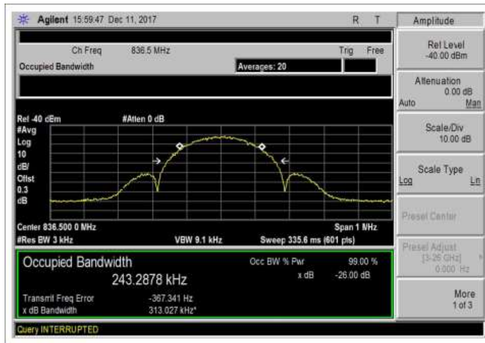
7.10 UL 824-849_EDGE_IN
