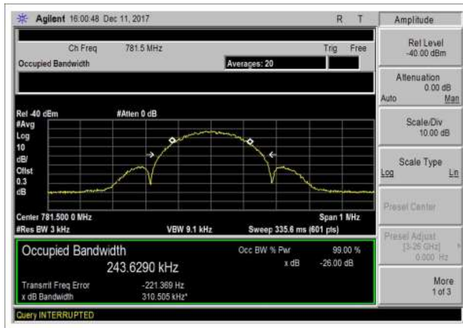
7.10 UL 776-787_EDGE_IN
