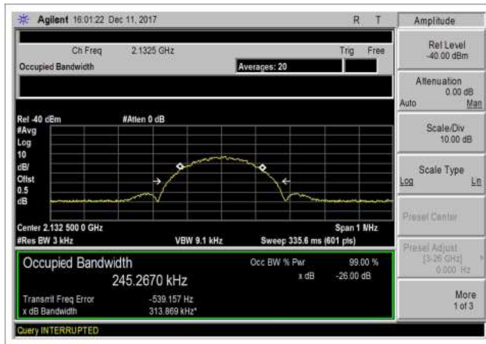
7.10 DL 2110-2155_EDGE_IN
