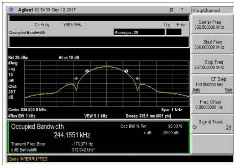
7.10 UL 824-849_EDGE_OUT
