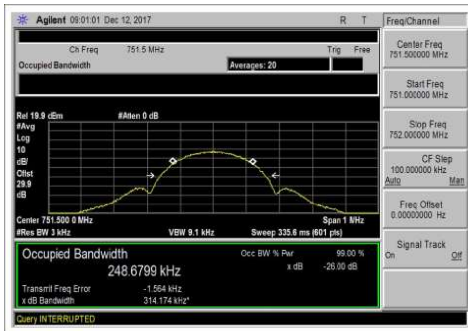
7.10 DL 746-757_EDGE_OUT
