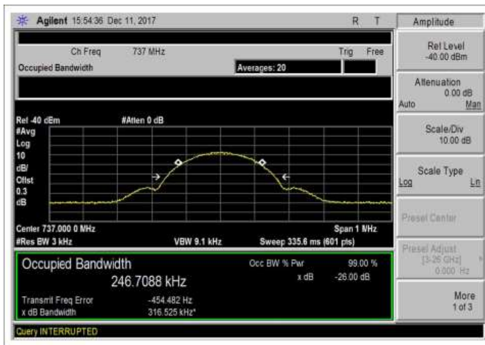
7.10 DL 728-746_GSM_IN
