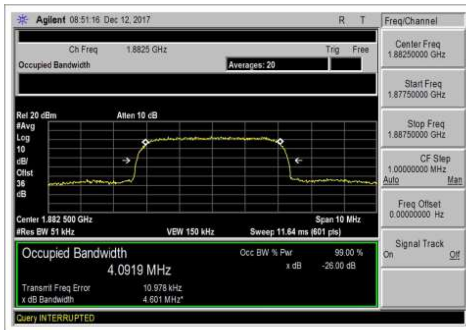
7.10 UL 1850-1915_WCDMA_OUT
