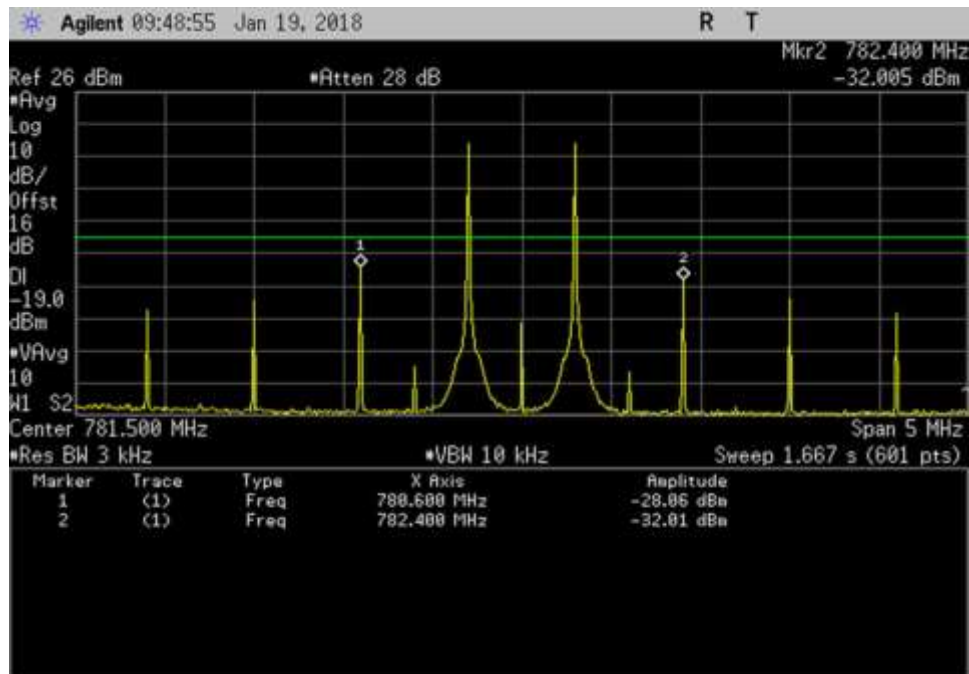
UL_781.5MHz
