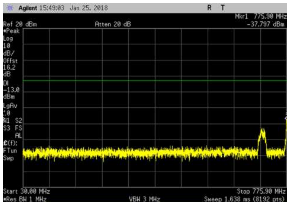
UL_ 30- 775.9MHz_AWGN
