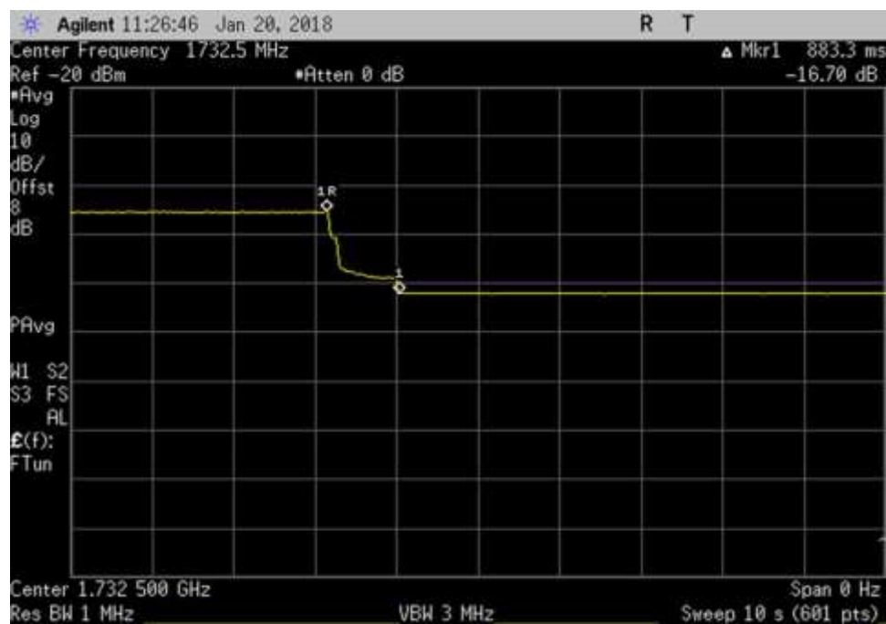
UL_1732.5MHz_Uplink Timing
