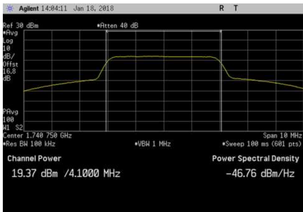
UL_ 1740.75MHz_AWGN_Max
