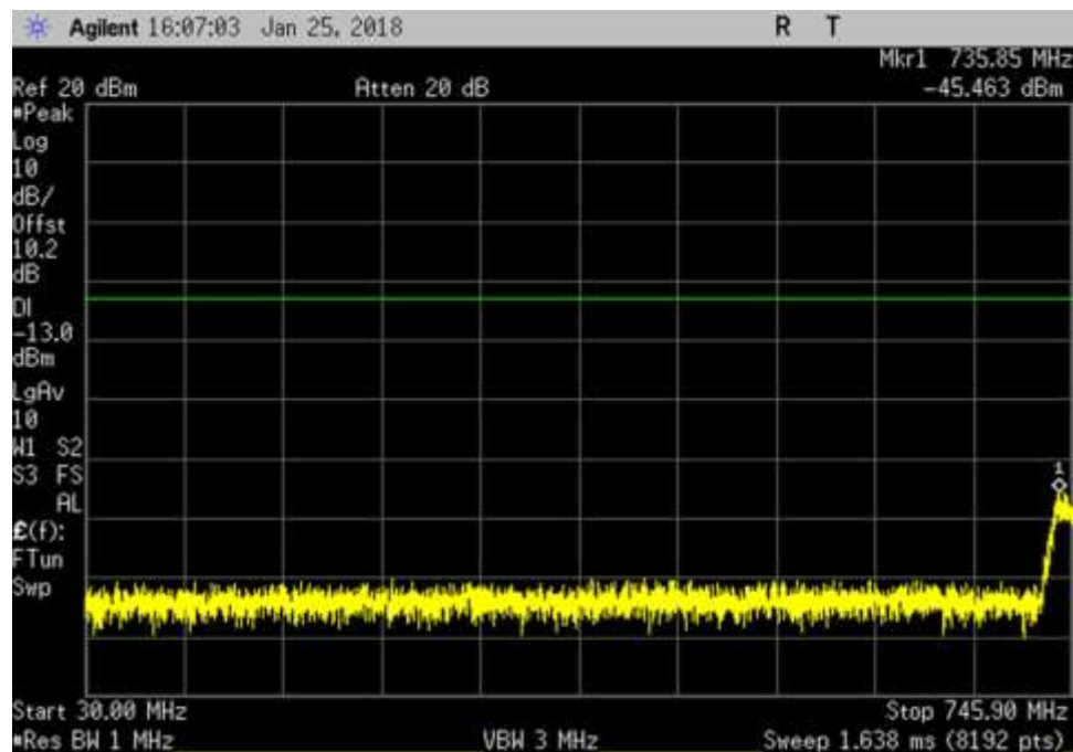
DL_ 30- 745.9MHz_AWGN
