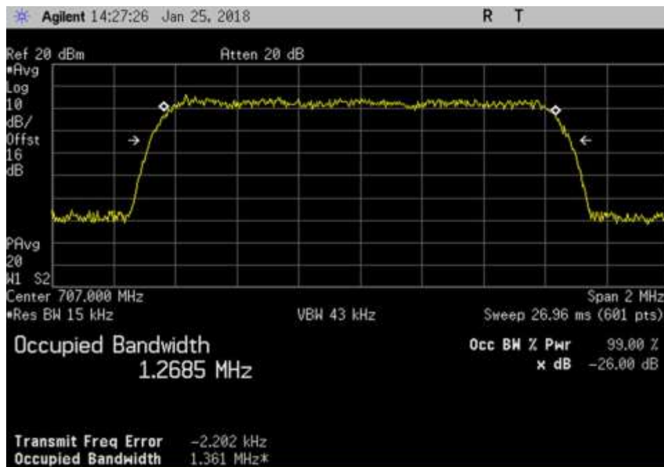
UL_707MHz_CDMA
