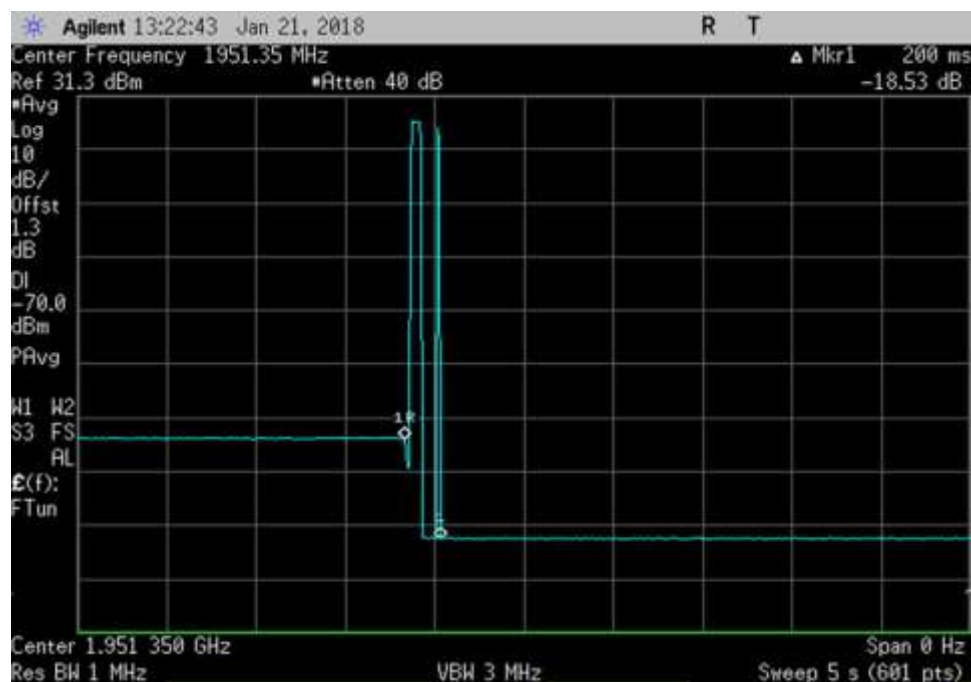
DL_ 1951.35MHz_time
