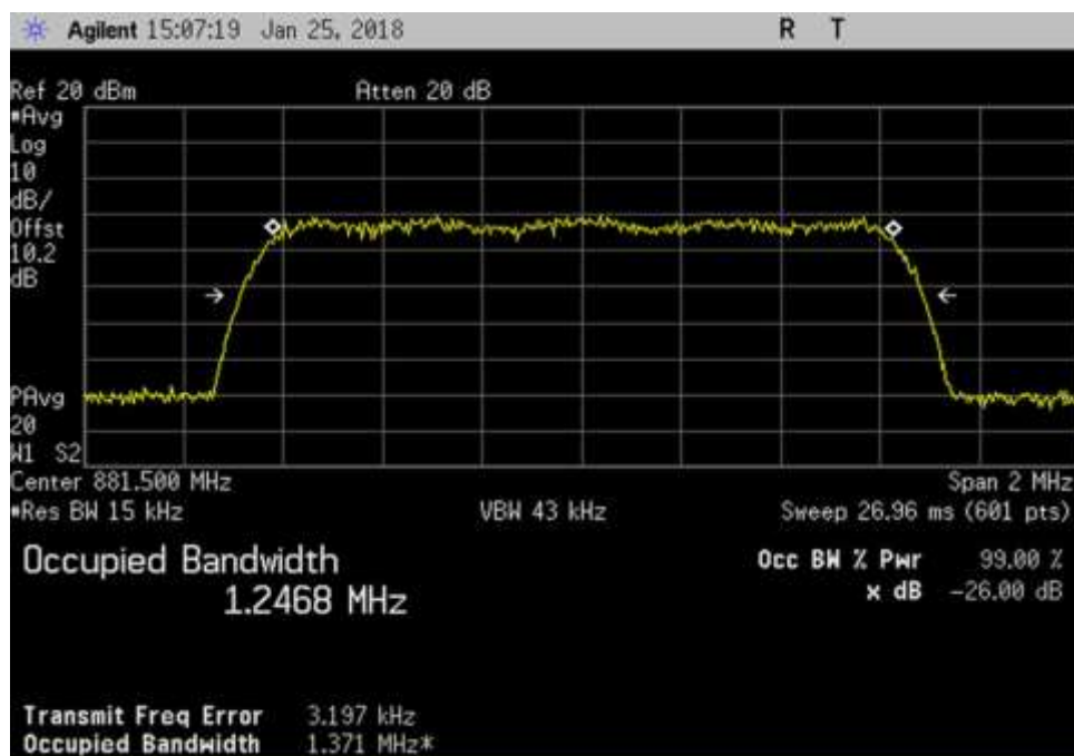
DL_881.5MHz_CDMA
