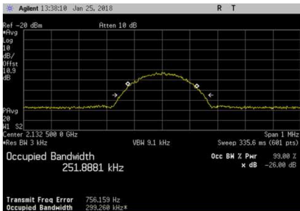
DL_2132.5MHz_EDGE
