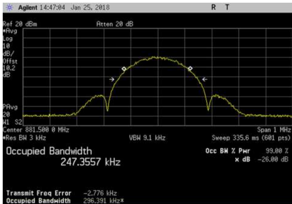
DL_881.5MHz_EDGE
