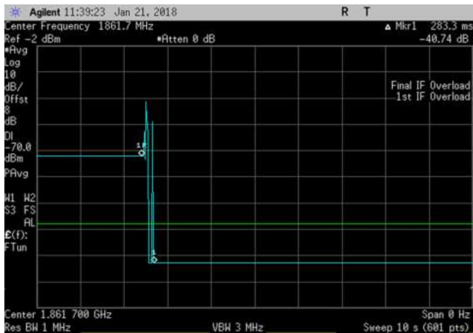
UL_1861.7MHz_time
