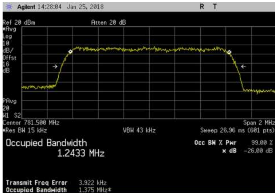
UL_781.5MHz_CDMA
