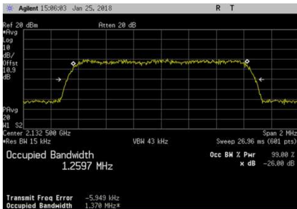
DL_2132.5MHz_CDMA
