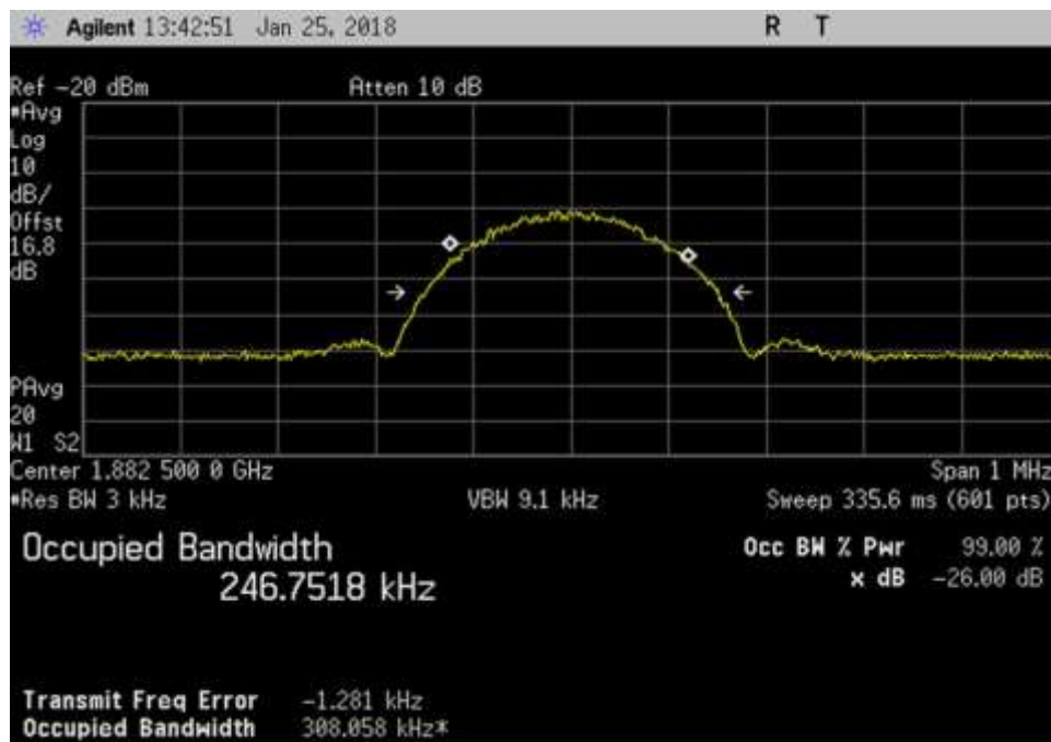
UL_1882.5MHz_EDGE
