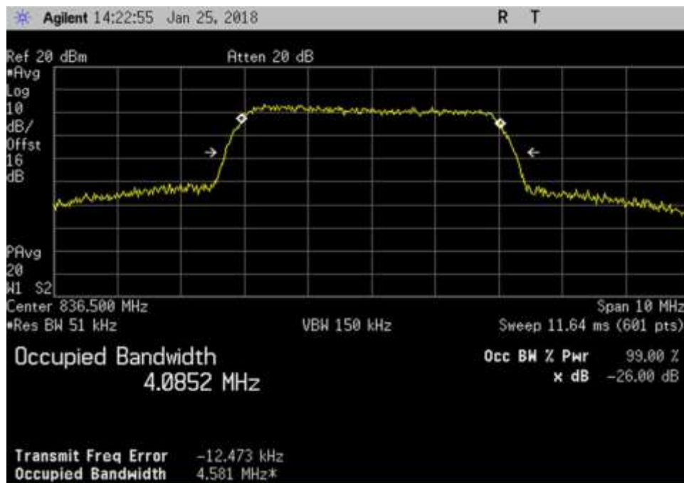
UL_836.5MHz_AWGN
