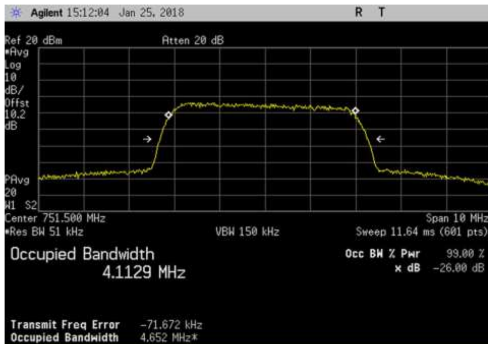
DL_751.5MHz_AWGN
