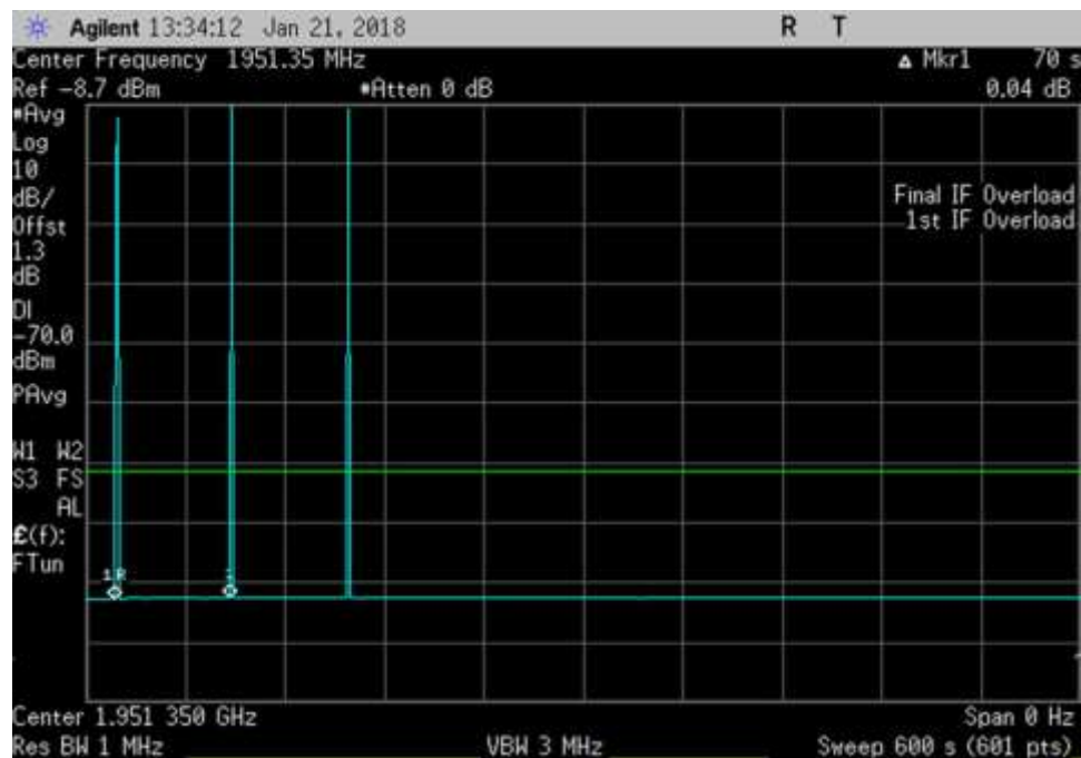
DL_ 1951.35MHz_600sec
