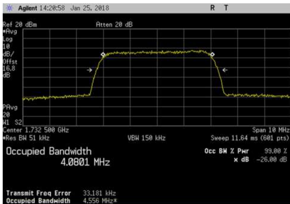
UL_1732.5MHz_AWGN
