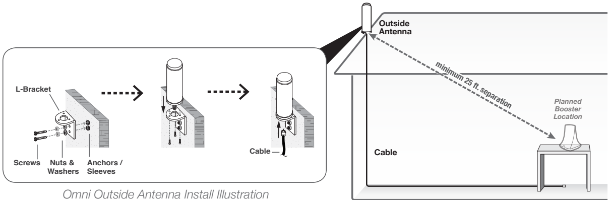
Omni Outside Antenna Install Illustration
