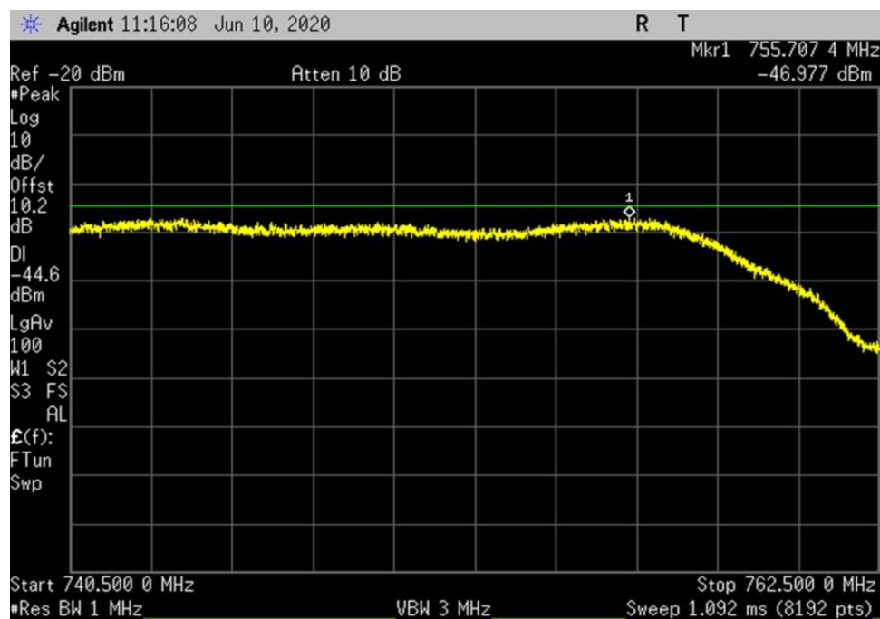
DL_746-757_751.5MHz_Max
