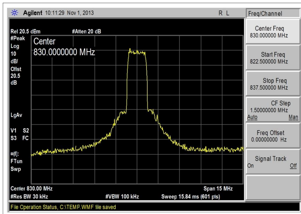
824-894MHz, UL_CDMA_Output
