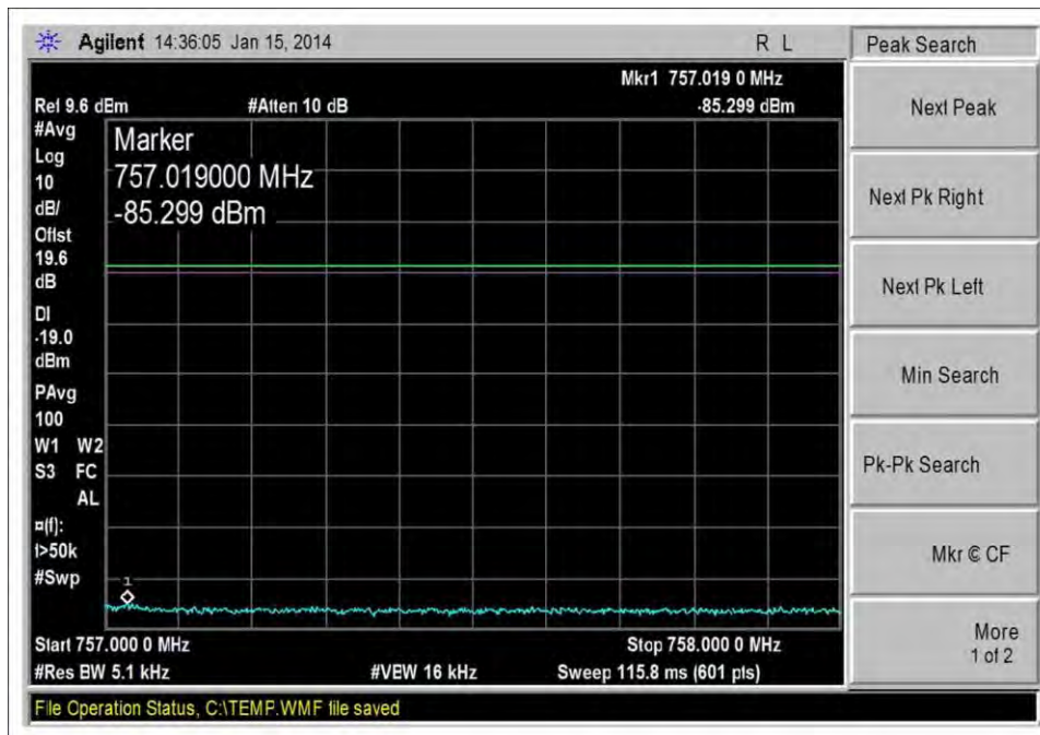
DL_746-757MHz_GSM_H_-20dBm
