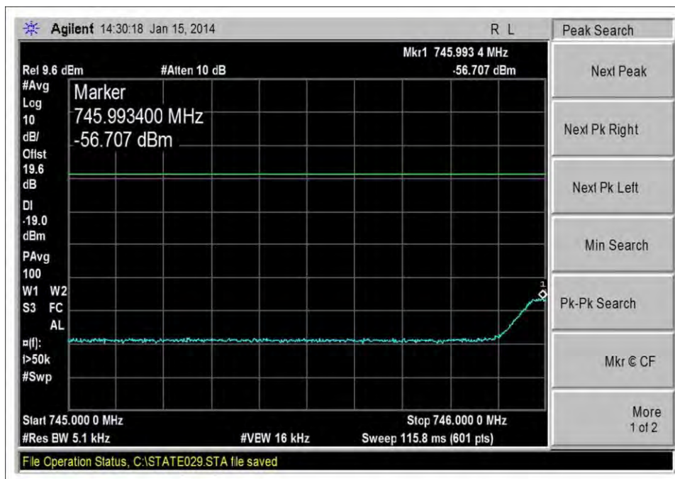
DL_746-757MHz_GSM_L_-67dBm
