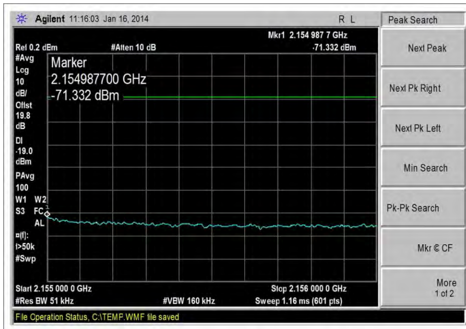
DL_2110-2155MHz_CDMA_H_-20dBm
