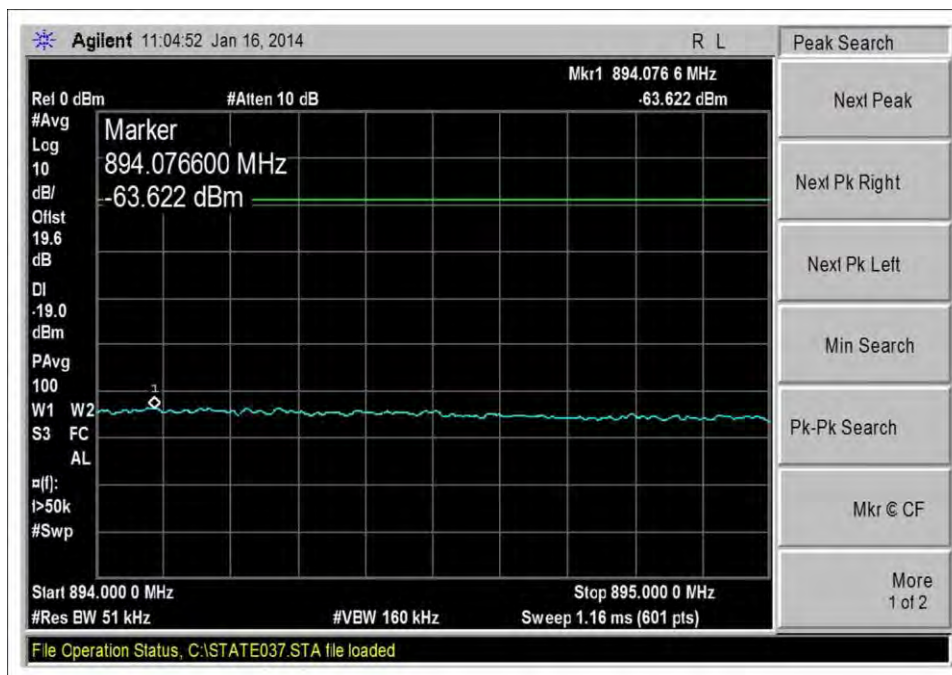
DL_891.5-894MHz_CDMA_L_-61dBm
