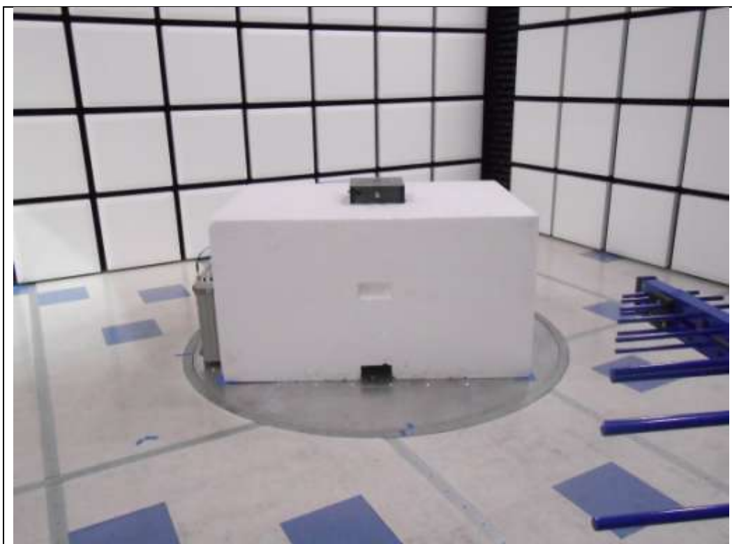
RF Radiated #2
