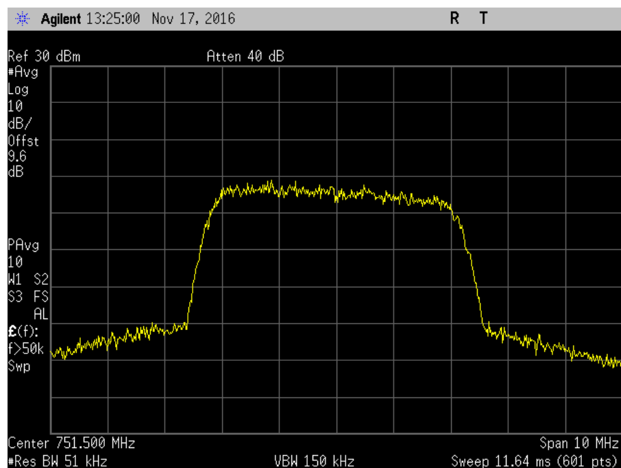
7.10_OBW_DL_746-757MHz_WCDMA_Out
