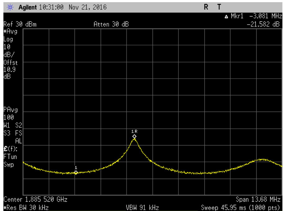
7.11.3_Osc_UL_1850-1915MHz+1_AWGNL
