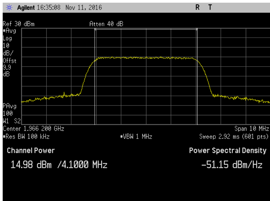
7.2_Power_DL_1930-1995MHz_AWGN_Max
