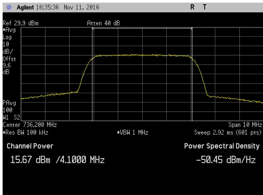
7.2_Power_DL_728-746MHz_AWGN_Max
