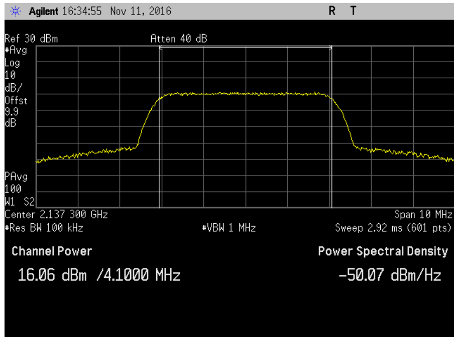
7.2_Power_DL_2110-2155MHz_AWGN_Max
