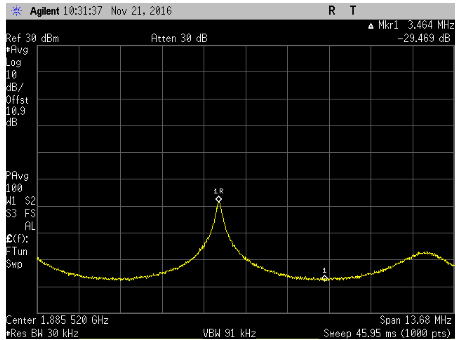
7.11.3_Osc_UL_1850-1915MHz+0_AWGNL
