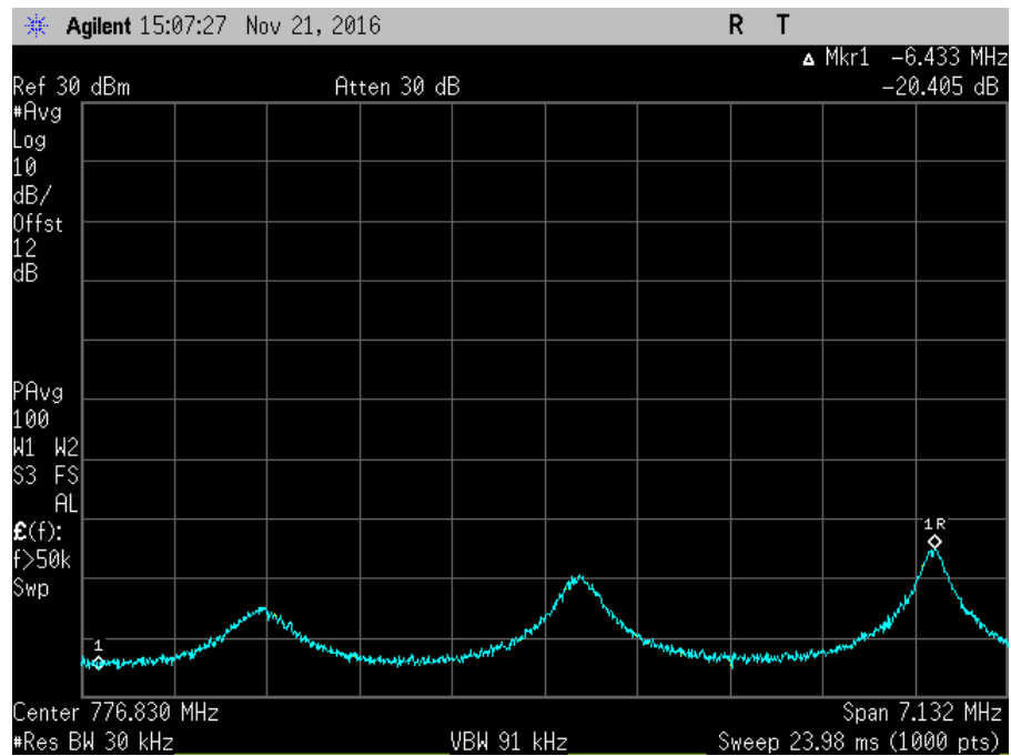
7.11.3_Osc_UL_776-787MHz-1_AWGNR
