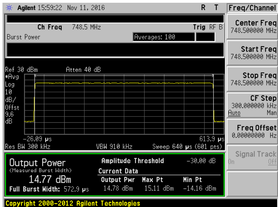
7.2_Power_DL_746-757MHz_GSM_Max
