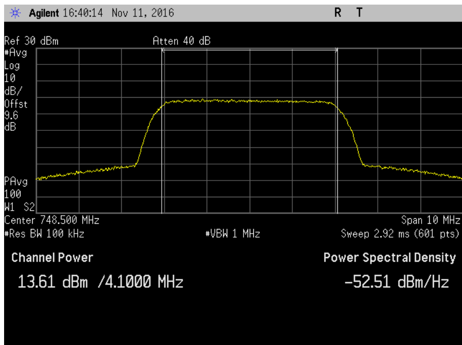
7.2_Power_DL_746-757MHz_AWGN_Max
