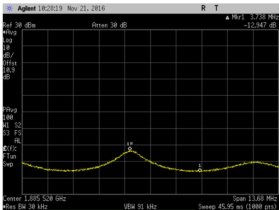
7.11.3_Osc_UL_1850-1915MHz+4_AWGNL
