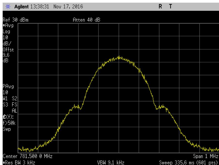
7.10_OBW_UL_776-787MHz_GSM_Out
