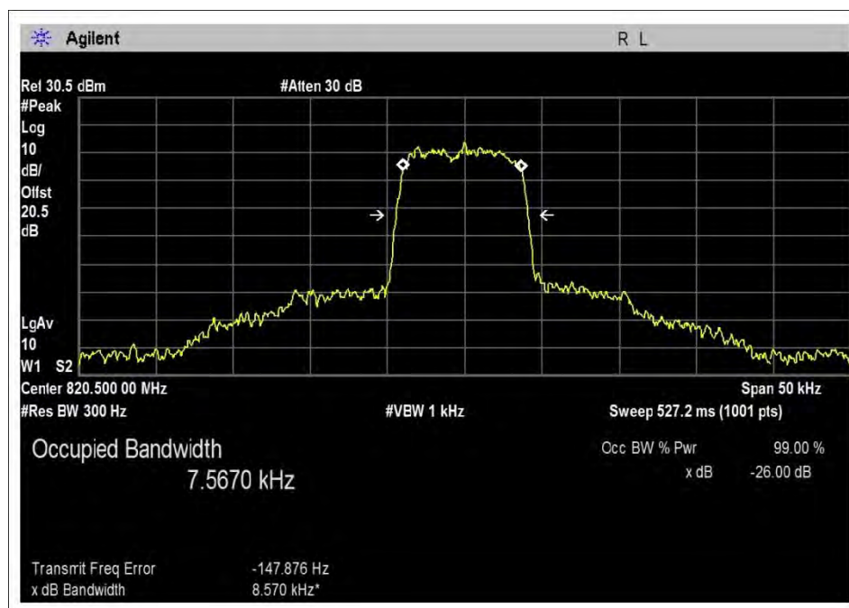
UL-817-824M-Out-27.4
