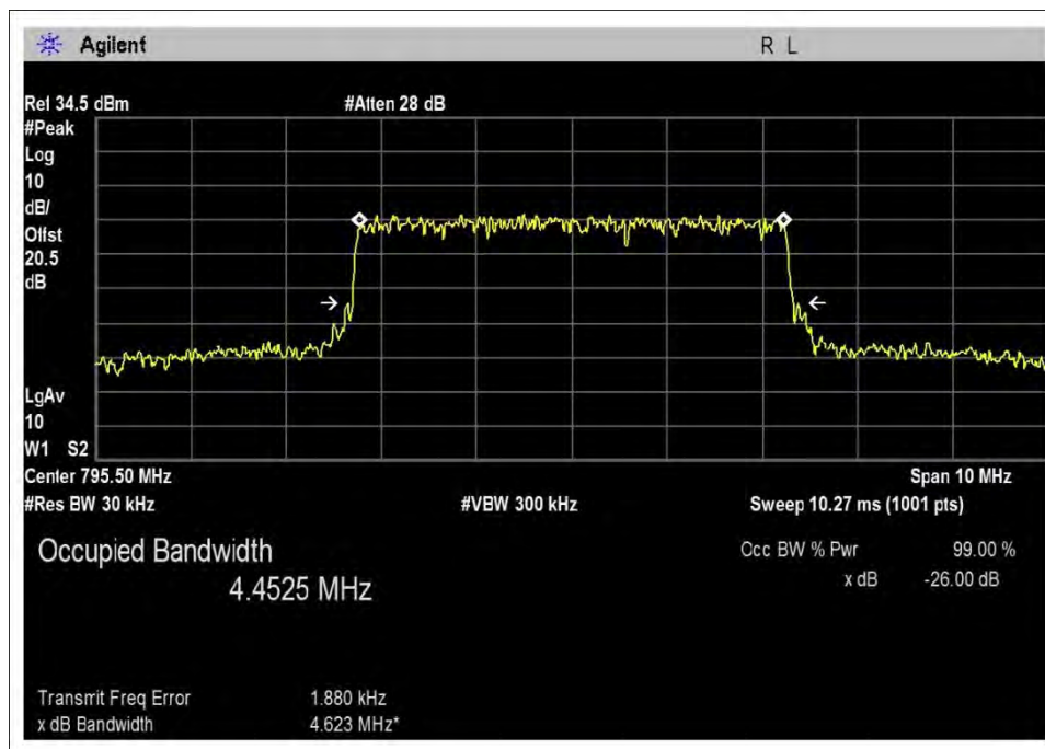
Output-UL-788-798H-AGC+10dB
