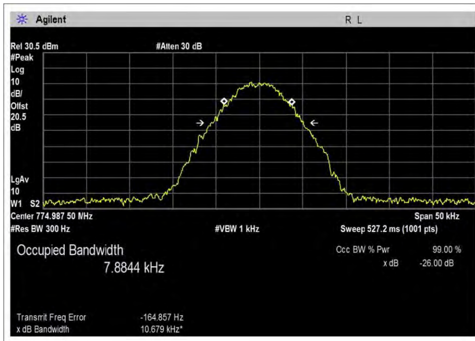
DL_775H-Out-31
