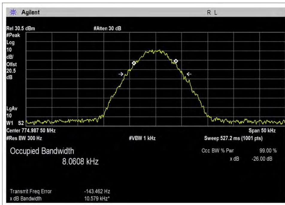
DL_775H-Out-AGC
