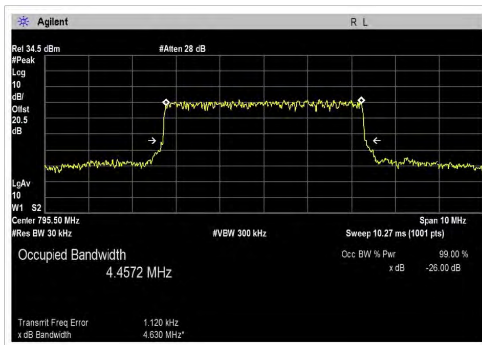
Output-UL-788-798H-AGC
