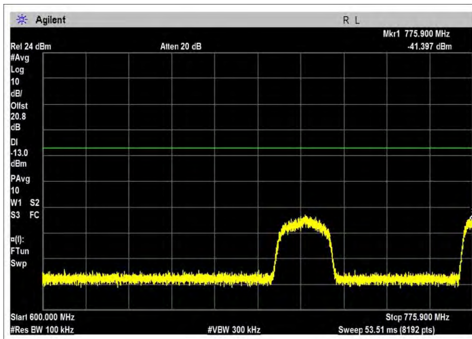
UL-698-716L-GSM-H
