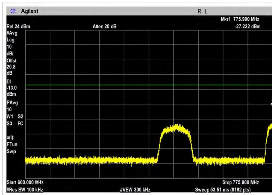
UL-776-787L-GSM-L
