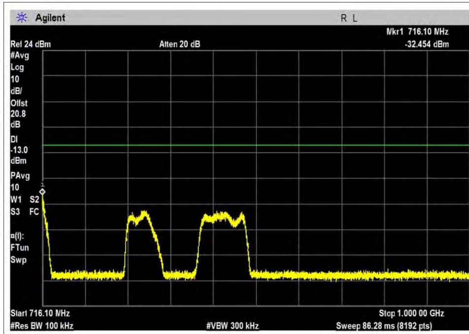
UL-698-716R-AWGN-H
