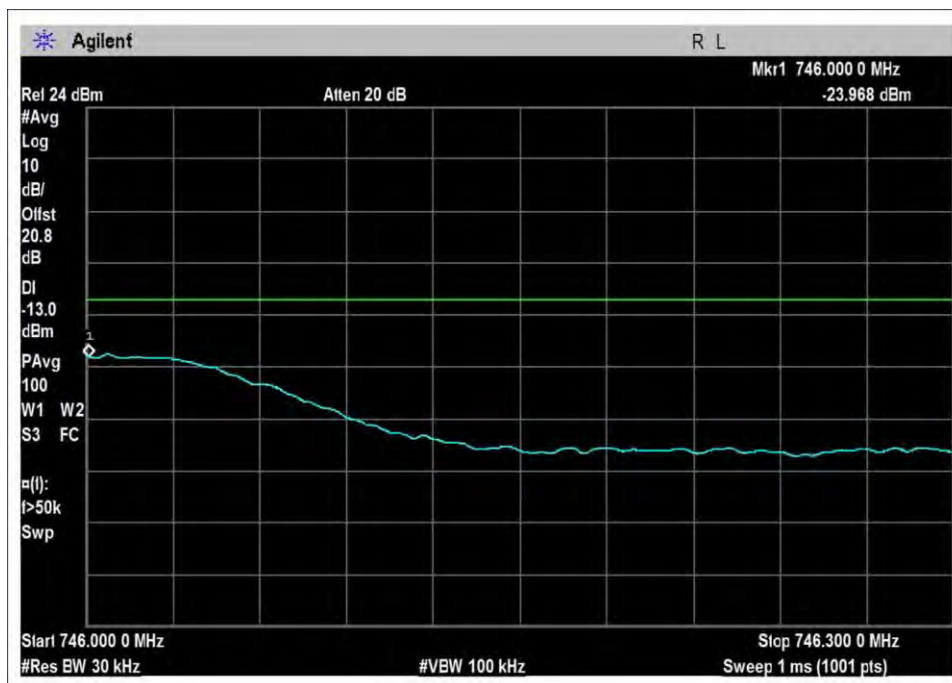
DL-728-746H-Sn-preAGC
