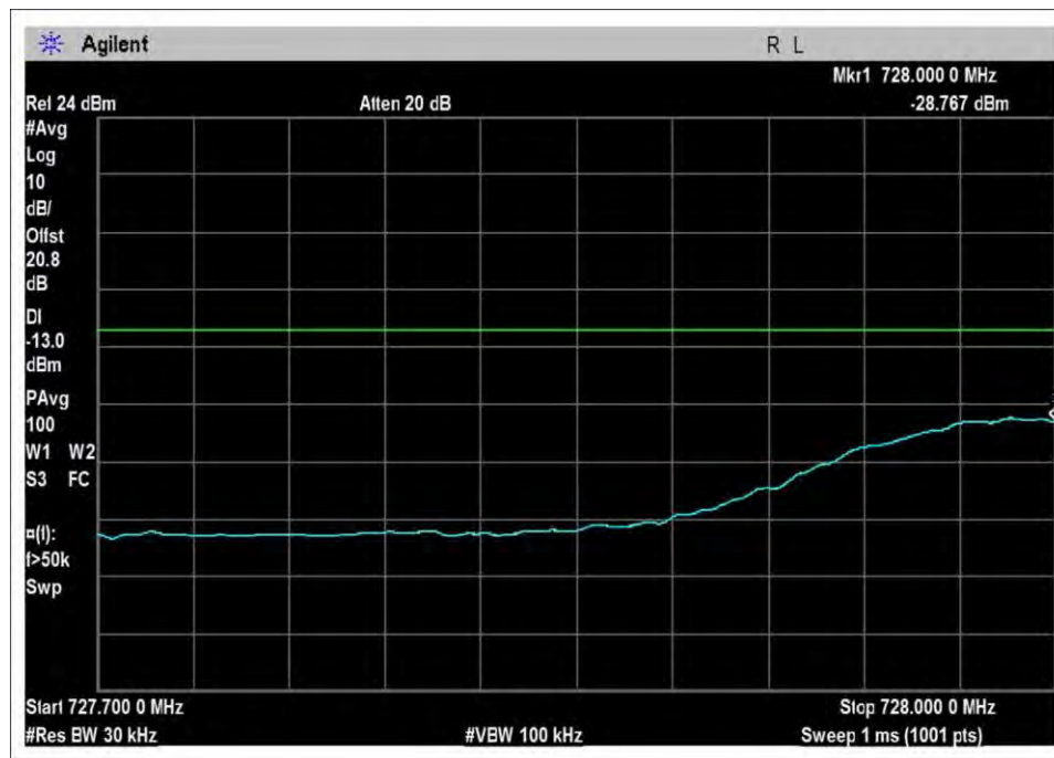
DL-728-746L-Sn-AGC+3
