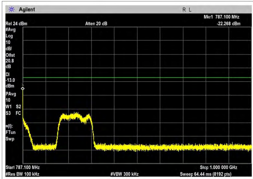
UL-776-787R-GSM-H
