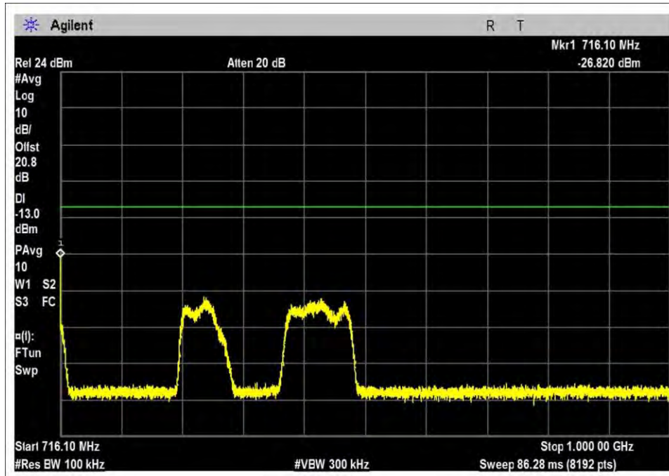
UL-698-716R-GSM-H
