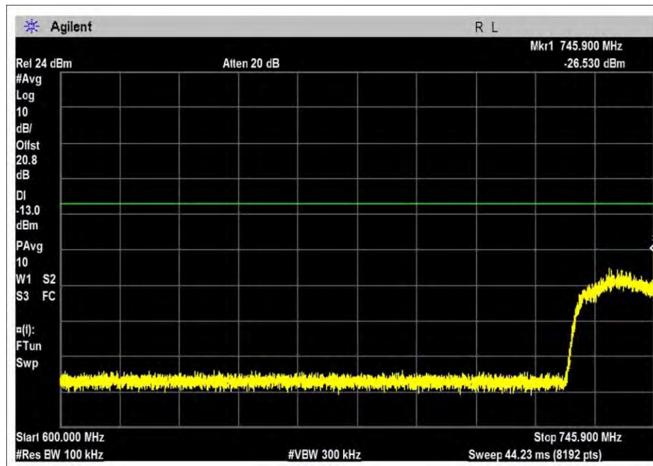
DL-746-757L-GSM-L
