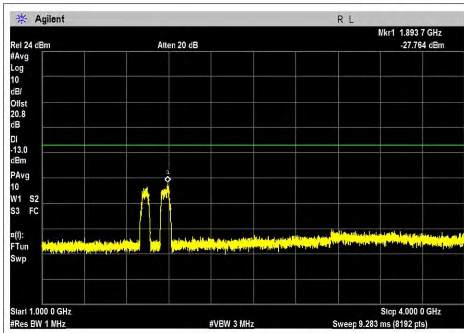
UL-776-787-GSM-L
