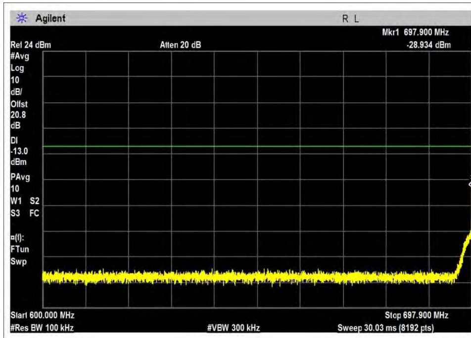
UL-698-716L-GSM-L
