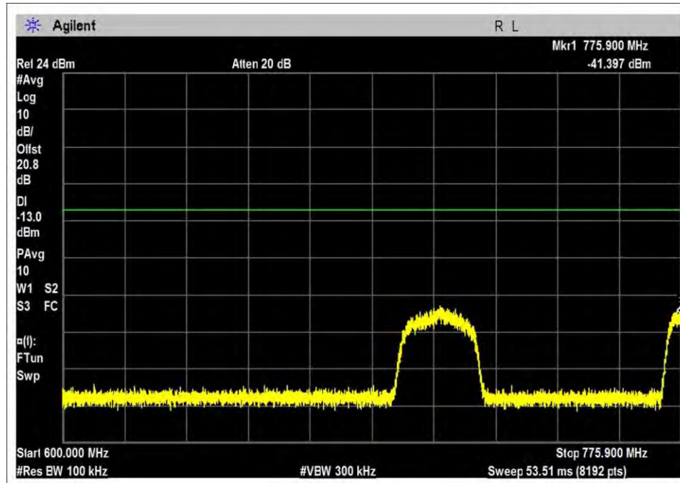
UL-776-787L-GSM-H
