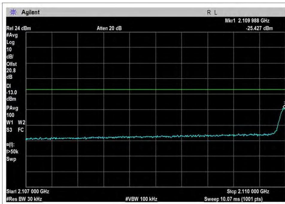
DL-2110-2155L-Sn-preAGC
