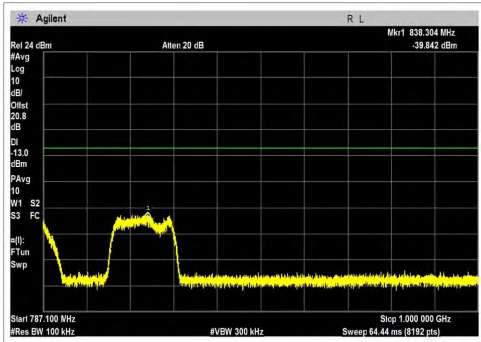
UL-776-787R-GSM-L
