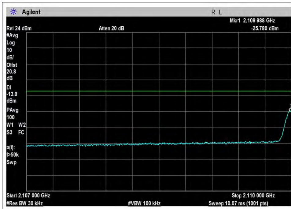
DL-2110-2155L-Sn-AGC+3
