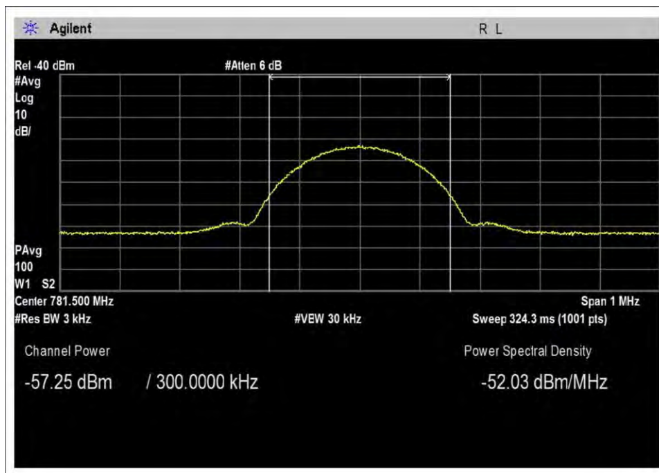
UL-776-787M-Input
