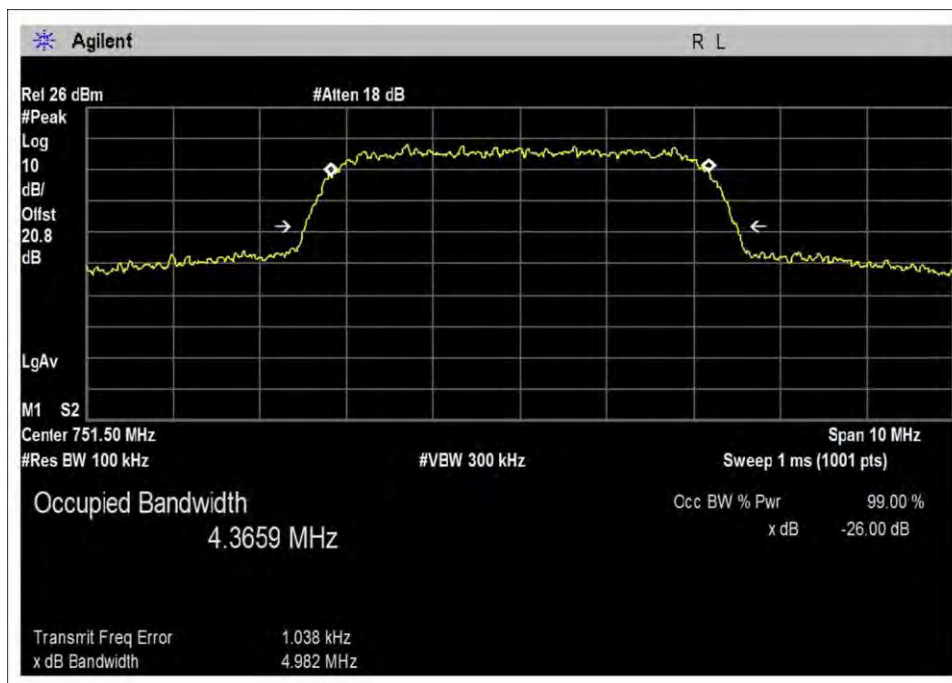
DL-746-757M-Out-49.6
