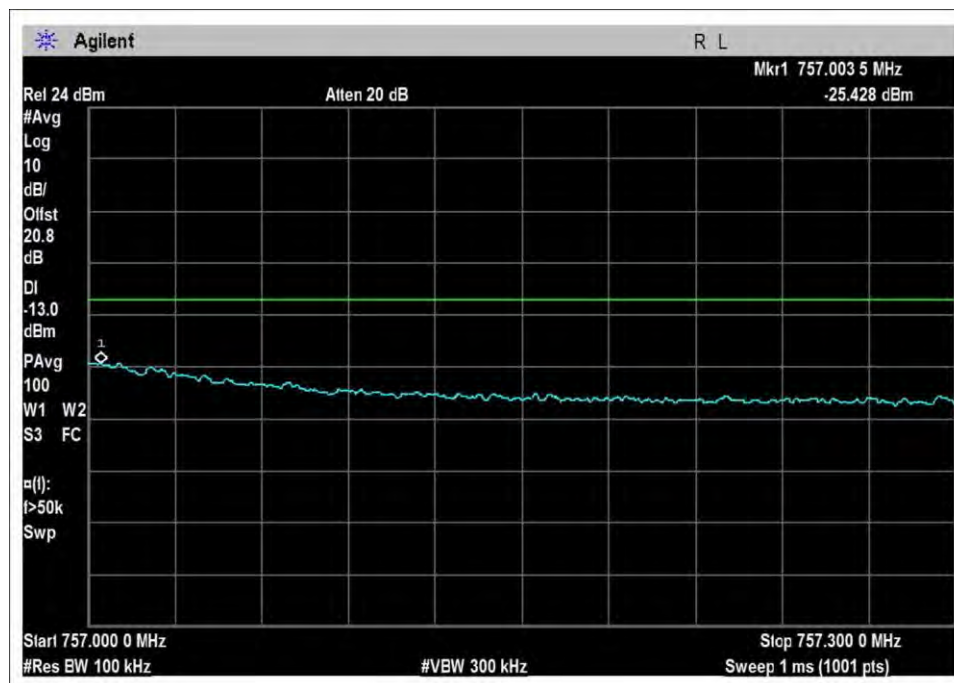
DL-746-757H-Sn-preAGC
