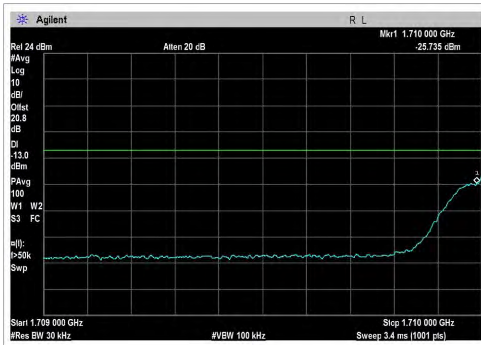
UL-1710-1755L-Sn-AGC+3
