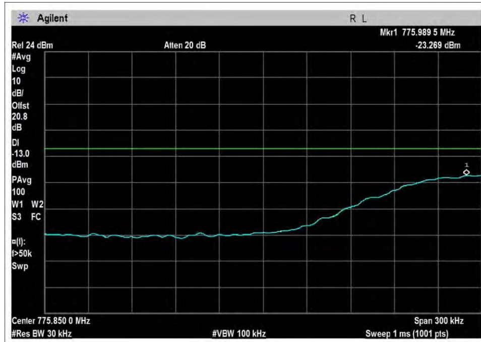
UL-776-787L-Sn-preAGC
