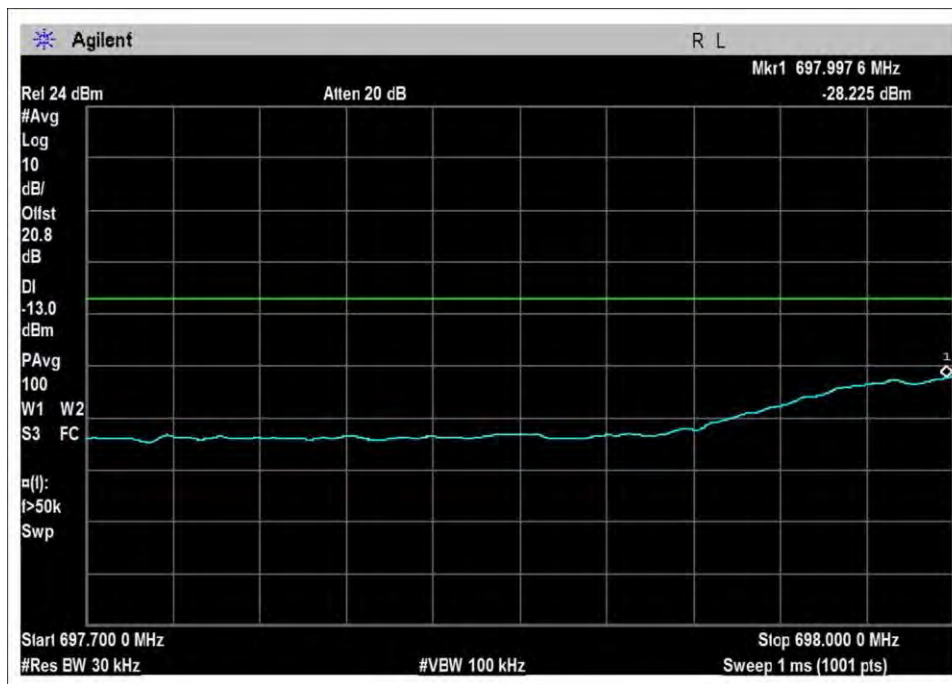
UL-698-716L-Cm-AGC+3
