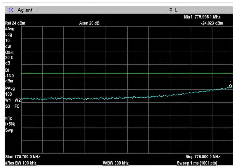
UL-776-787L-Cm-AGC+3
