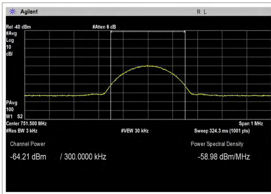
DL-746-757M-Input
