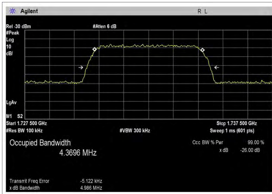
UL-1710-1755M-M-Input
