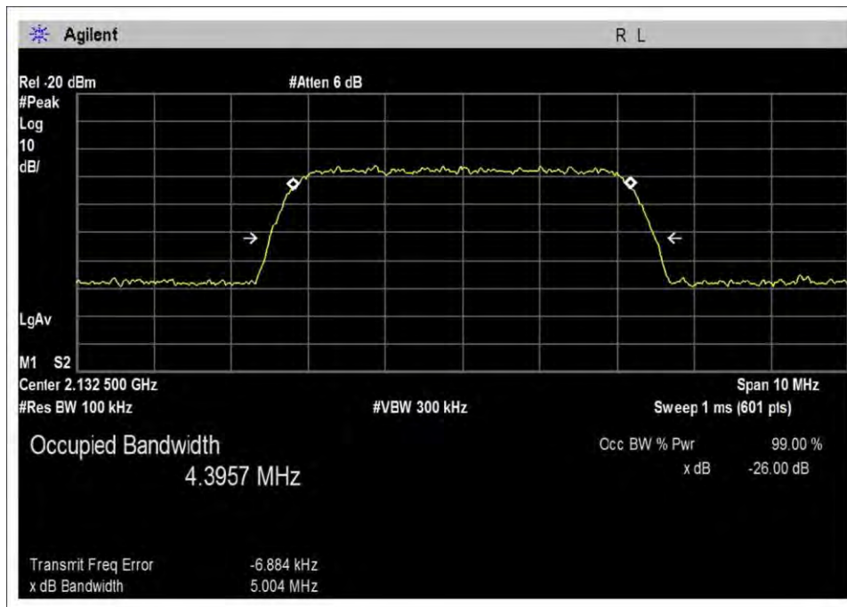
DL-2110-2155M-M-Input
