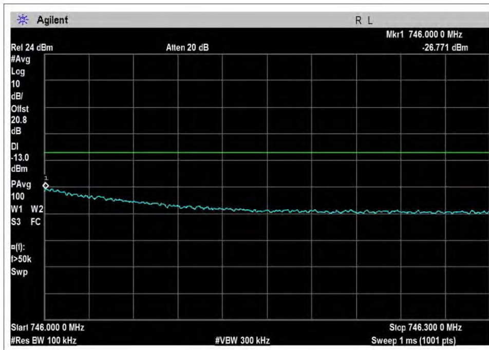
DL-728-746H-Cm-AGC+3
