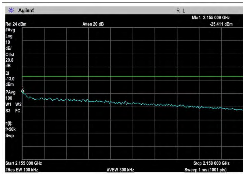
DL-2110-2155H-Sn-preAGC
