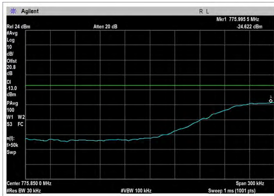
UL-776-787L-Sn-AGC+3
