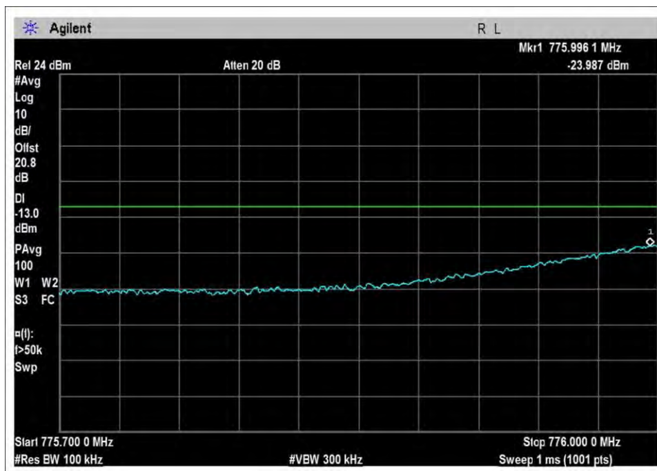
UL-776-787L-Sn-preAGC
