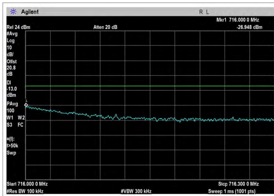
UL-698-716H-Cm-preAGC
