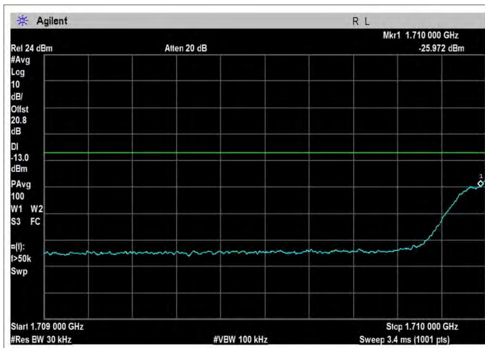
UL-1710-1755L-Sn-preAGC
