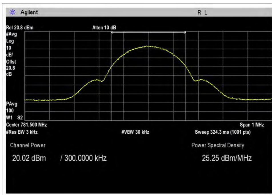
UL-776-787M-Out-42.9
