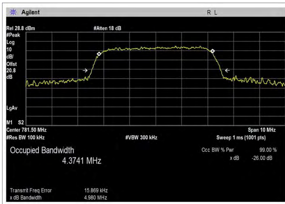
UL-776-787M-Out-43.1
