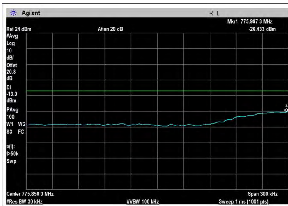
UL-776-787L-Cm-preAGC
