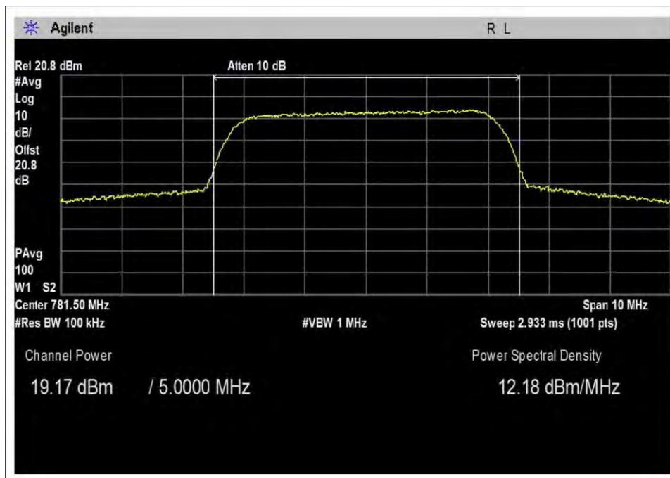
UL-776-787M-Out-43.1
