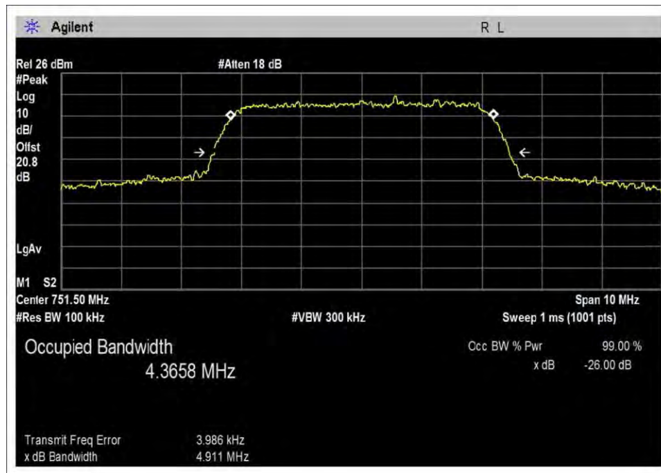
DL-746-757M-Out-AGC+3
