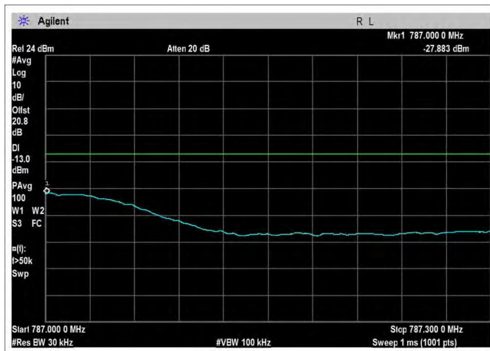
UL-776-787H-Cm-preAGC
