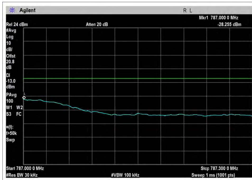
UL-776-787H-Cm-AGC+3
