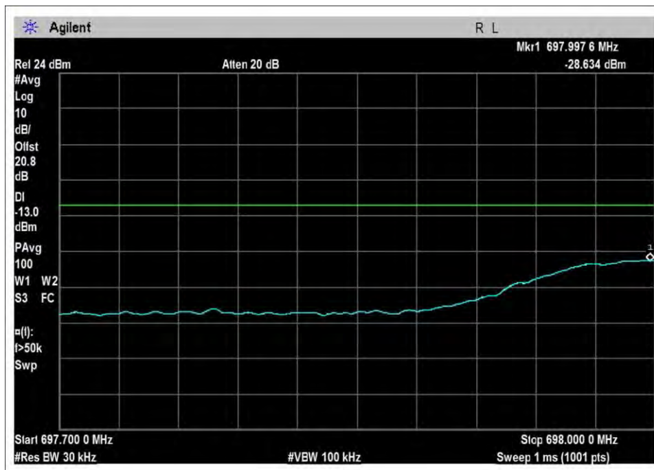
UL-698-716L-Cm-preAGC
