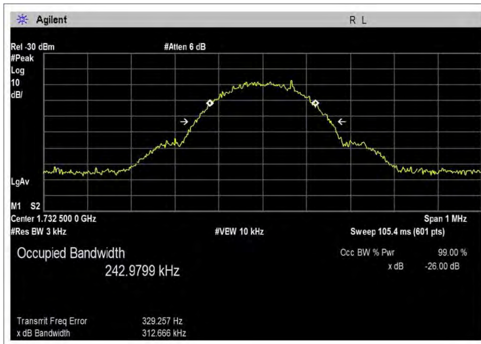
UL-1710-1755M-Input
