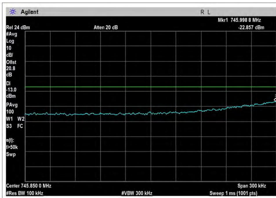
DL-746-757L-Sn-preAGC
