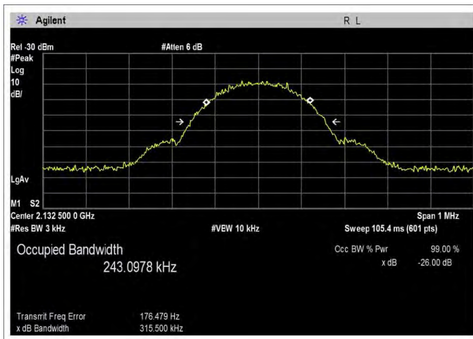
DL-2110-2155M-Input
