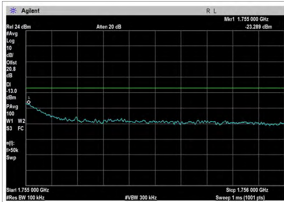
UL-1710-1755H-Sn-preAGC
