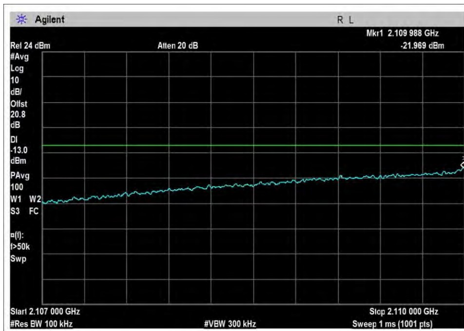
DL-2110-2155L-Sn-preAGC
