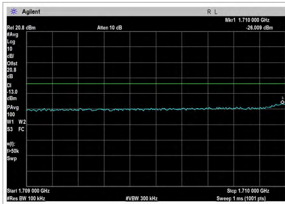
UL-1710-1755L-Cm-AGC+3dB
