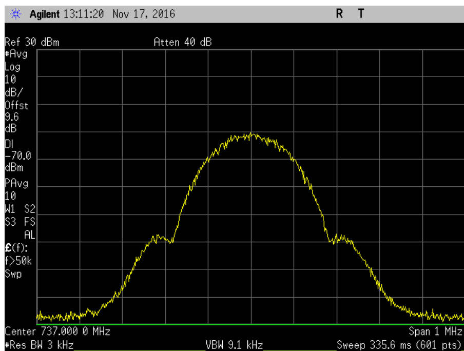
7.10_OBW_DL_728-746MHz_GSM_Out
