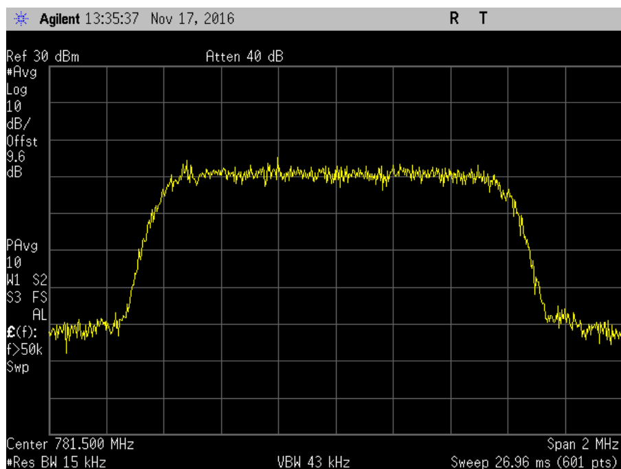
7.10_OBW_UL_776-787MHz_CDMA_Out
