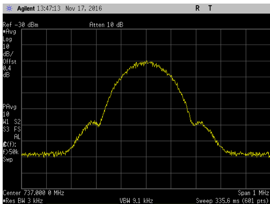
7.10_OBW_DL_728-746MHz_GSM_In
