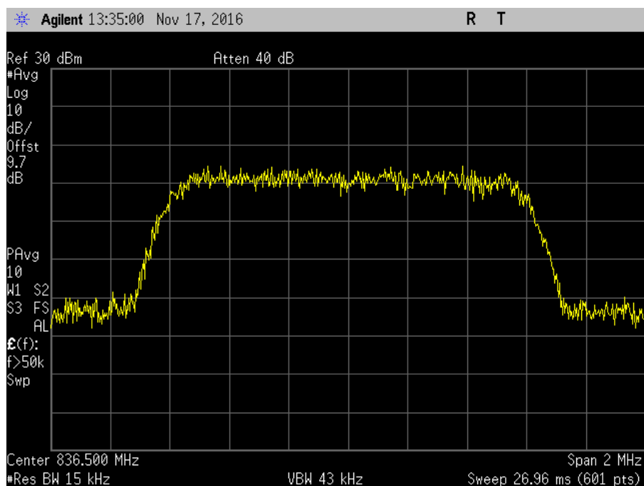
7.10_OBW_UL_824-849MHz_CDMA_Out
