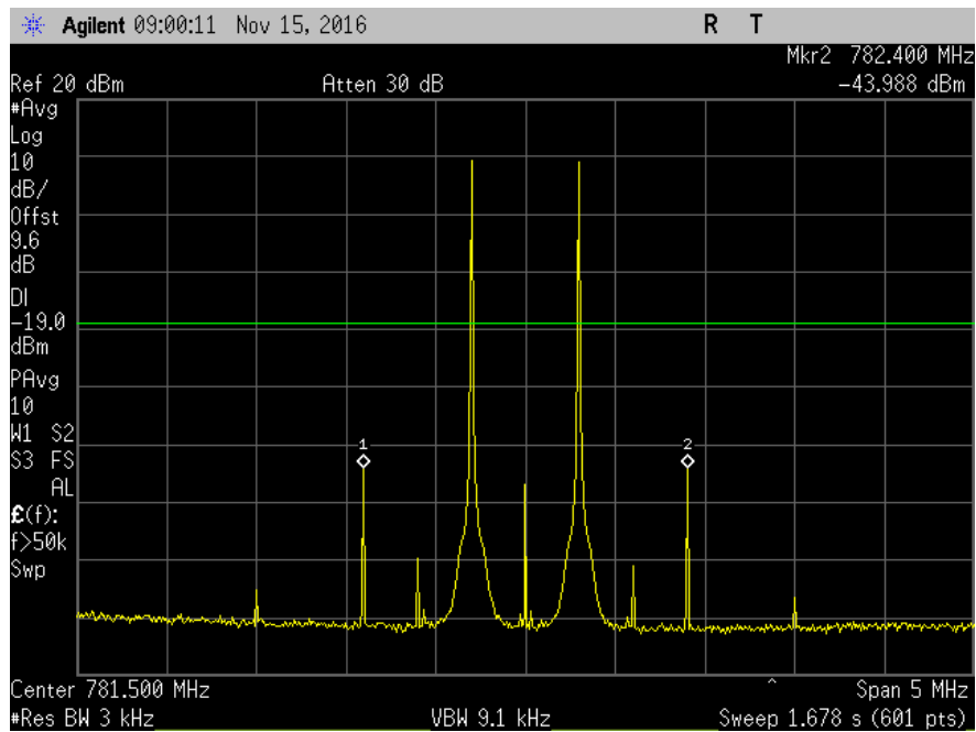
7.4_Intermod_UL_776-787MHz
