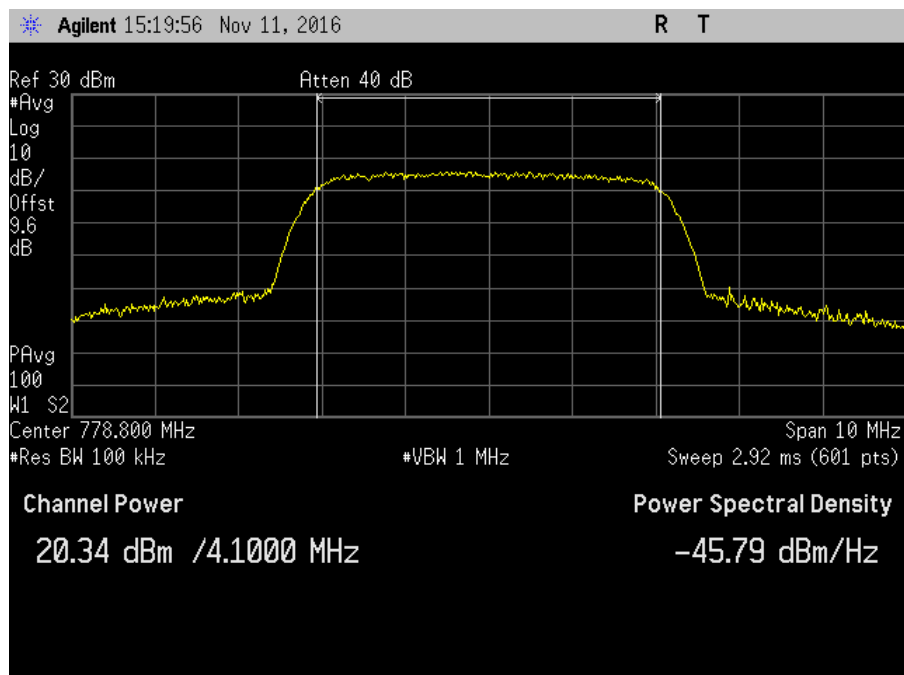
7.2_Power_UL_776-787MHz_AWGN_Max
