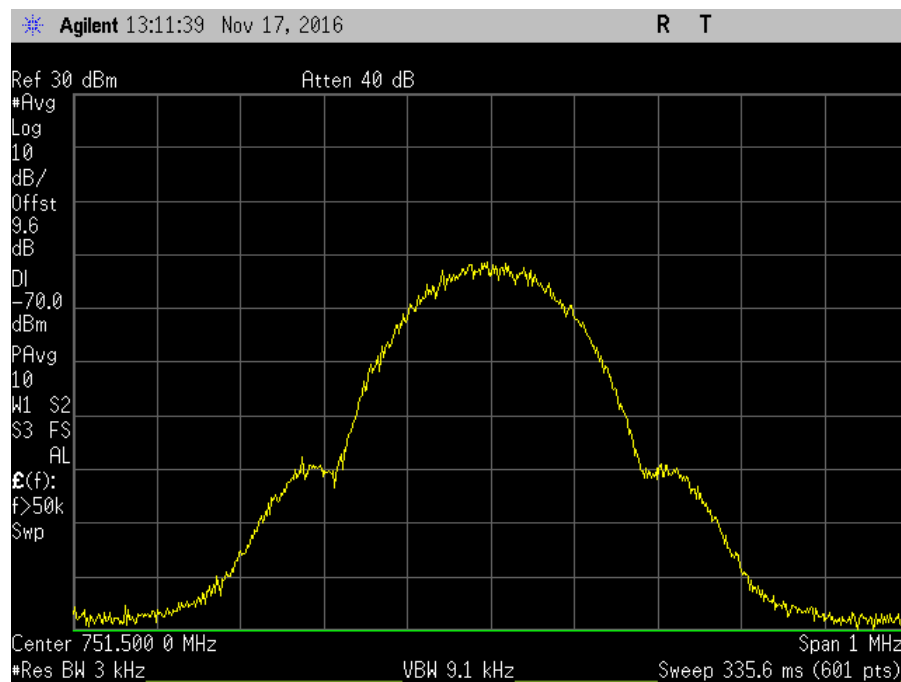
7.10_OBW_DL_746-757MHz_GSM_Out
