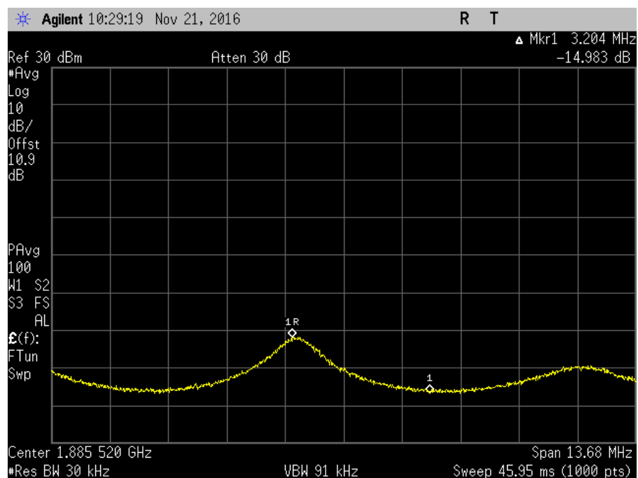
7.11.3_Osc_UL_1850-1915MHz+3_AWGNL
