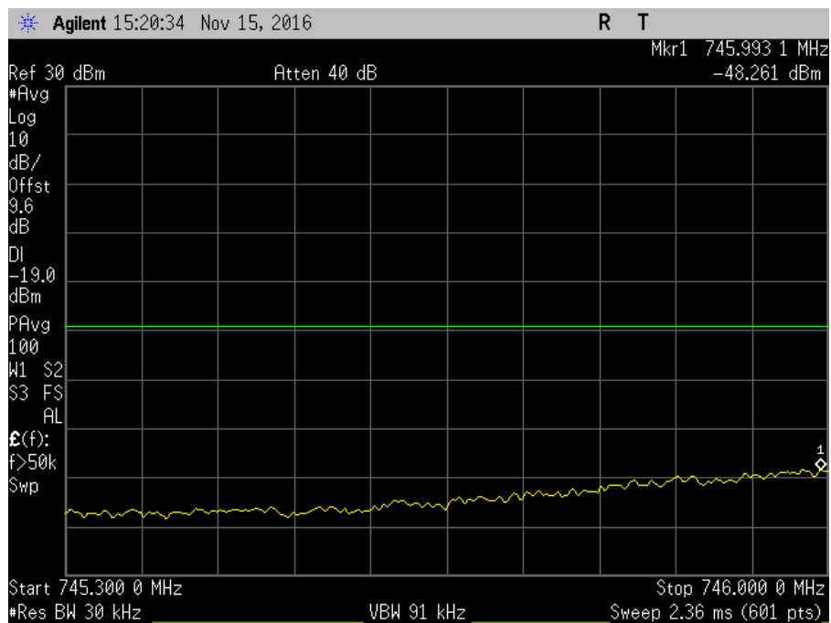
7.5_OBE_DL_746-757MHz_L_PreAGC_CDMA
