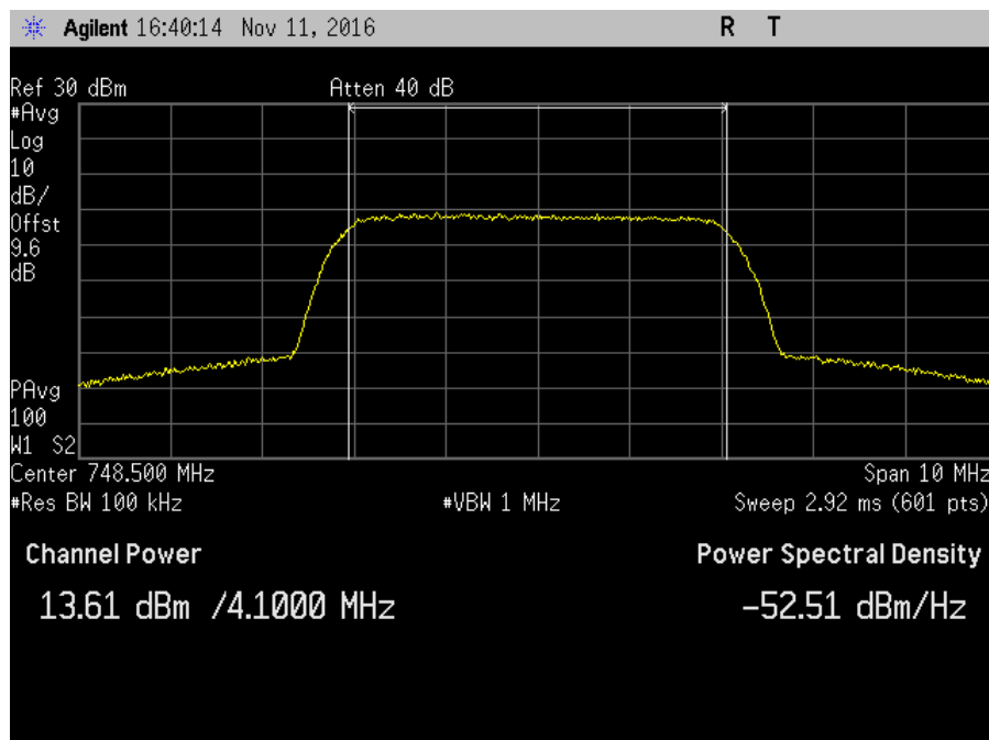
7.2_Power_DL_746-757MHz_AWGN_Max
