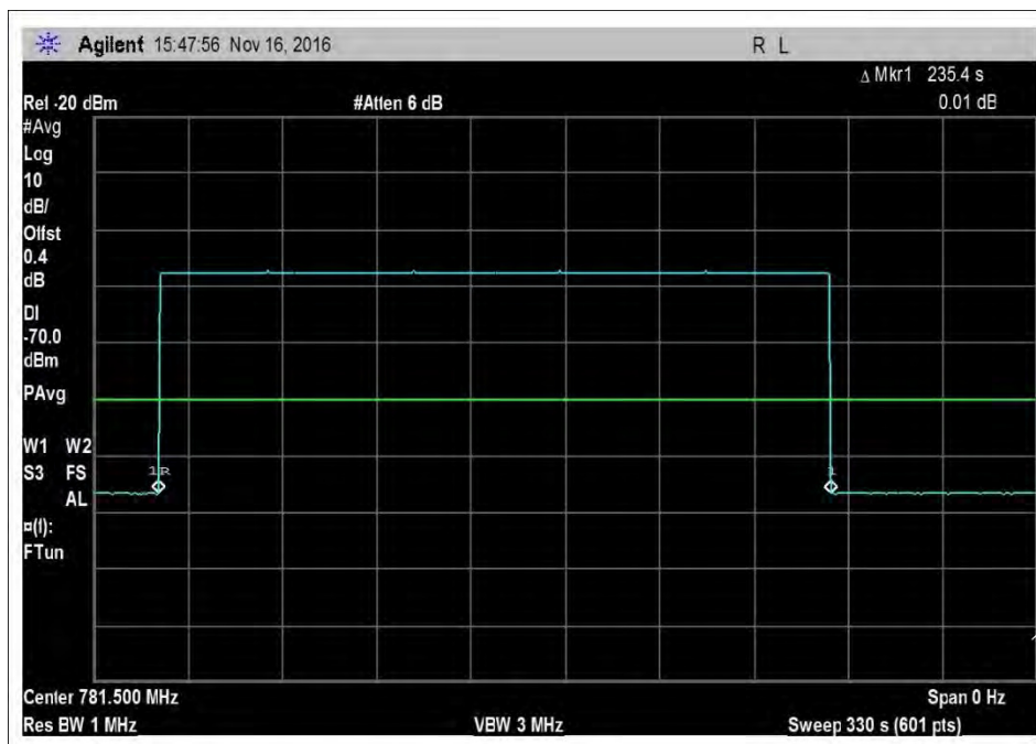
7.8_Inactivity_UL_776-787MHz
