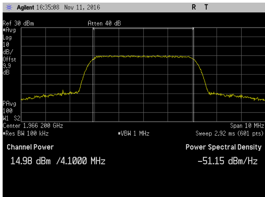
7.2_Power_DL_1930-1995MHz_AWGN_Max
