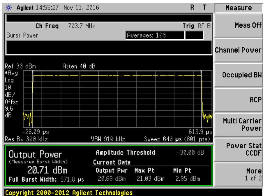
7.2_Power_UL_698-716MHz_GSM
