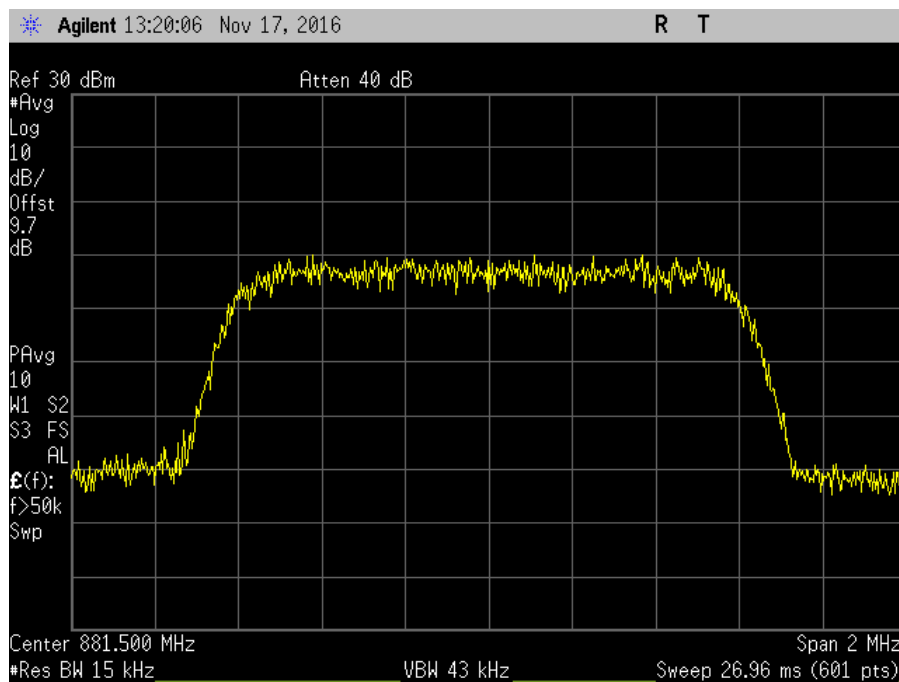
7.10_OBW_DL_869-894MHz_CDMA_Out
