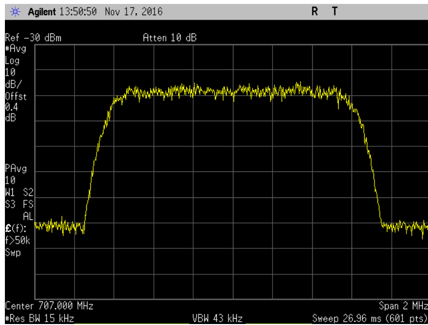
7.10_OBW_UL_698-716MHz_CDMA_In
