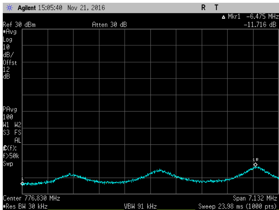
7.11.3_Osc_UL_776-787MHz+3_AWGNR
