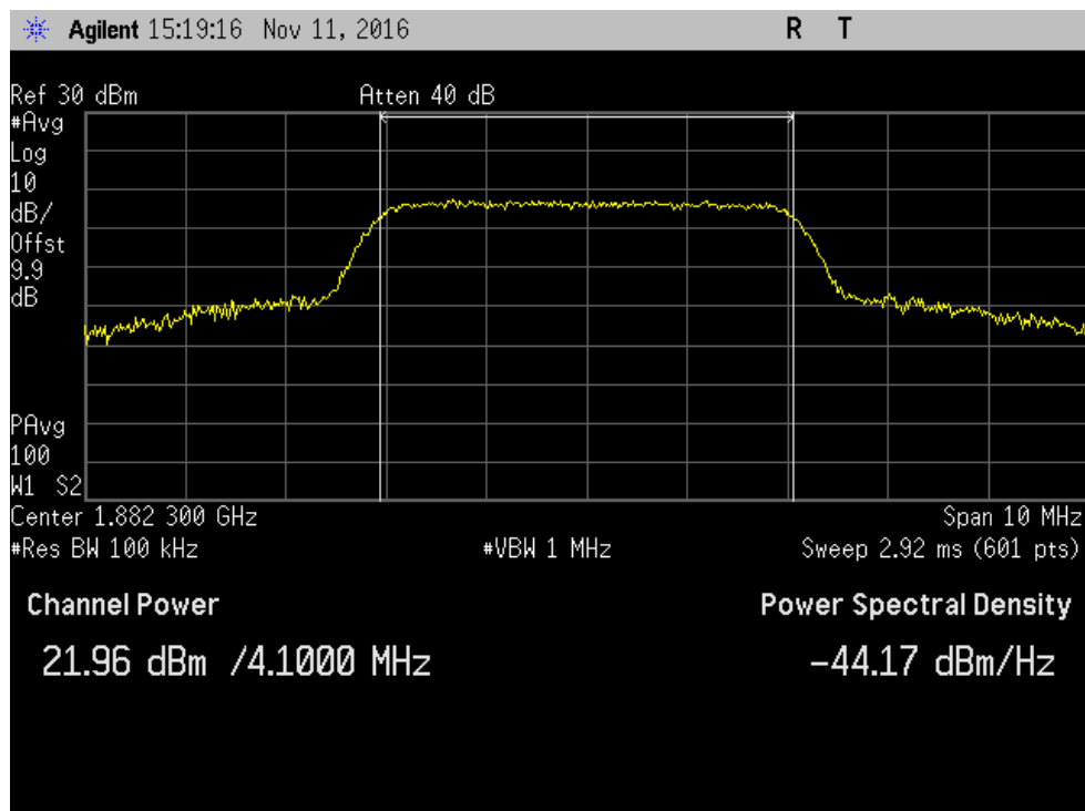
7.2_Power_UL_1850-1915MHz_AWGN_Max
