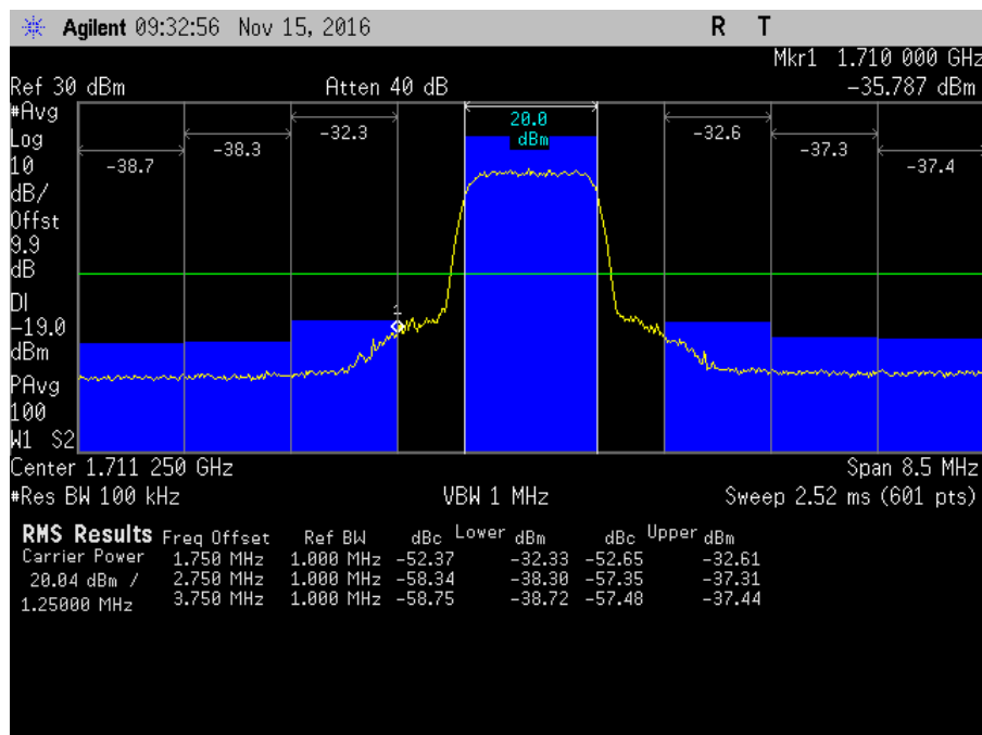
7.5_OBE_UL_1710-1755MHz_L_PreAGC_CDMA
