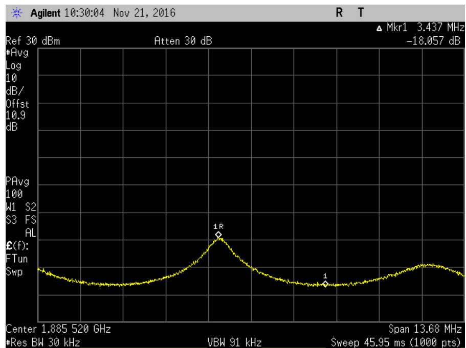
7.11.3_Osc_UL_1850-1915MHz+2_AWGNL
