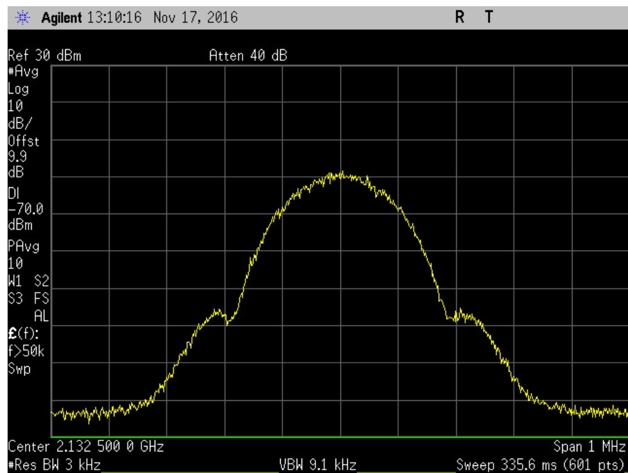
7.10_OBW_DL_2110-2155MHz_GSM_Out
