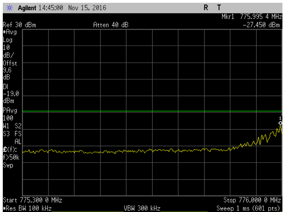
7.5_OBE_UL_776-787MHz_L_PreAGC_LTE
