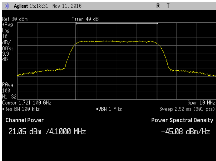
7.2_Power_UL_1710-1755MHz_AWGN_Max
