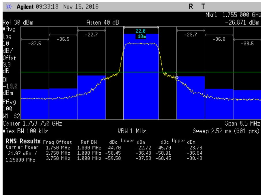
7.5_OBE_UL_1710-1755MHz_H_PreAGC_CDMA
