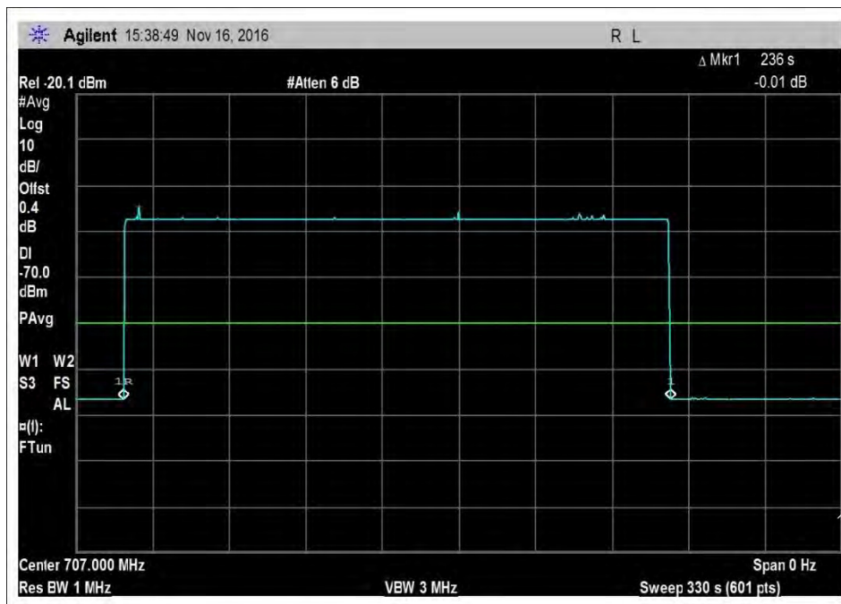
7.8_Inactivity_UL_698-707MHz
