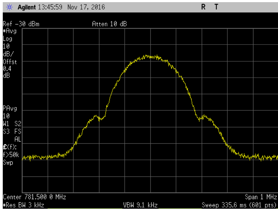
7.10_OBW_UL_776-787MHz_GSM_In
