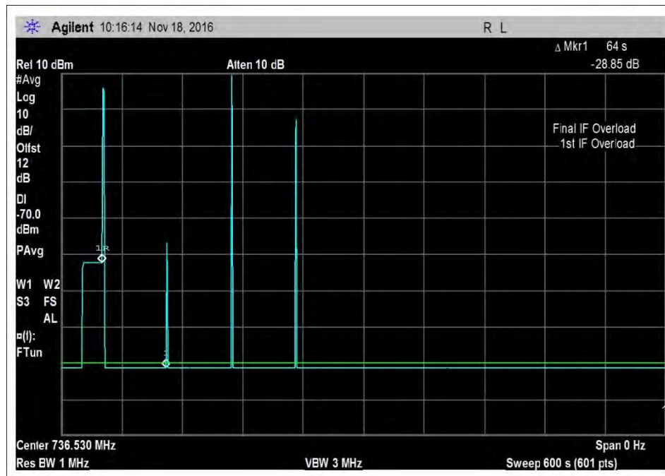
7.11_osc_DL-728-746MHz-600sec
