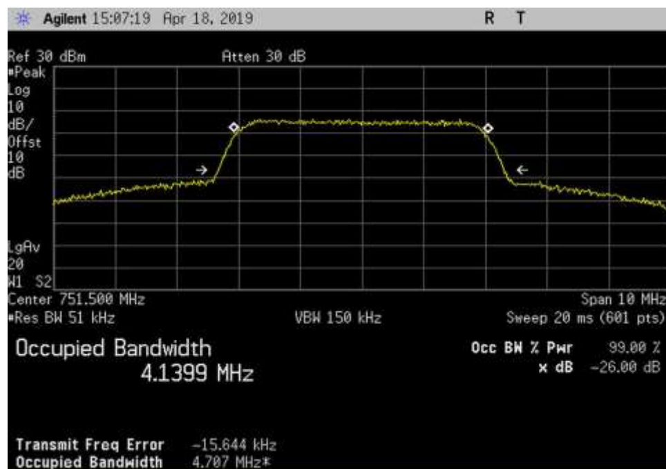
Out_DL_746-757_AWGN_751.5MHz
