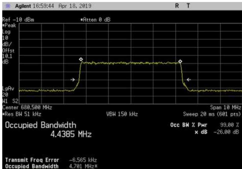
In_UL_663-698_LTE_680.5MHz
