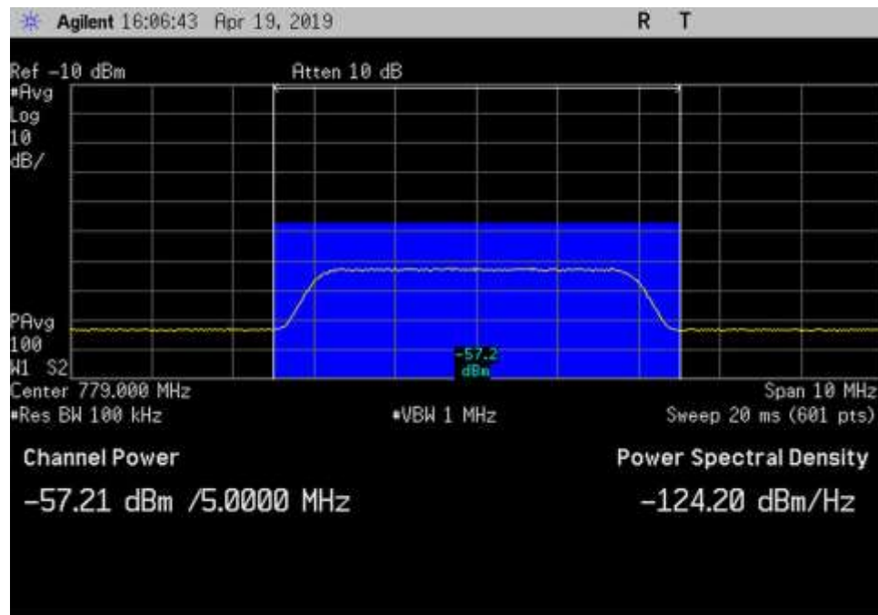
UL_776-787_AWGN_779MHz_Input
