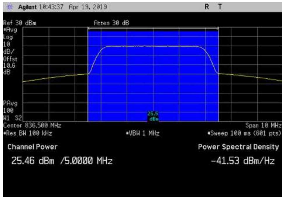
UL_824-849_AWGN_836.5MHz
