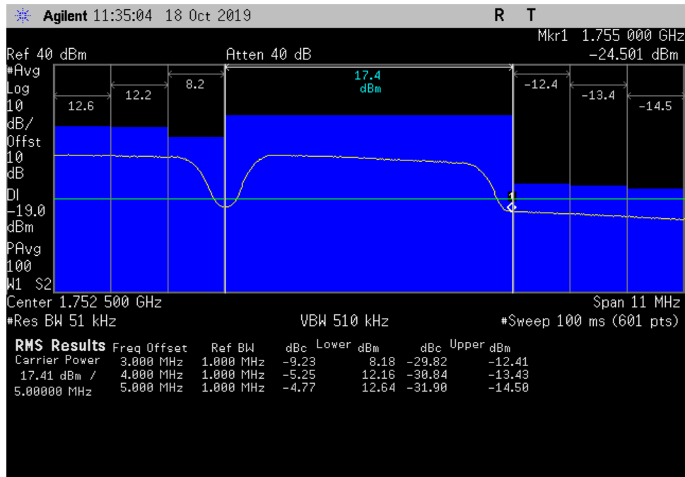
UL_1710-1755_AWGN_ 1747- 1758MHz_Cm_H
