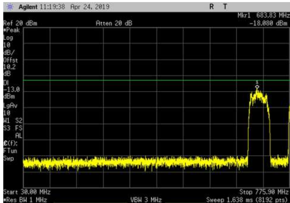
UL_776-787_GSM_30-775.9MHz_HC
