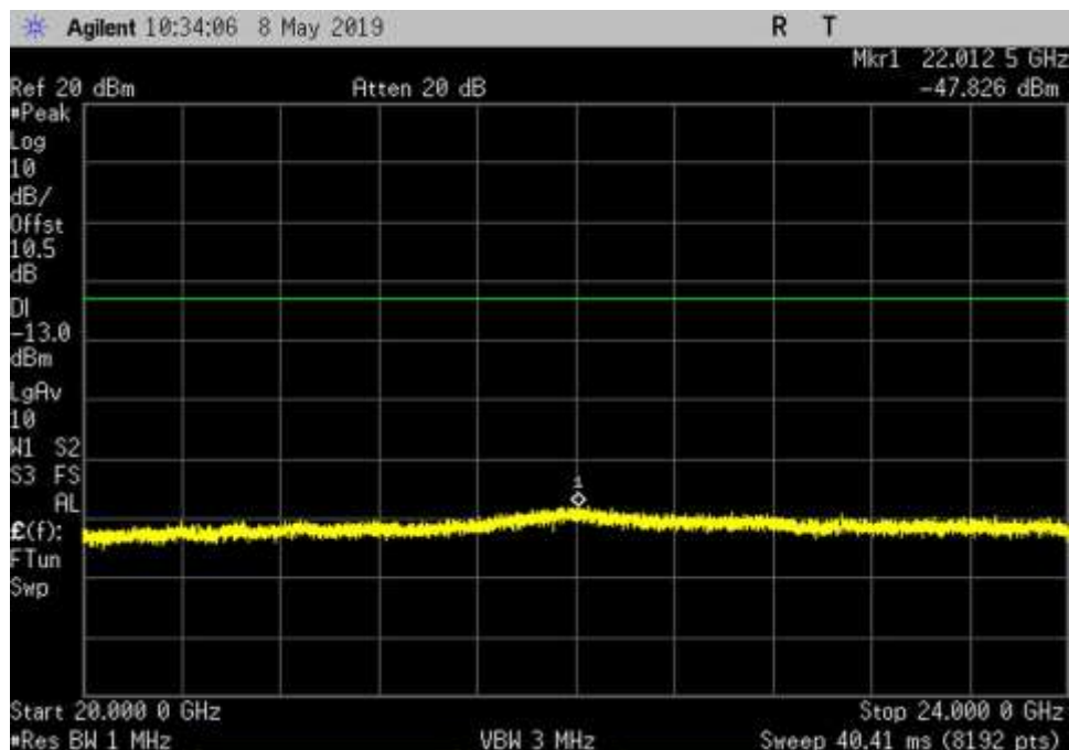
DL_2350-2360_AWGN_20000-24000MHz_MC
