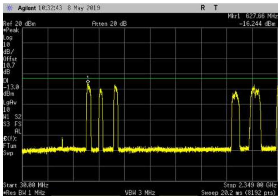
DL_2350-2360_AWGN_30- 2349MHz_MC
