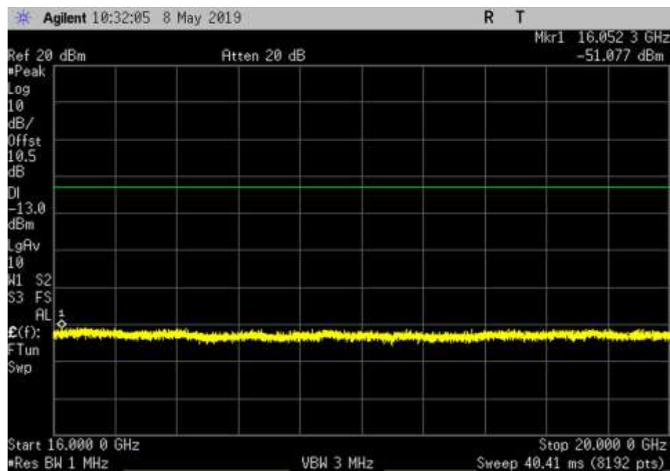
DL_2350-2360_AWGN_16000- 20000MHz_LC
