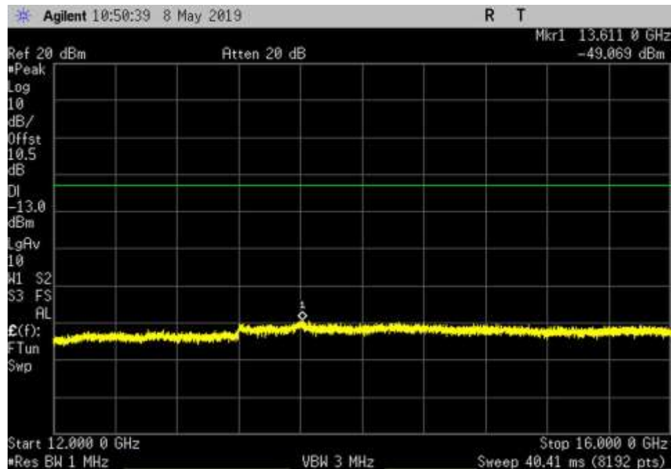
UL_2305-2315_GSM_12000- 16000MHz_LC
