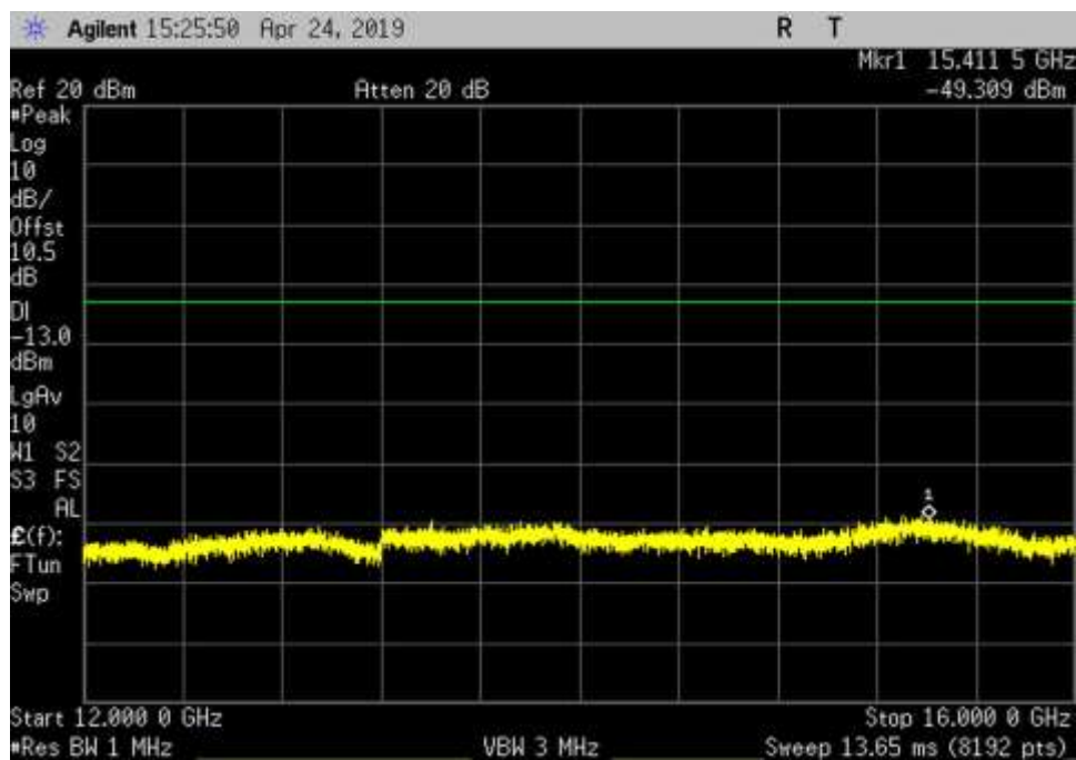
DL_2110-2155_AWGN_ 12000- 16000MHz_LC
