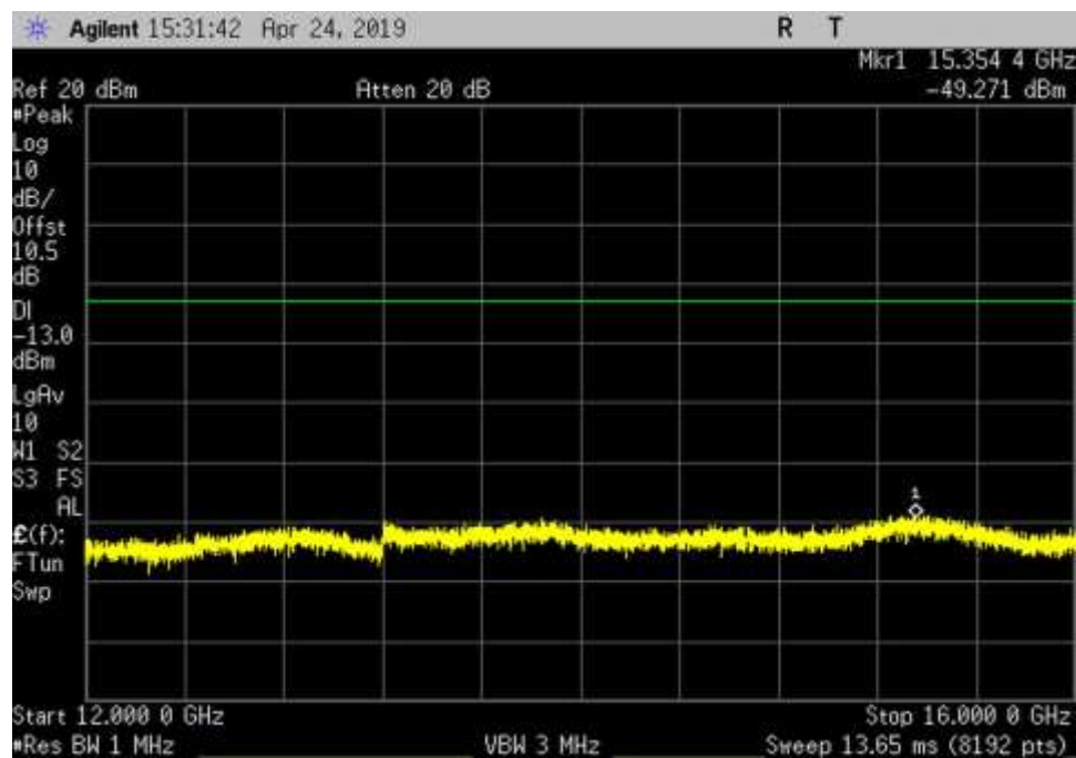
DL_1930-1995_AWGN_12000- 16000MHz_LC
