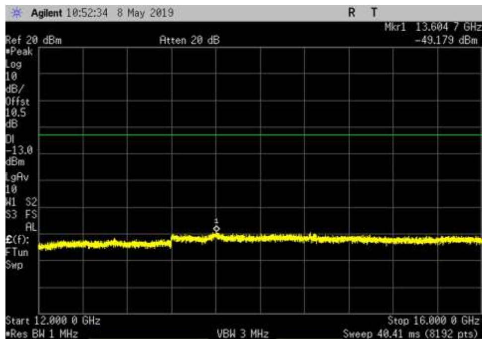
UL_2305-2315_GSM_12000- 16000MHz_MC
