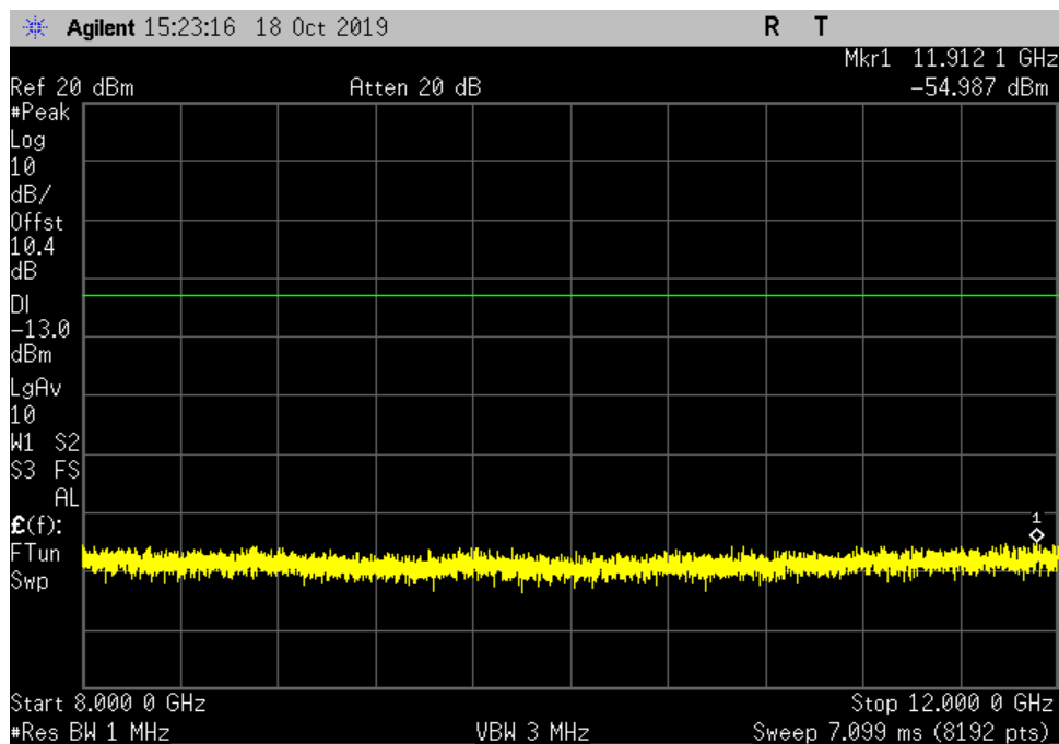
UL_1710-1755_GSM_8000-12000MHz_HC
