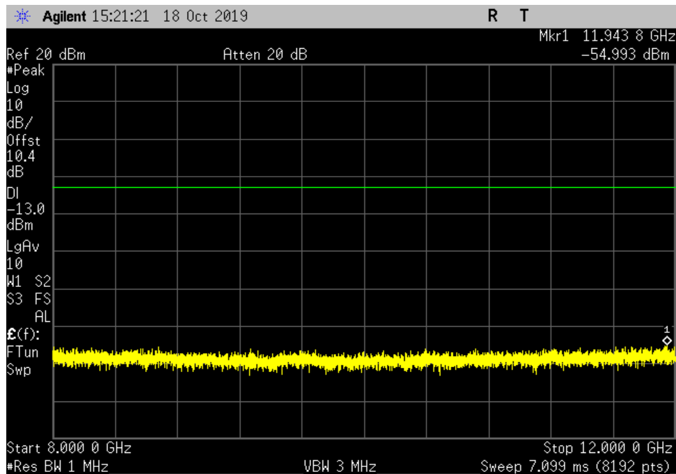
UL_1710-1755_GSM_8000-12000MHz_MC
