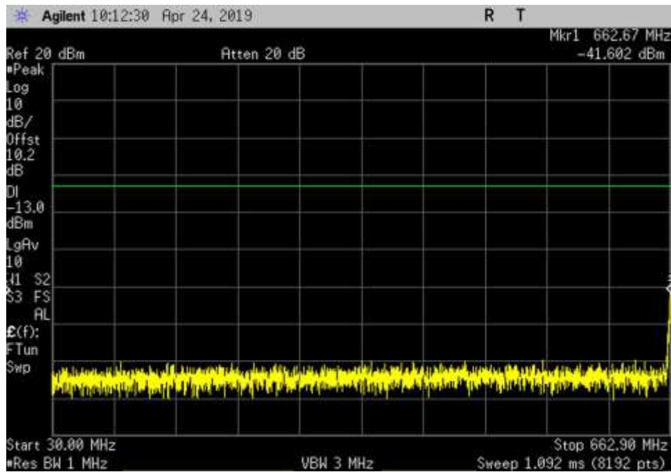
UL_663-698_GSM_30- 662.9MHz_MC
