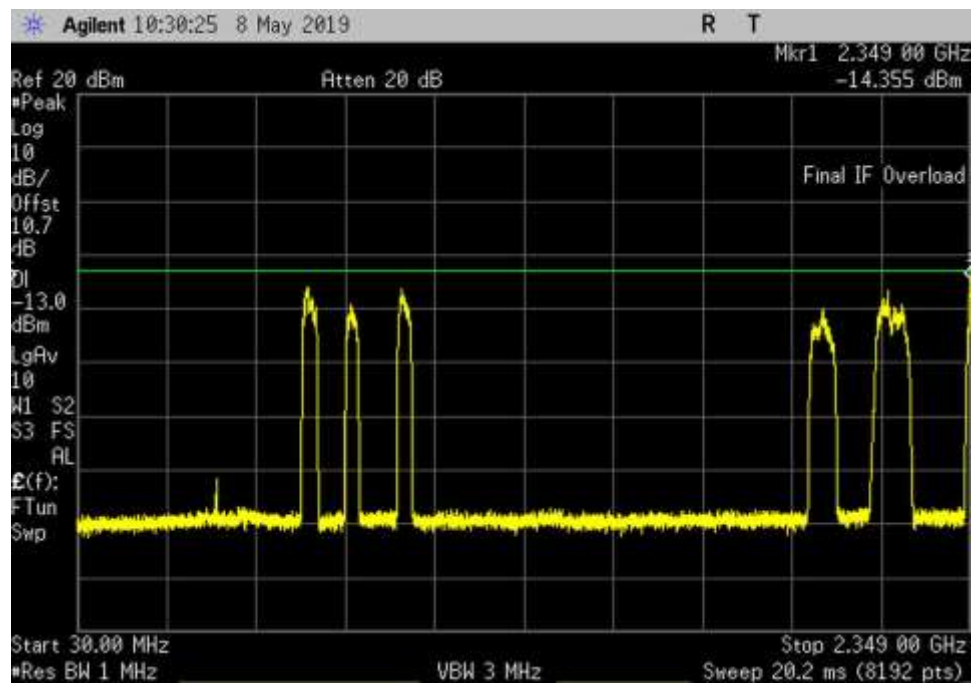
DL_2350-2360_AWGN_30- 2349MHz_LC
