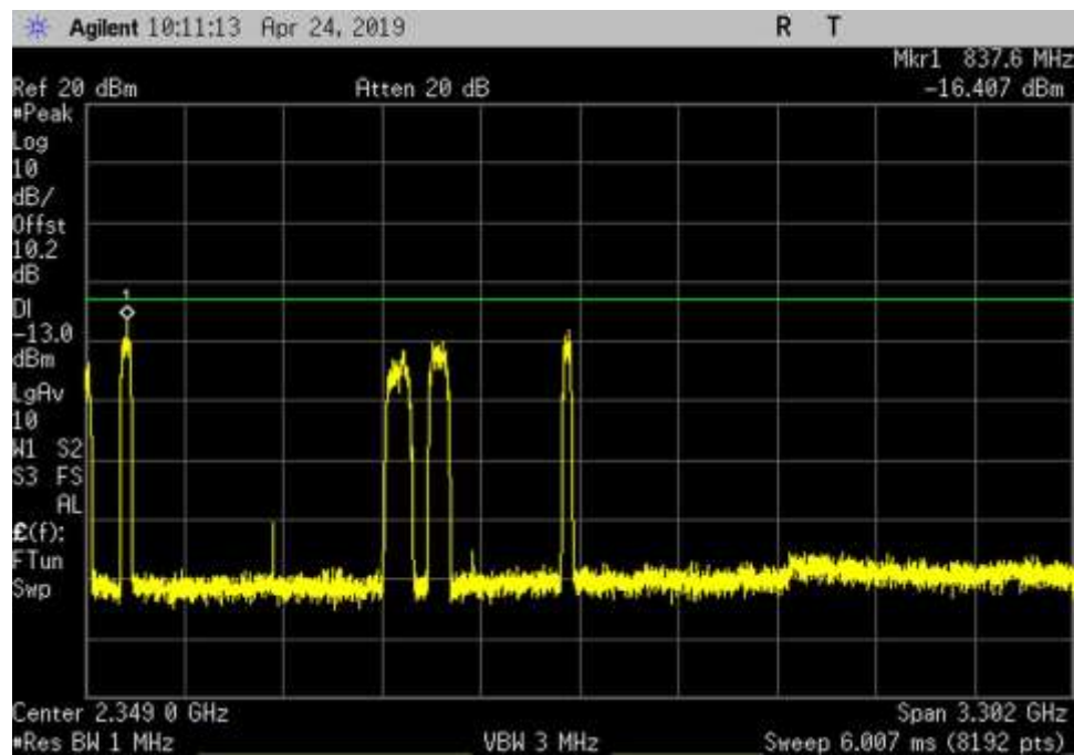
UL_663-698_GSM_698.1- 4000MHz_LC
