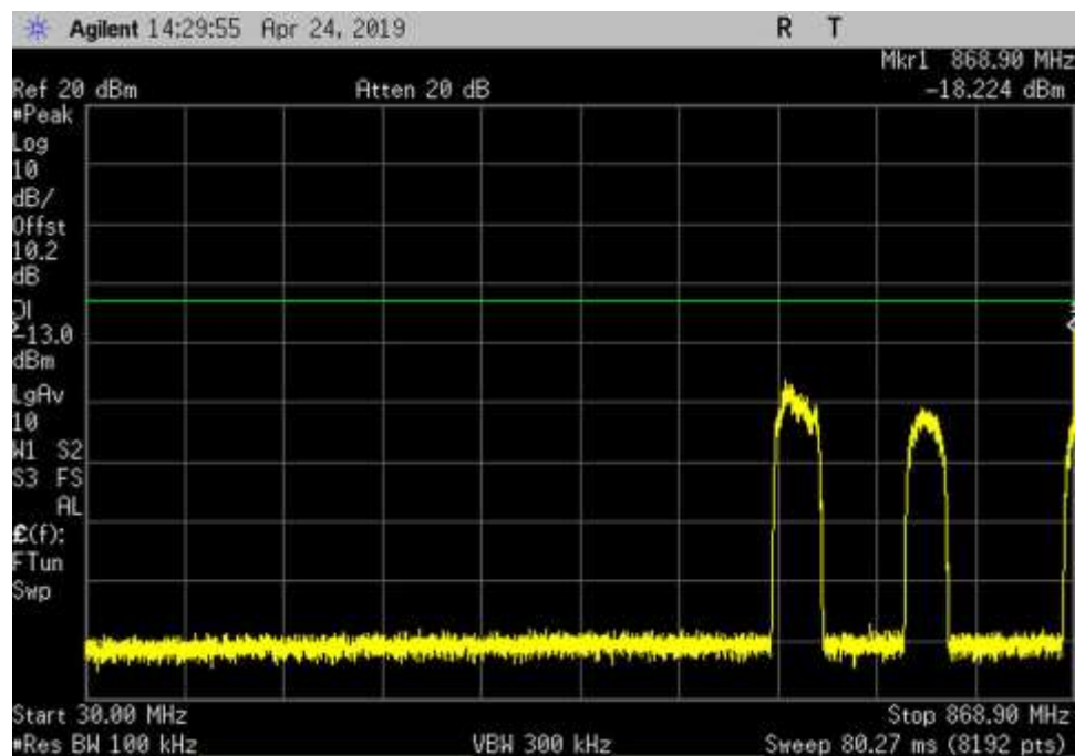
DL_869-894_GSM_30- 868.9MHz_LC
