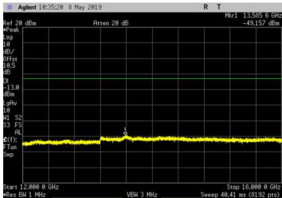
DL_2350-2360_AWGN_12000- 16000MHz_HC
