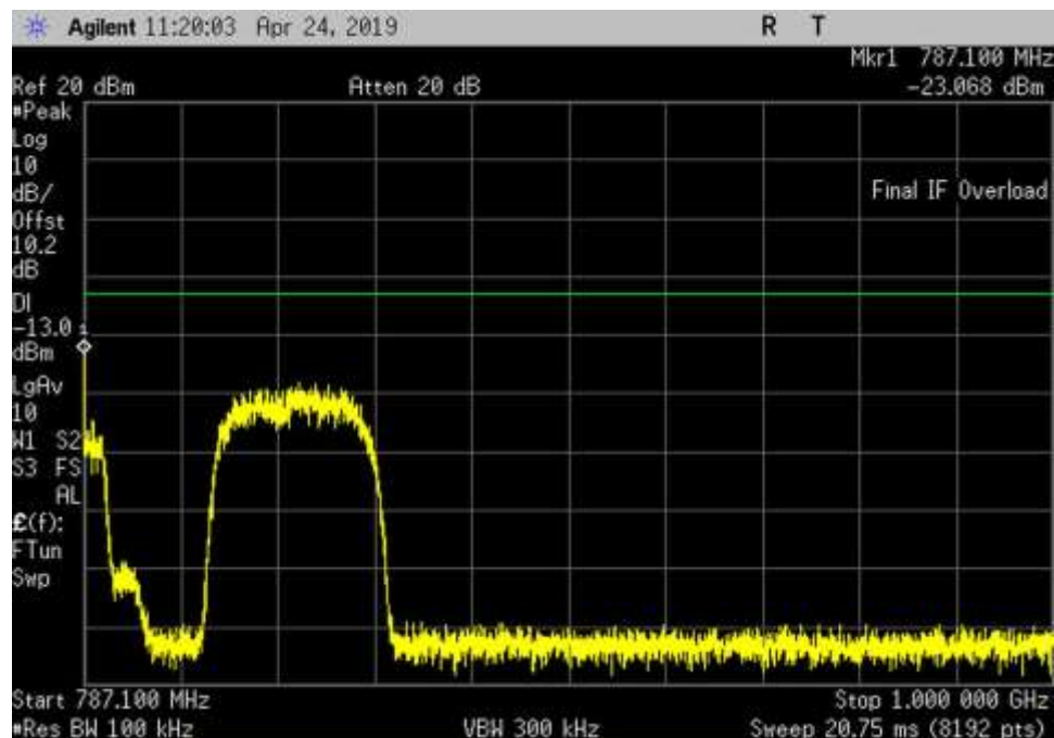
UL_776-787_GSM_787.1-1000MHz_HC
