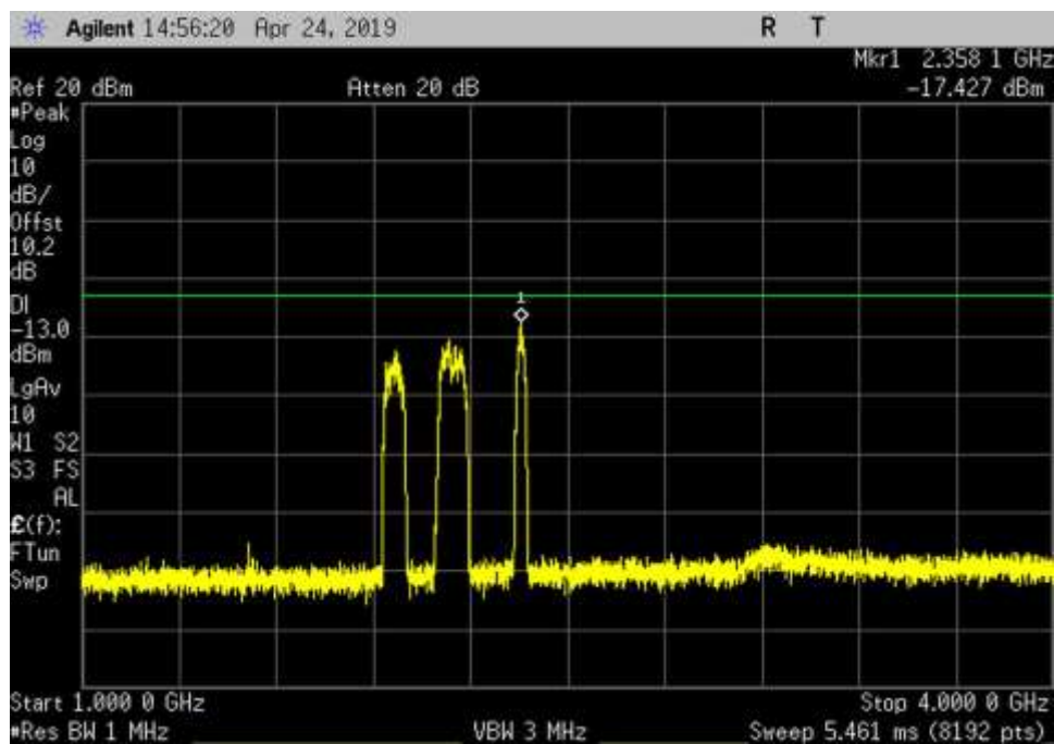
DL_746-757_GSM_1000-4000MHz_HC
