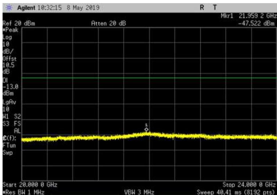
DL_2350-2360_AWGN_20000-24000MHz_LC
