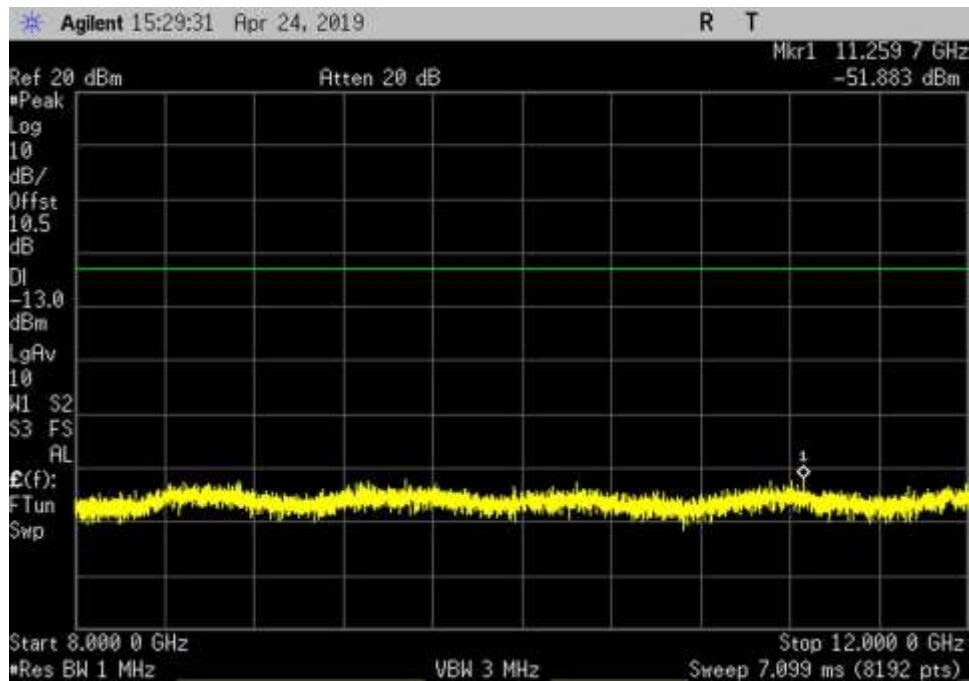
DL_2110-2155_AWGN_ 8000- 12000MHz_HC
