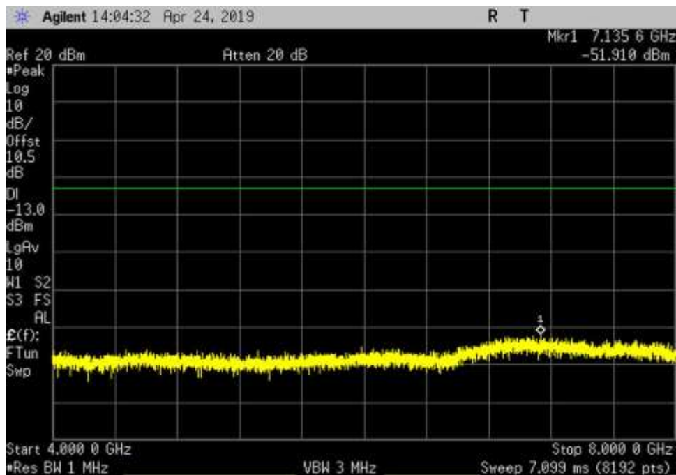
DL_2110-2155_GSM_4000-8000MHz_MC
