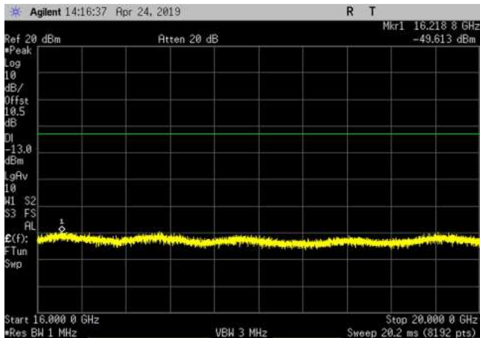
DL_2110-2155_GSM_16000-20000MHz_HC
