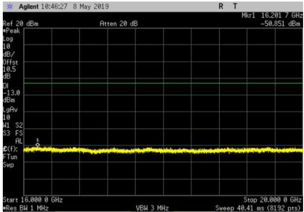
DL_2350-2360_GSM_16000- 20000MHz_HC
