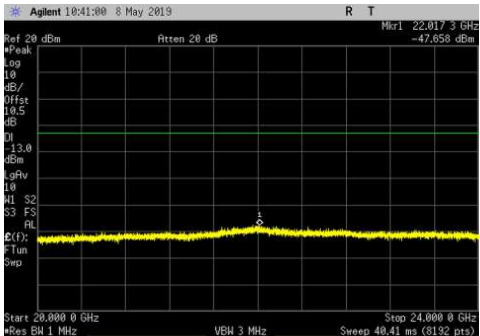
DL_2350-2360_GSM_20000- 24000MHz_LC
