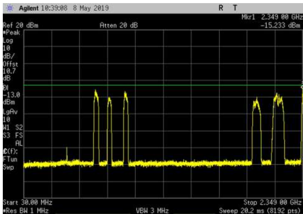
DL_2350-2360_GSM_30- 2349MHz_LC
