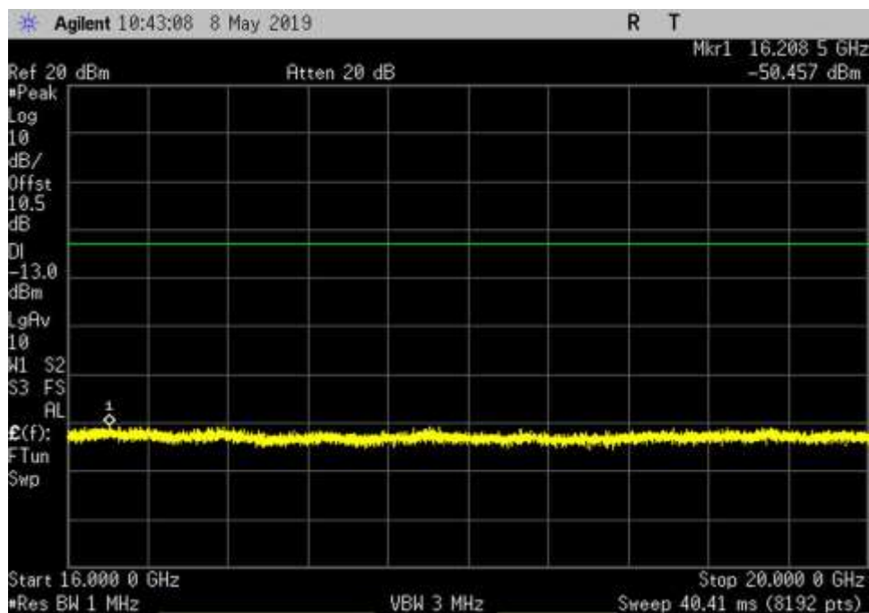
DL_2350-2360_GSM_16000- 20000MHz_MC
