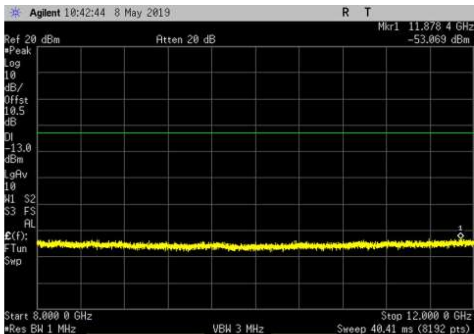
DL_2350-2360_GSM_8000- 12000MHz_MC
