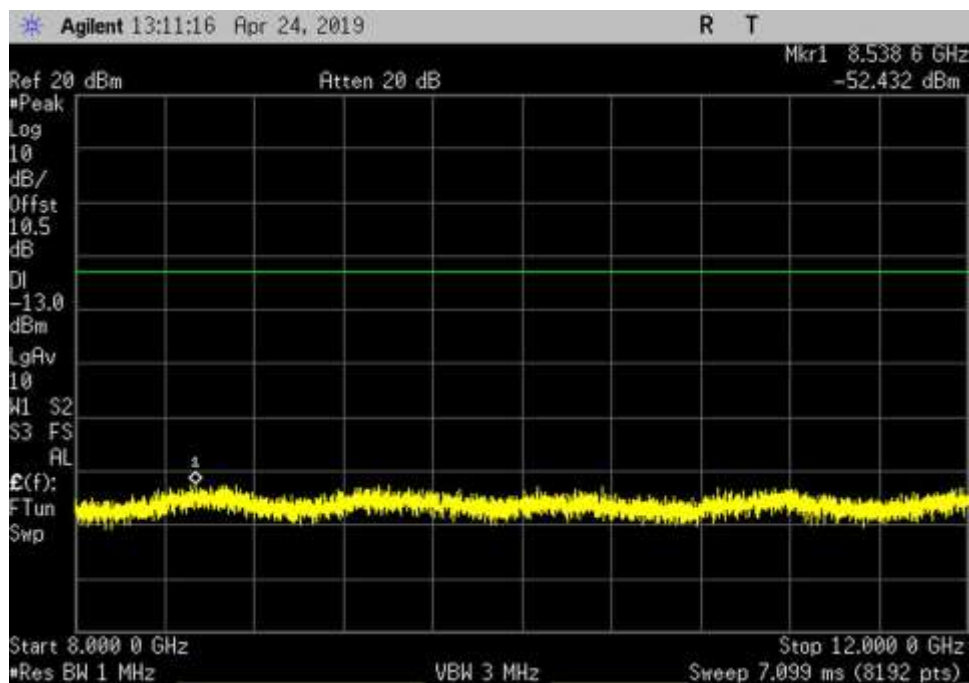
DL_2110-2155_GSM_8000- 12000MHz_LC
