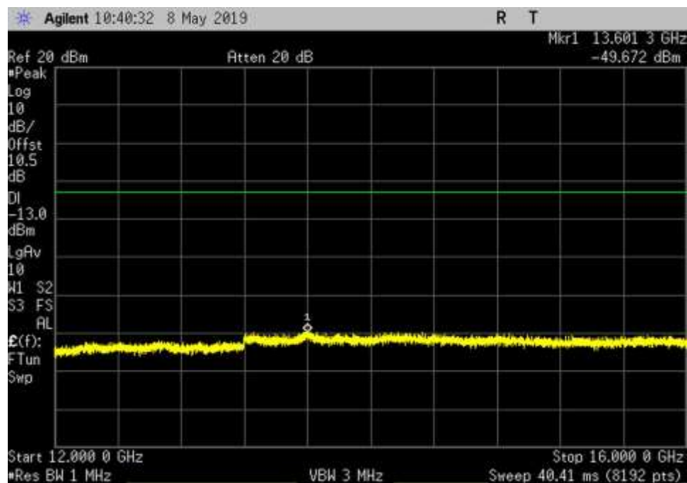
DL_2350-2360_GSM_12000- 16000MHz_LC
