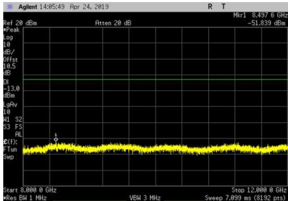
DL_2110-2155_GSM_8000-12000MHz_MC
