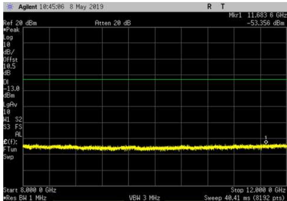
DL_2350-2360_GSM_8000- 12000MHz_HC
