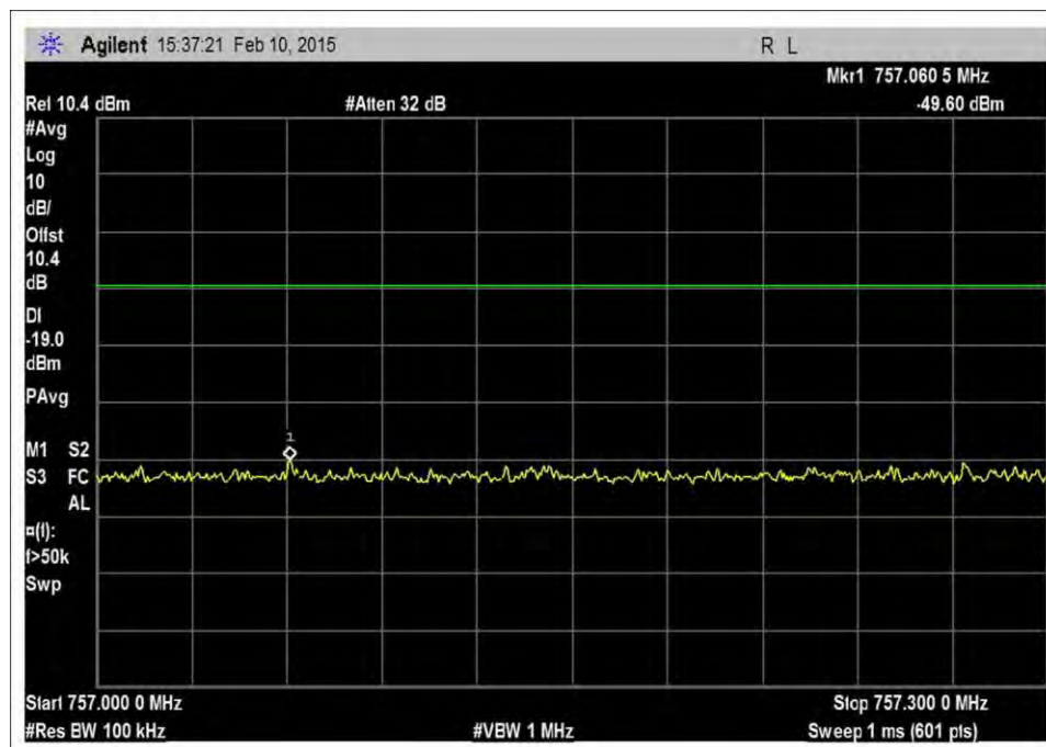
7.5_OBE_DL_746-757MHz_CDMA_H_-46dBm
