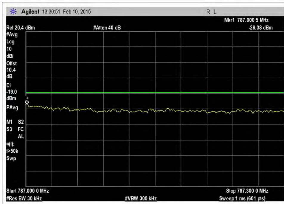
7.5_OBE_UL_776-787MHz_LTE_H_-26dBm
