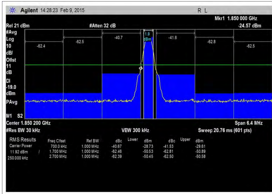
7.5_OBE_UL_1850-1915MHz_GSM_L_-27dBm
