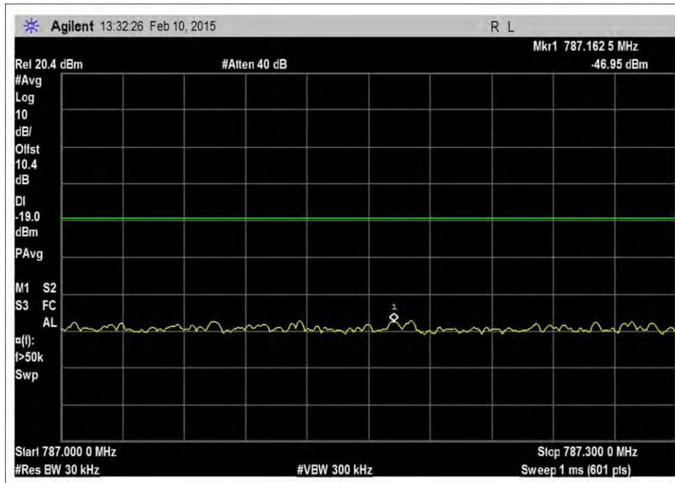
7.5_OBE_UL_776-787MHz_LTE_H_+10dBm
