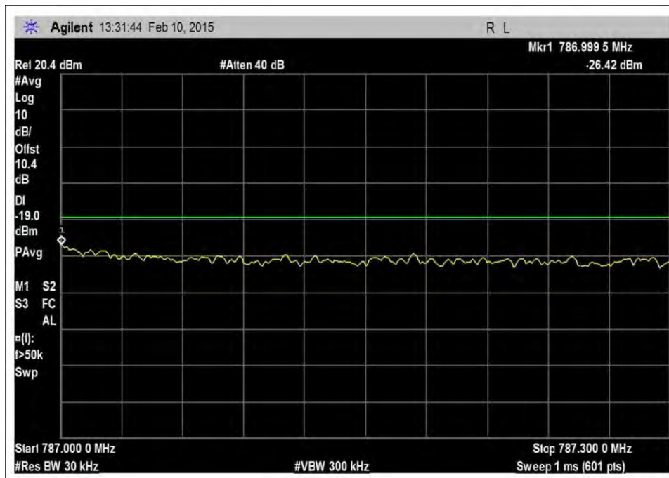
7.5_OBE_UL_776-787MHz_LTE_H_-22dBm
