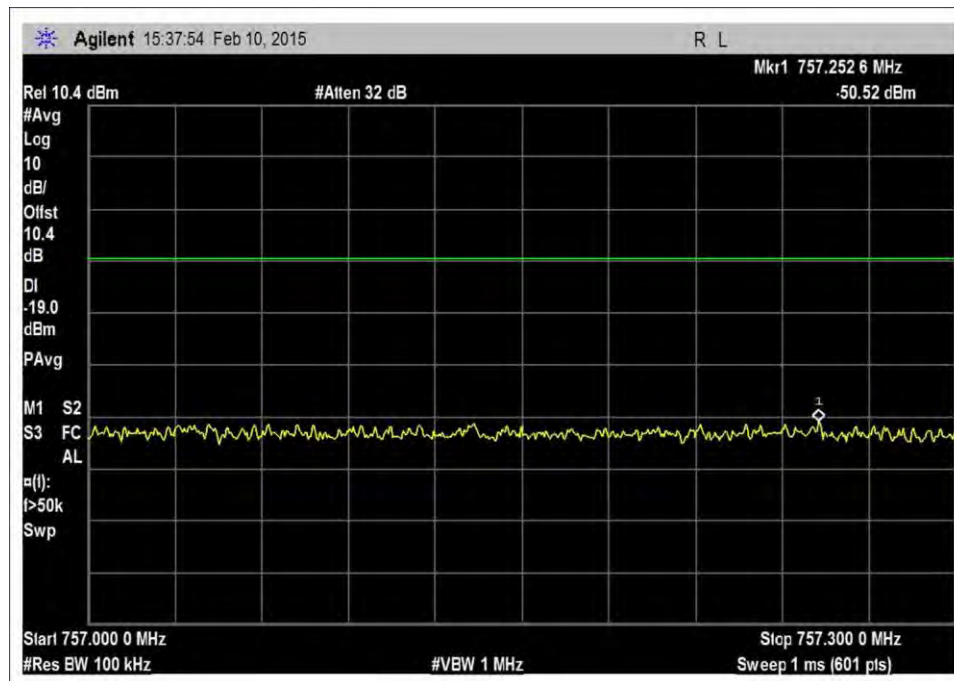
7.5_OBE_DL_746-757MHz_CDMA_H_-20dBm
