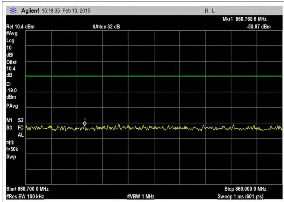
7.5_OBE_DL_869-880MHz_CDMA_L_-20dBm
