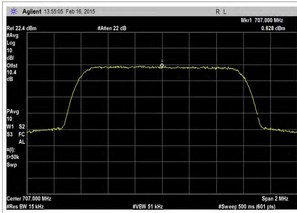
7.10_OBW_UL_698-716MHz_CDMA_Output
