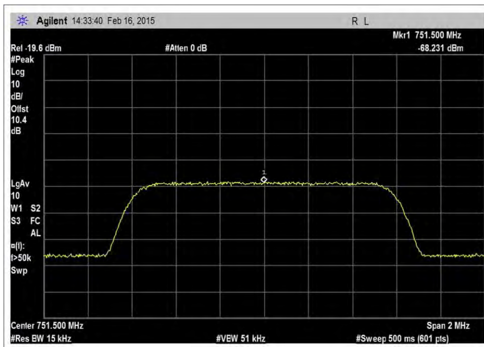
7.10_OBW_DL_746-757MHz_CDMA_Input
