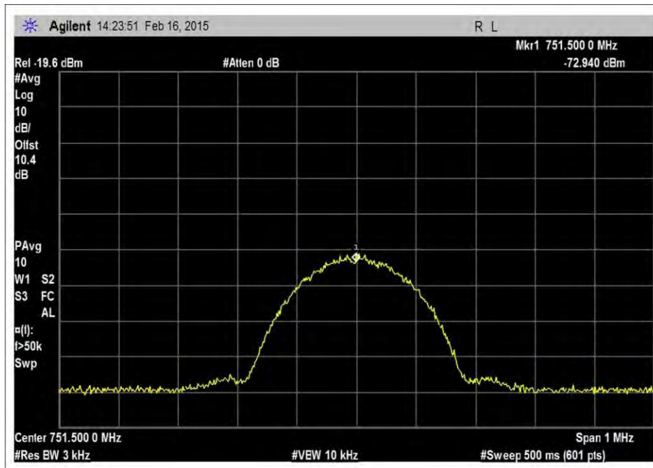
7.10_OBW_DL_746-757MHz_GSM__Input
