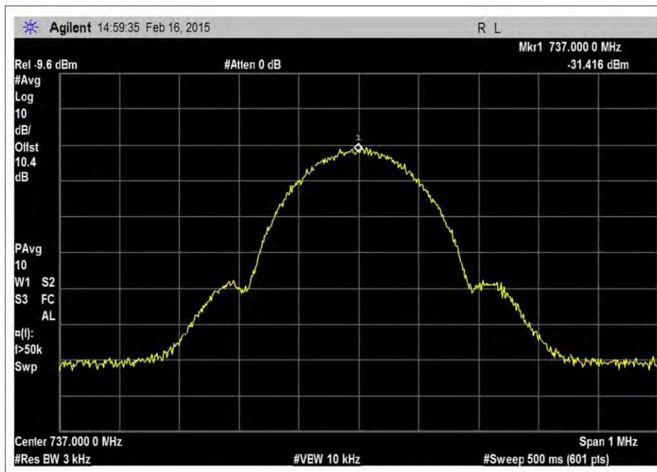
7.10_OBW_DL_728-746MHz_GSM_Output
