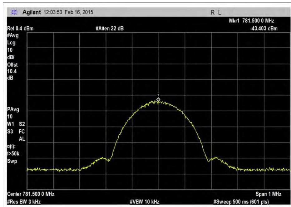
7.10_OBW_UL_776-787MHz_GSM__Input
