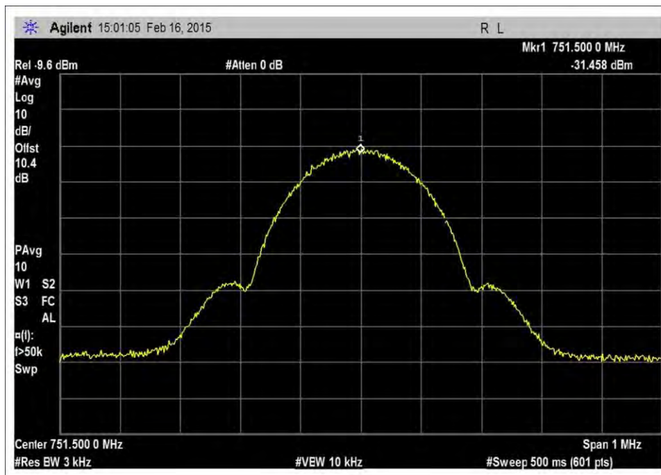
7.10_OBW_DL_746-757MHz_GSM_Output
