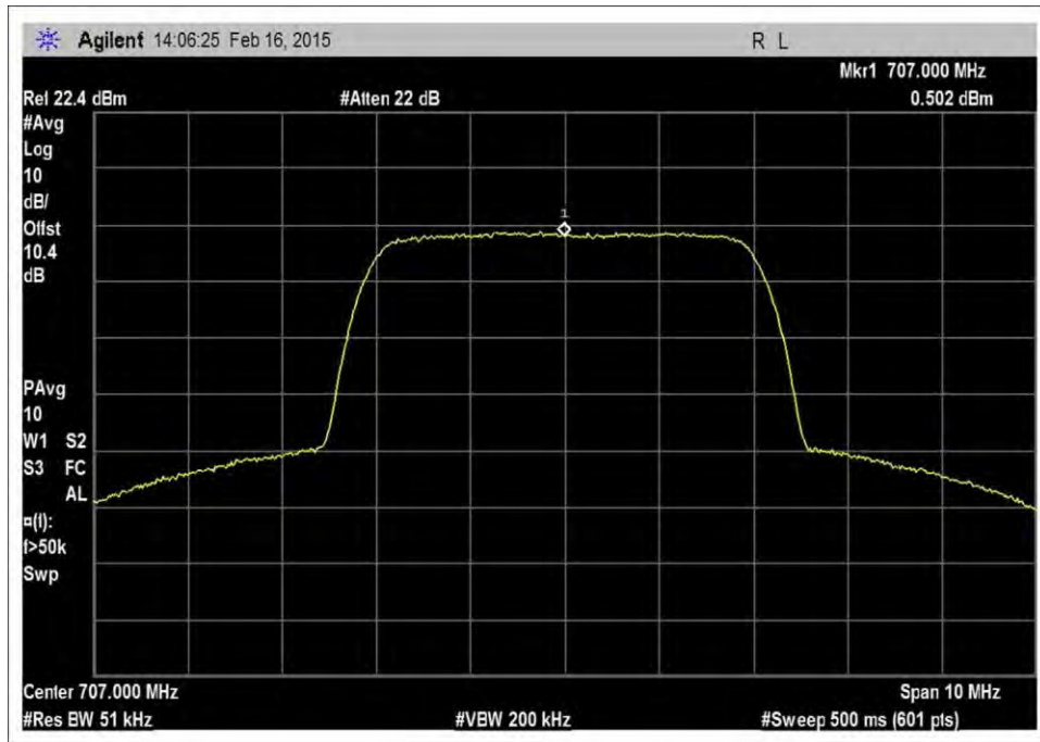
7.10_OBW_UL_698-716MHz_WCDMA_Output
