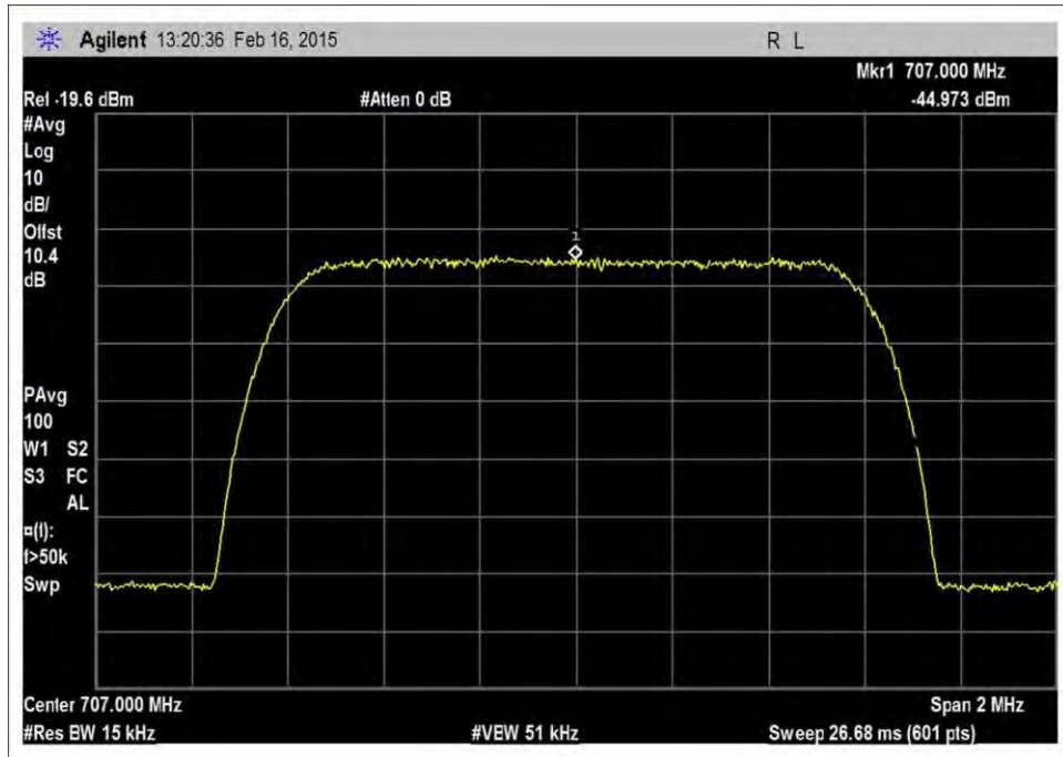
7.10_OBW_UL_698-716MHz_CDMA_Input
