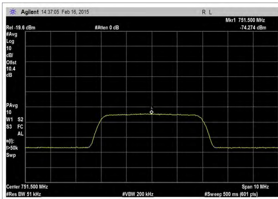
7.10_OBW_DL_746-757MHz_WCDMA_Input
