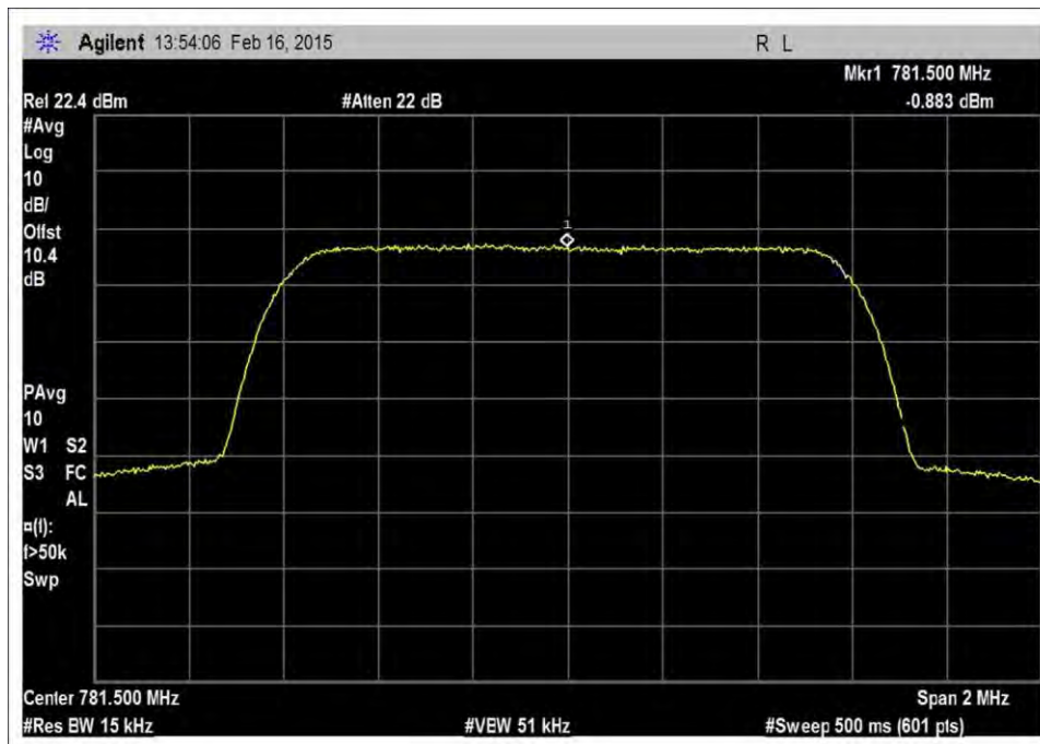
7.10_OBW_UL_776-787MHz_CDMA_Output
