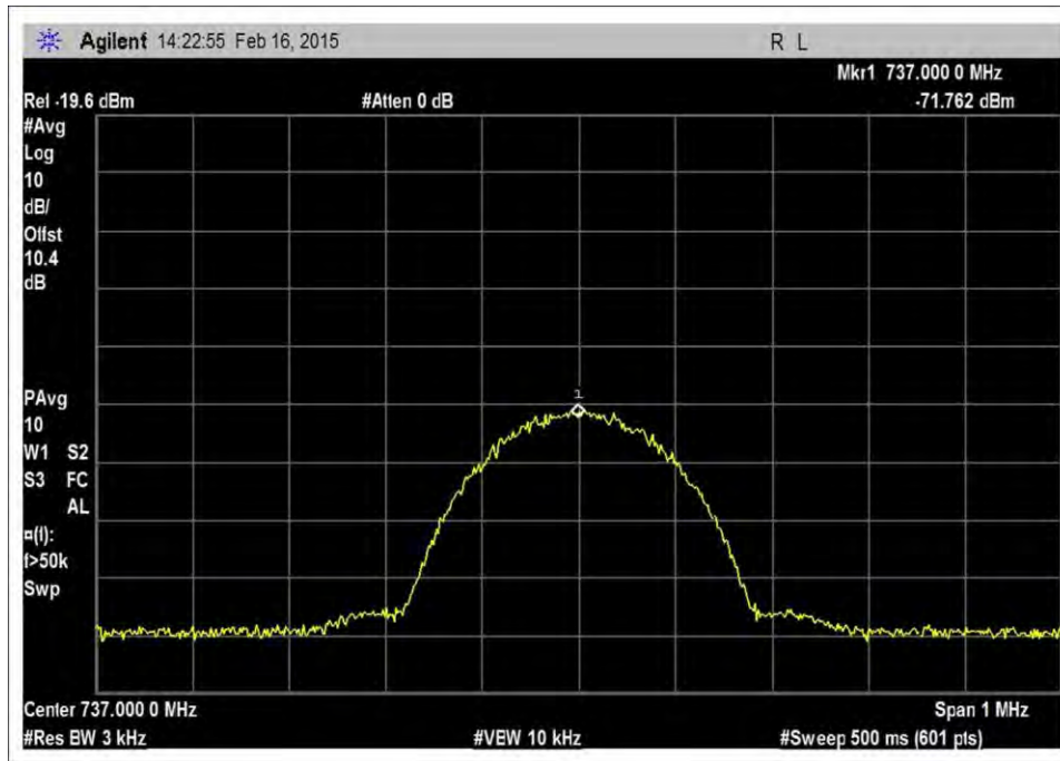
7.10_OBW_DL_728-746MHz_GSM__Input
