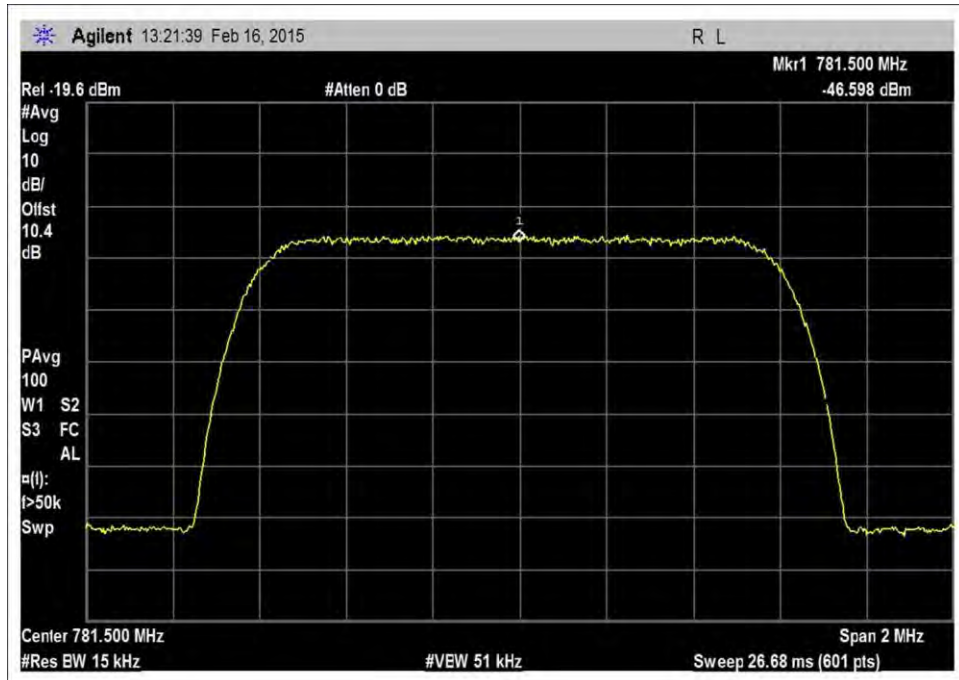
7.10_OBW_UL_776-787MHz_CDMA_Input
