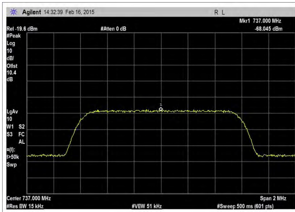
7.10_OBW_DL_728-746MHz_CDMA_Input
