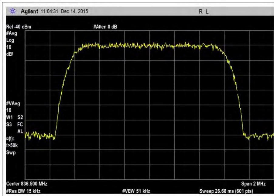
7.10_OBW_UL_824-849MHz_CDMA
