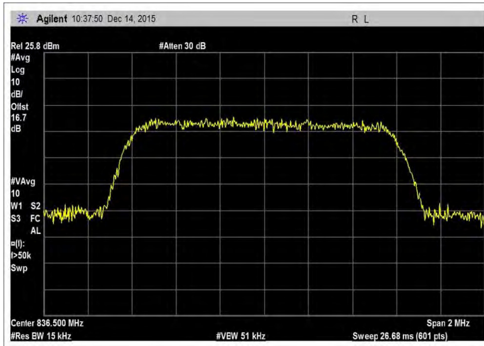
7.10_OBW_UL_824-849MHz_CDMA
